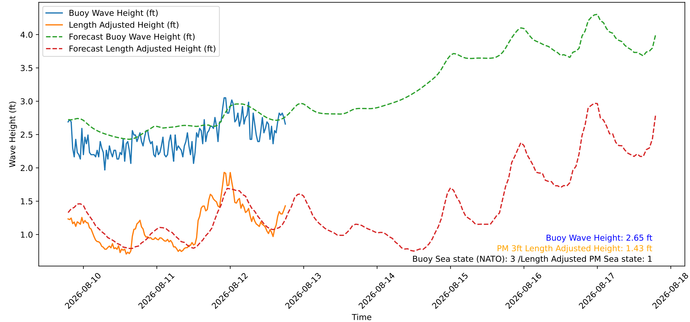
Wave Heights over Time for Oceanside Harbor at 2026-08-12 19:10:26
