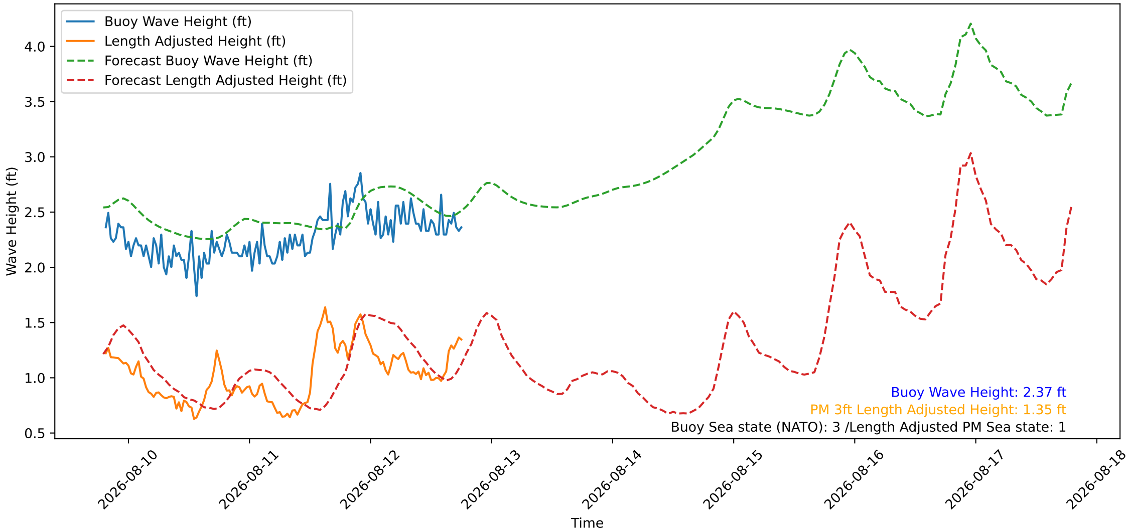
Wave Heights over Time for Red Beach at 2026-08-12 19:10:45
