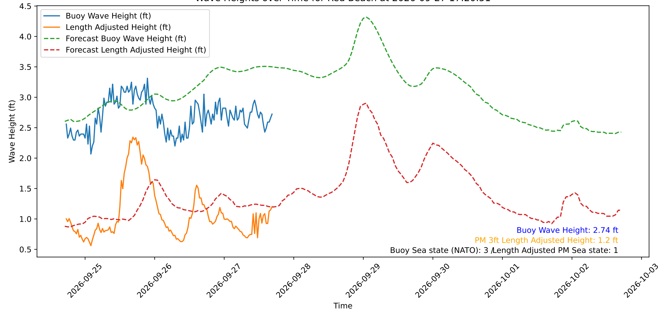
Wave Heights over Time for Red Beach at 2026-09-27 17:20:51
