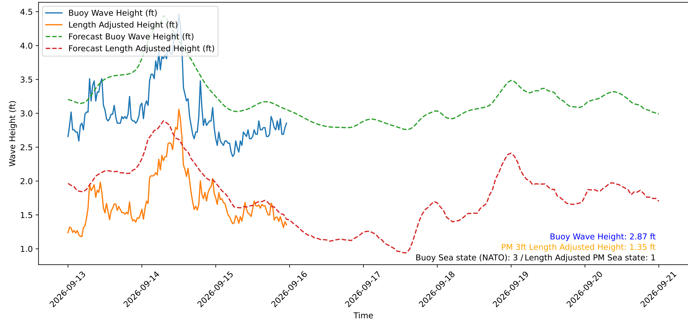
Wave Heights over Time for Oceanside Harbor at 2026-09-15 23:50:29
