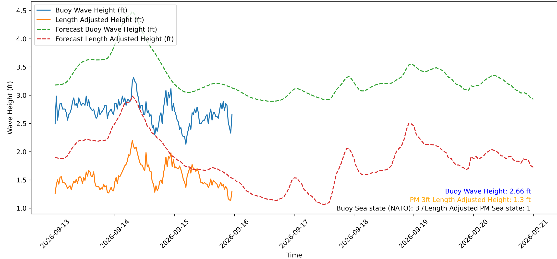
Wave Heights over Time for Green Beach at 2026-09-15 23:51:14
