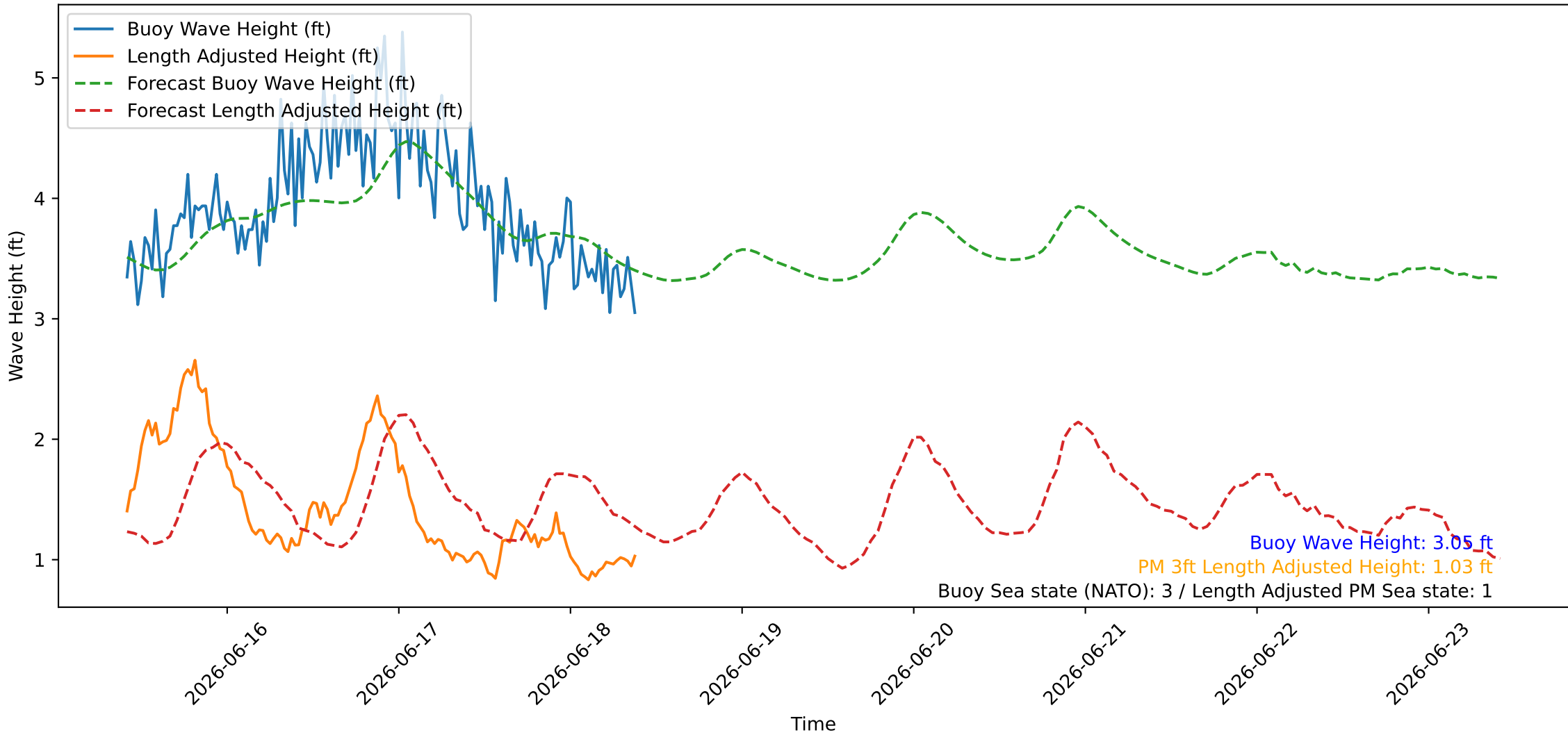
Wave Heights over Time for Red Beach at 2026-06-18 09:50:48
