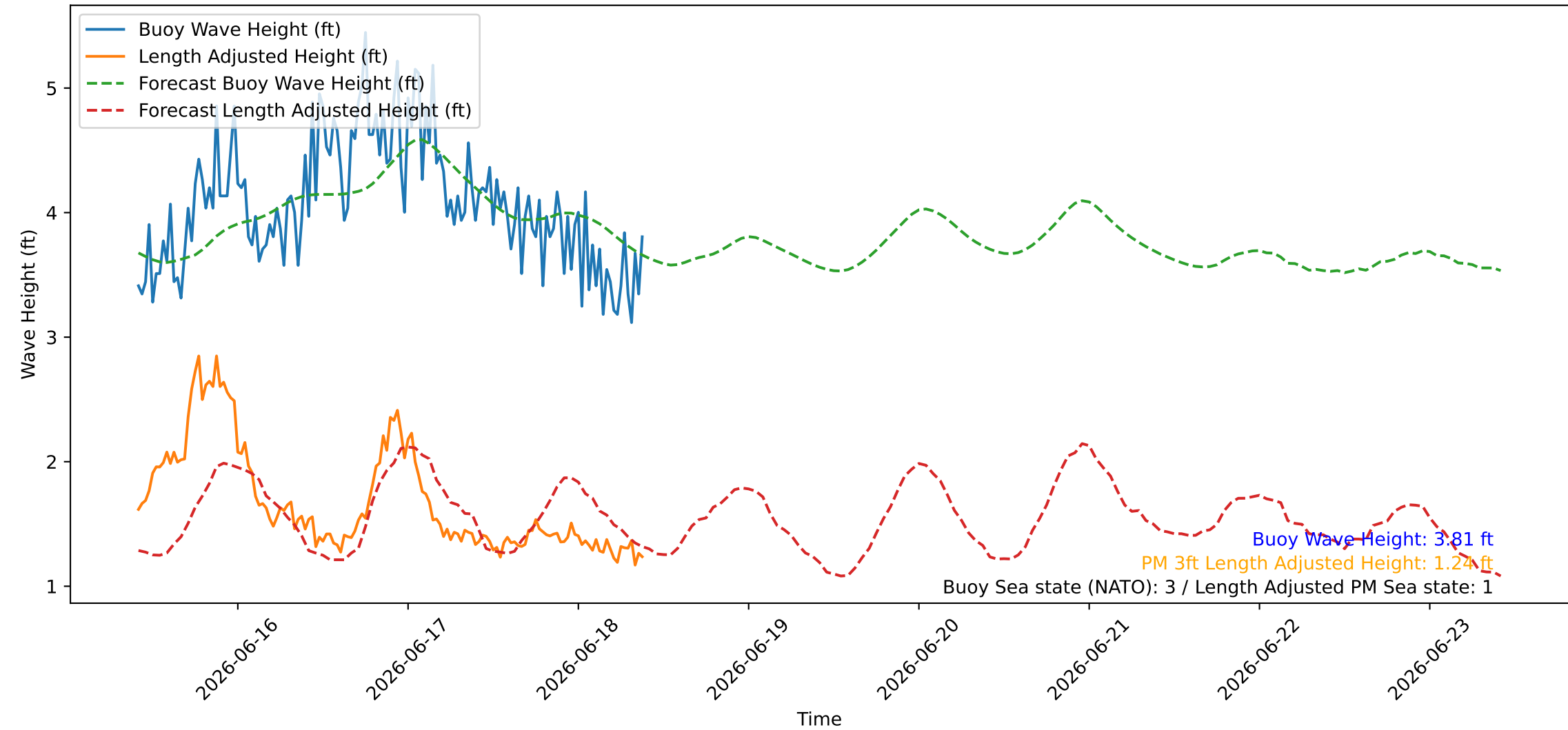
Wave Heights over Time for Oceanside Harbor at 2026-06-18 09:50:27
