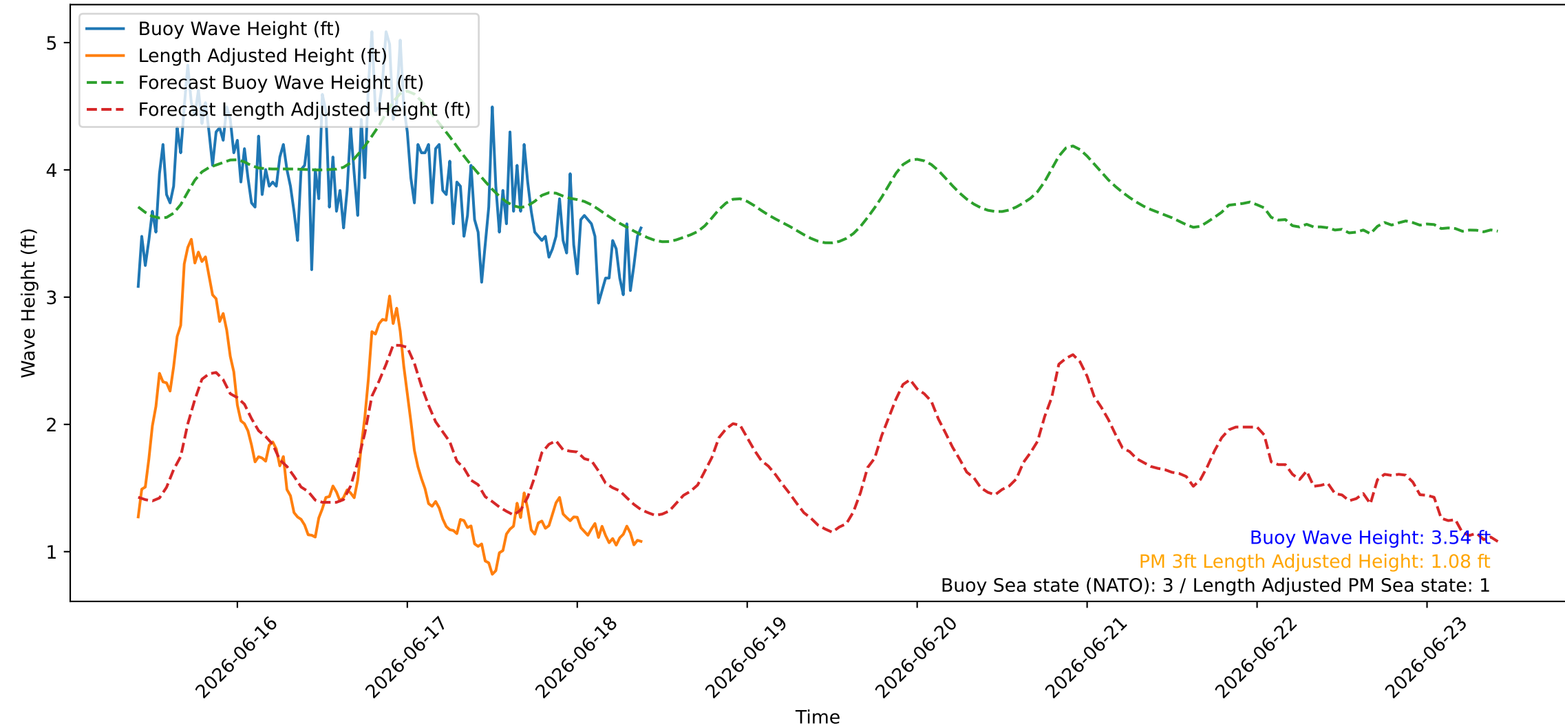
Wave Heights over Time for Green Beach at 2026-06-18 09:51:13
