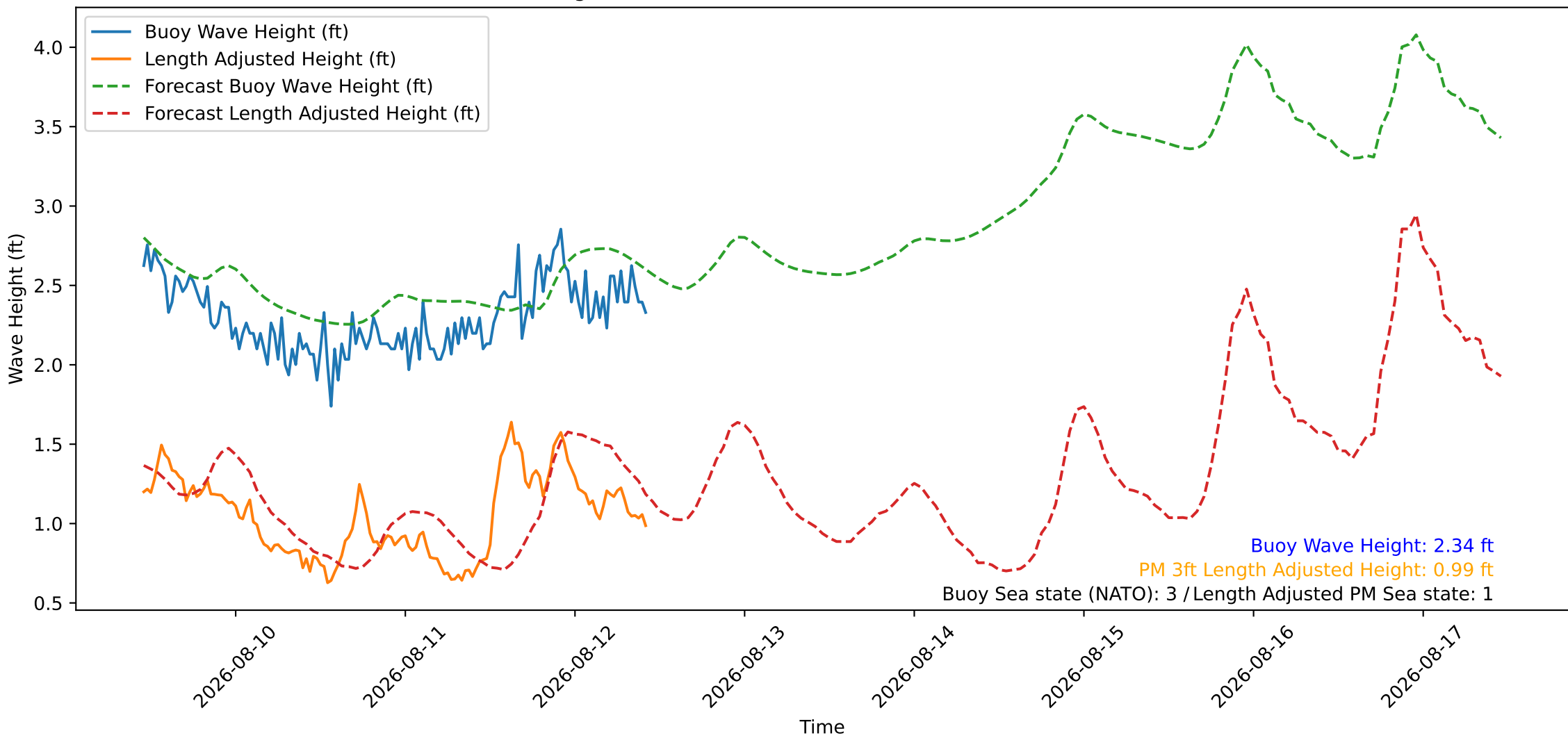
Wave Heights over Time for Red Beach at 2026-08-12 10:40:46
