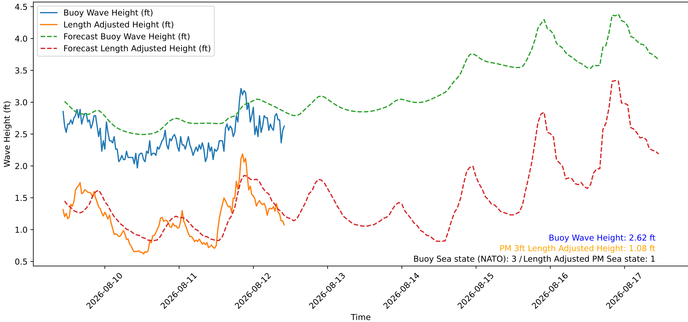
Wave Heights over Time for Green Beach at 2026-08-12 10:41:09
