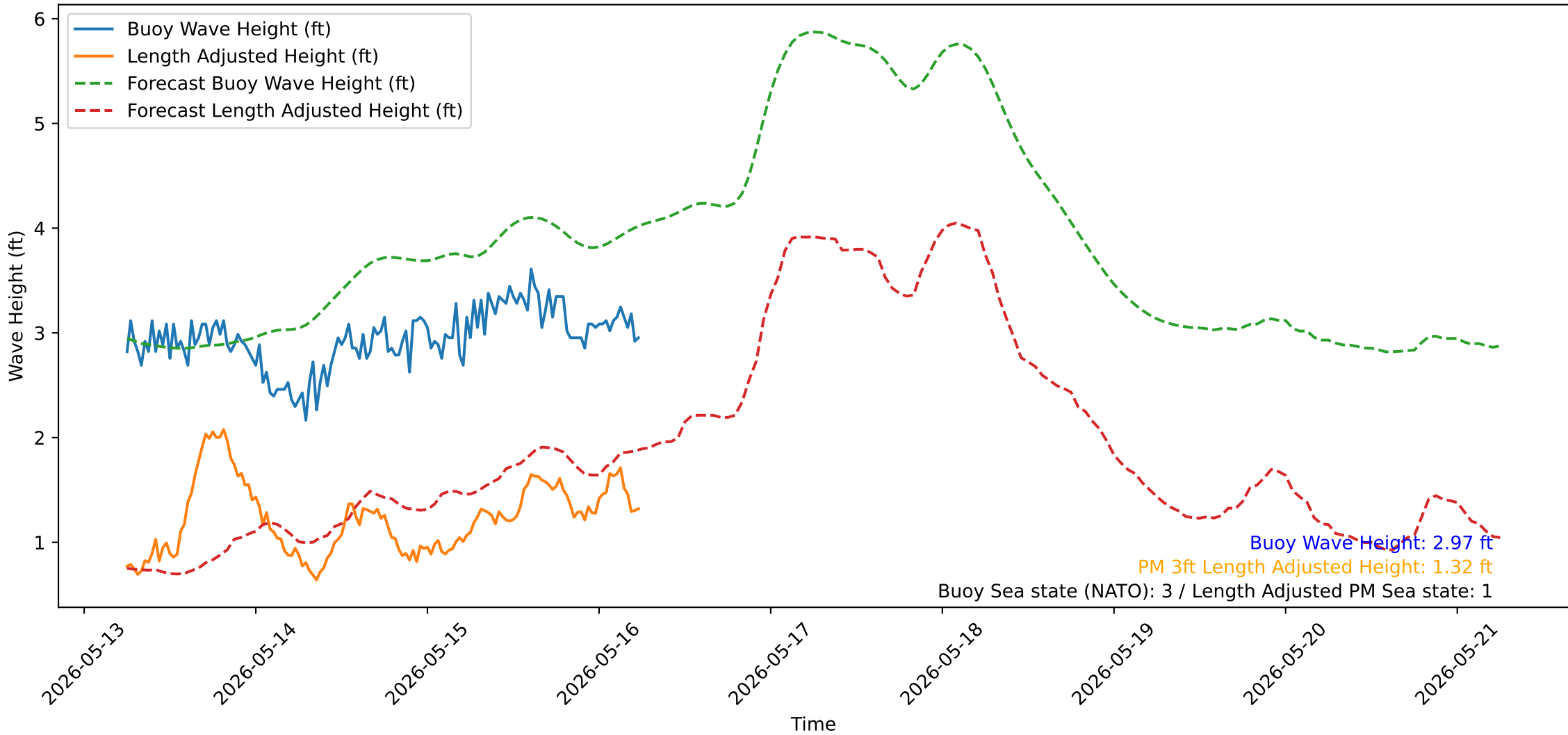
Wave Heights over Time for Oceanside Harbor at 2026-05-16 06:10:31
