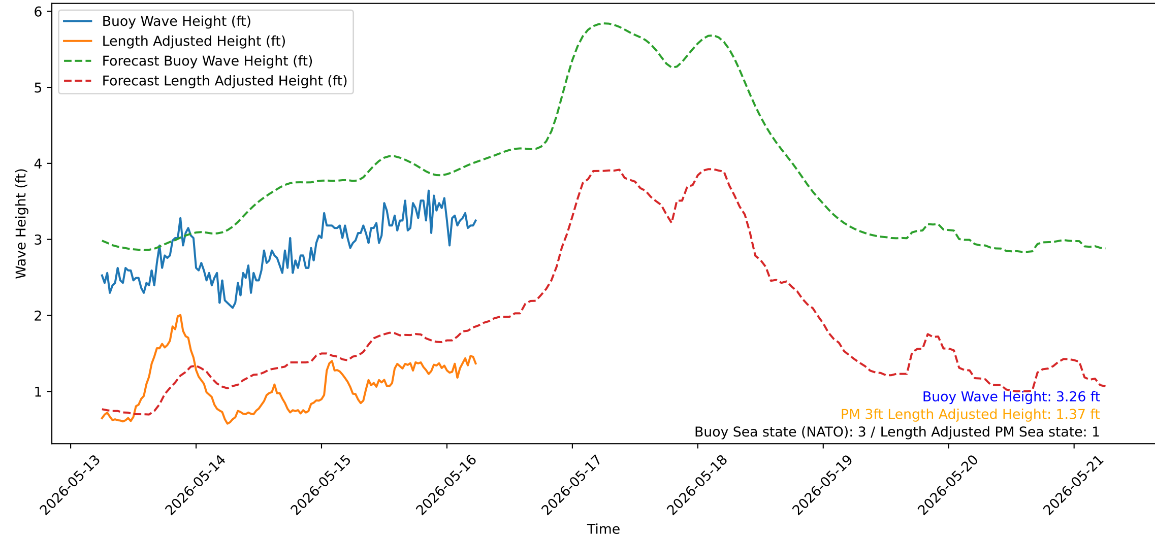
Wave Heights over Time for Green Beach at 2026-05-16 06:11:12
