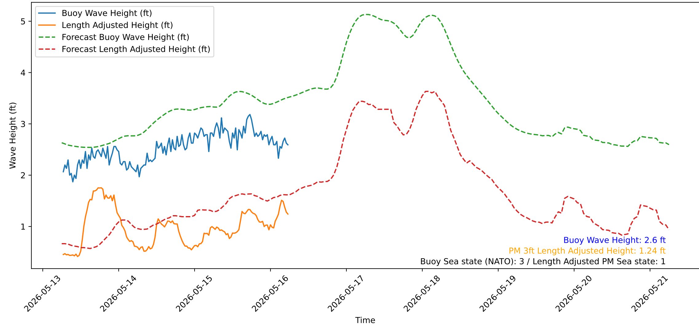
Wave Heights over Time for Red Beach at 2026-05-16 06:10:50
