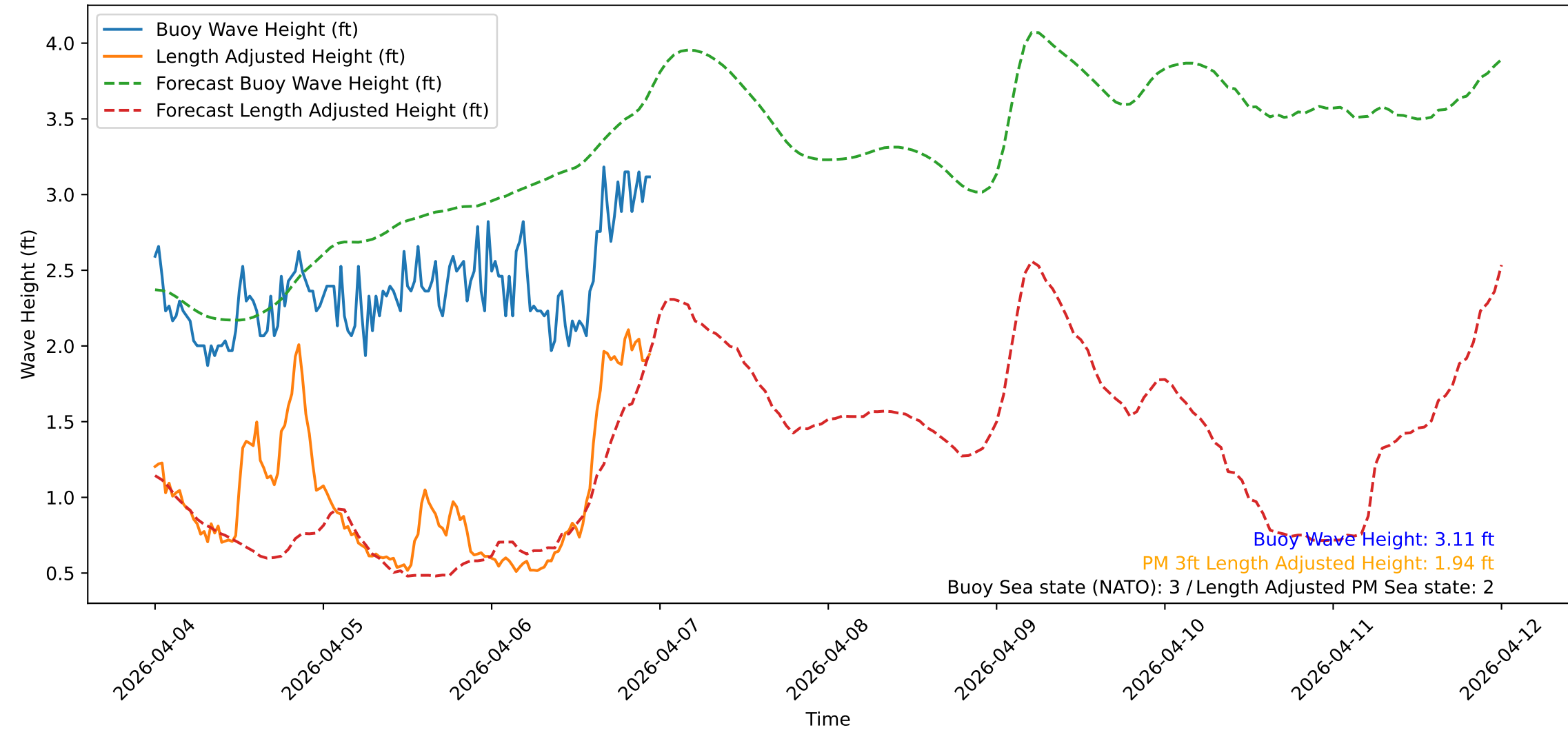
Wave Heights over Time for Red Beach at 2026-04-06 23:30:47
