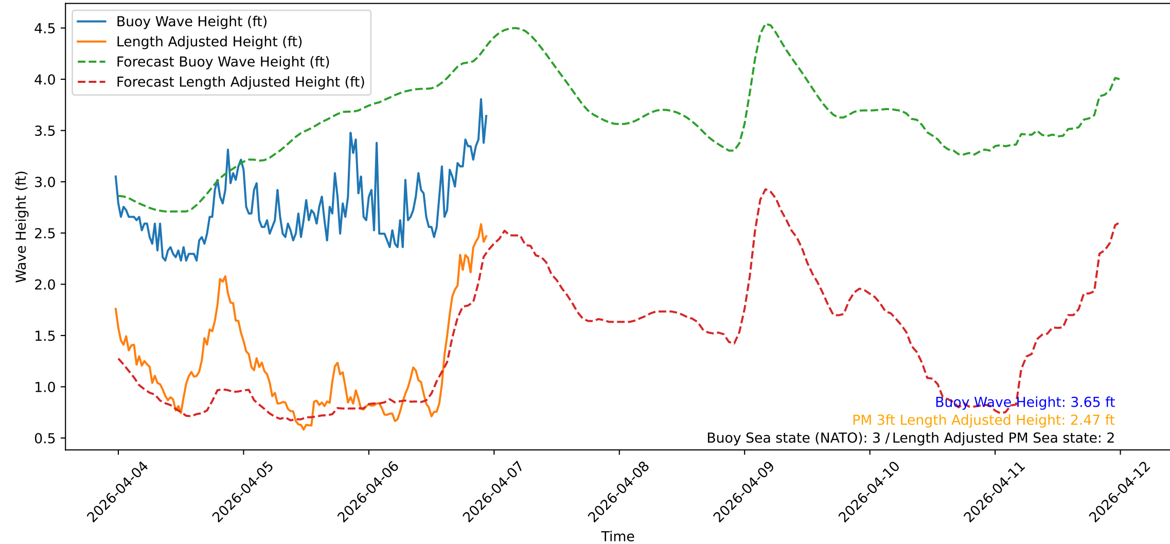
Wave Heights over Time for Green Beach at 2026-04-06 23:31:10
