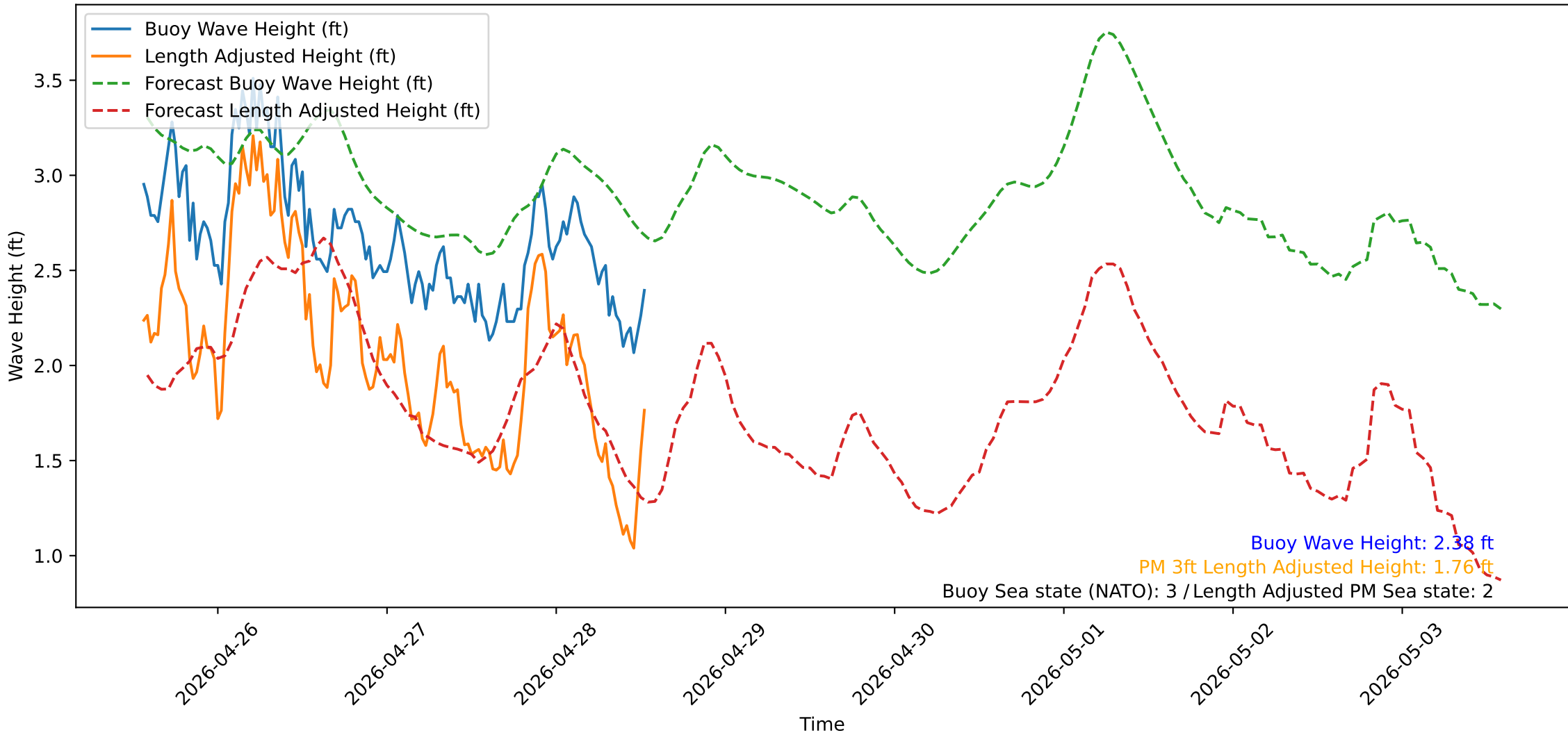
Wave Heights over Time for Green Beach at 2026-04-28 13:31:14
