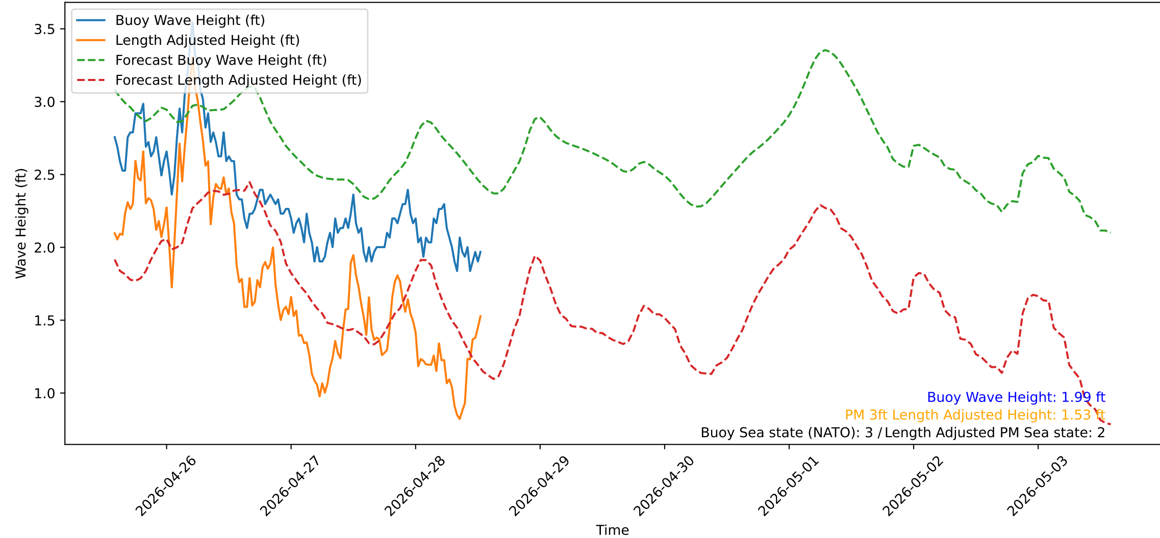
Wave Heights over Time for Red Beach at 2026-04-28 13:30:52
