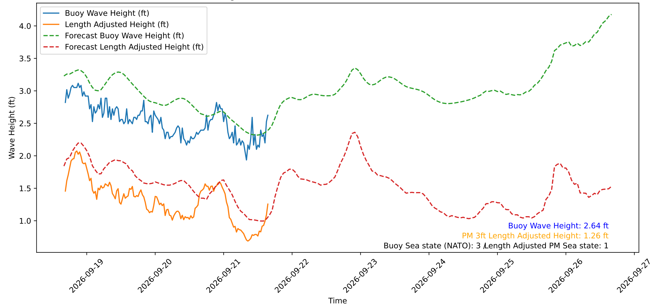
Wave Heights over Time for Green Beach at 2026-09-21 16:21:13
