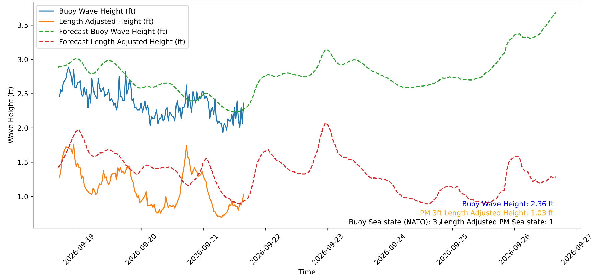
Wave Heights over Time for Red Beach at 2026-09-21 16:20:49
