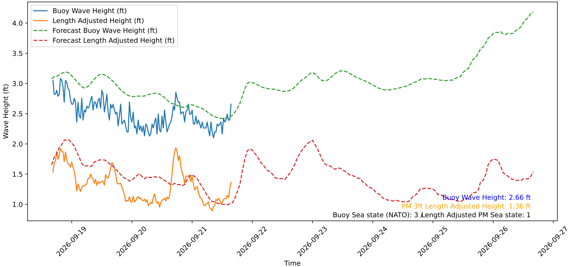
Wave Heights over Time for Oceanside Harbor at 2026-09-21 16:20:29
