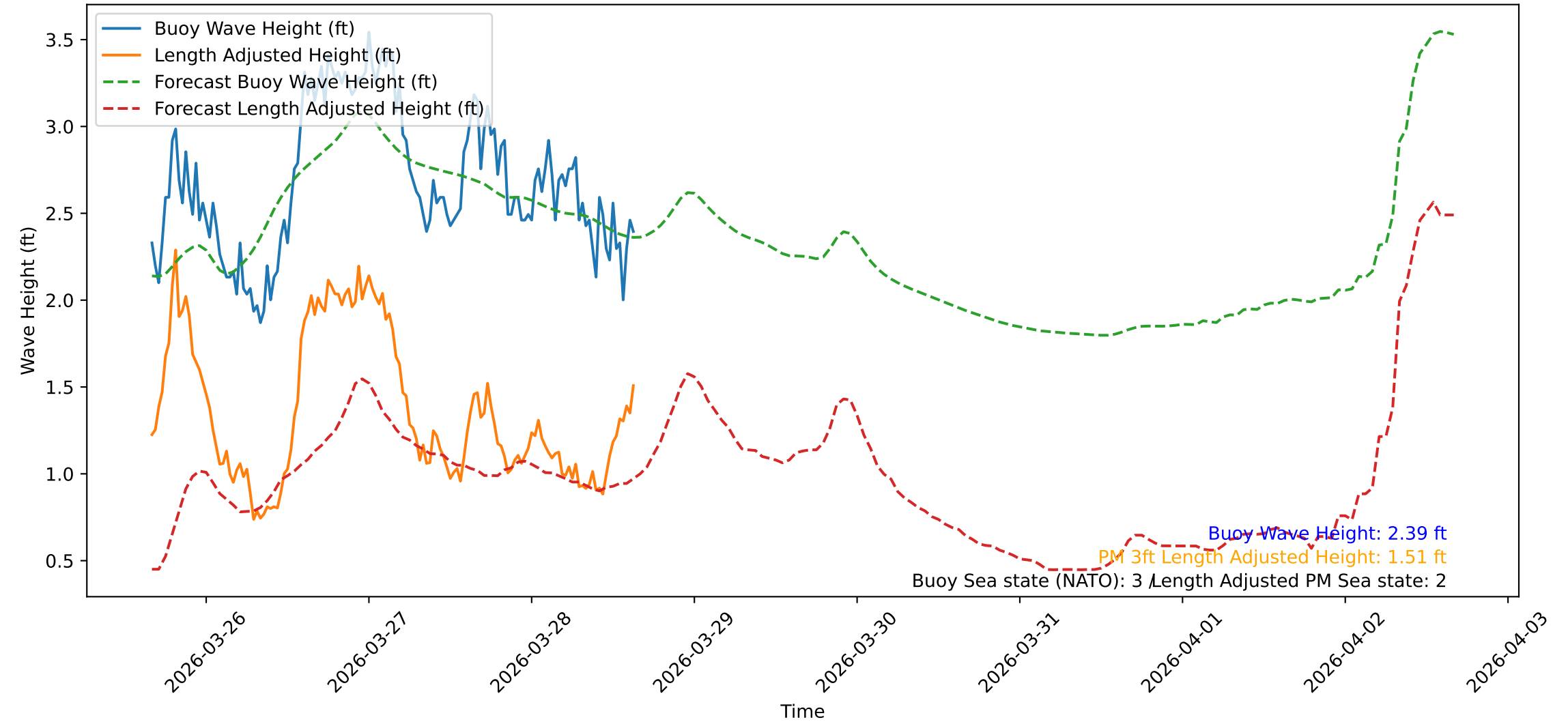
Wave Heights over Time for Green Beach at 2026-03-28 15:51:08
