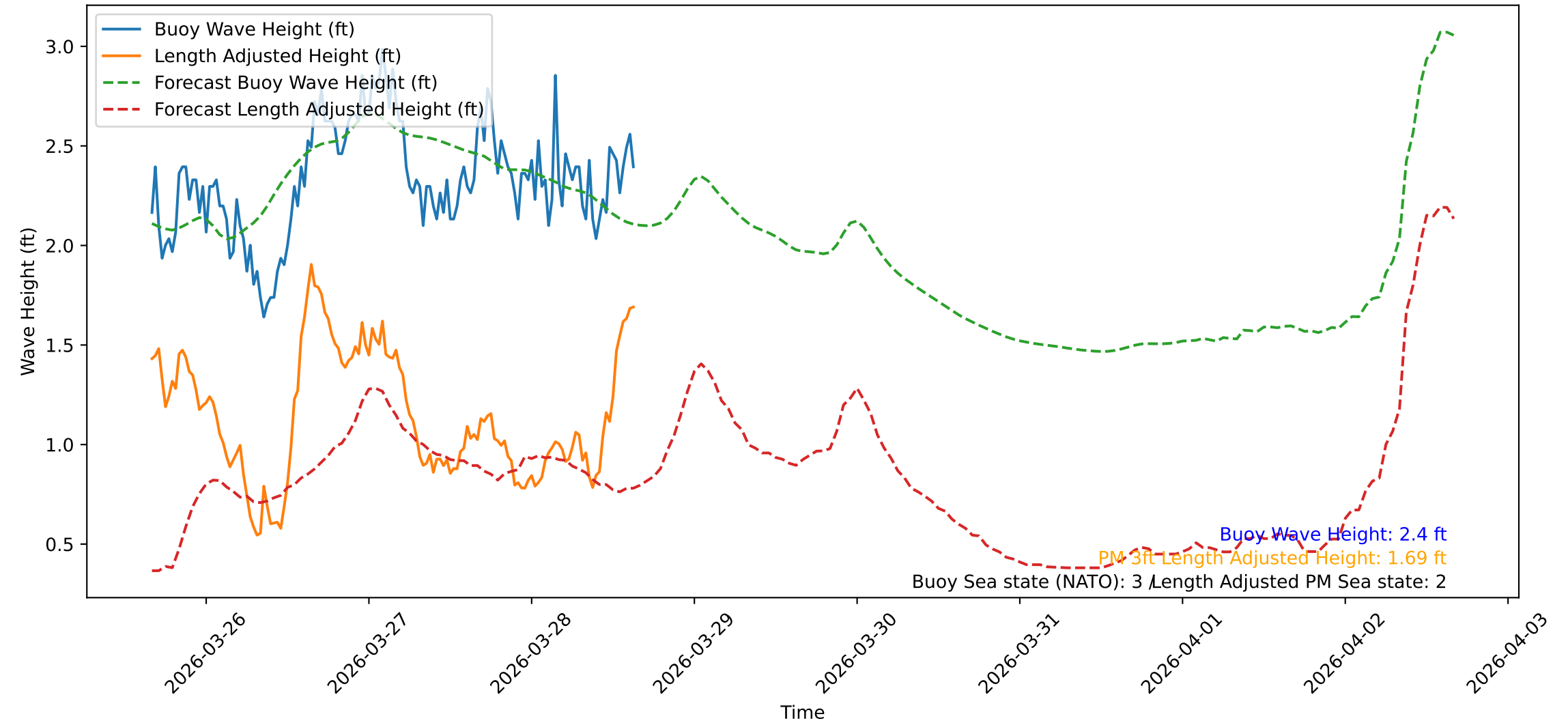
Wave Heights over Time for Red Beach at 2026-03-28 15:50:47
