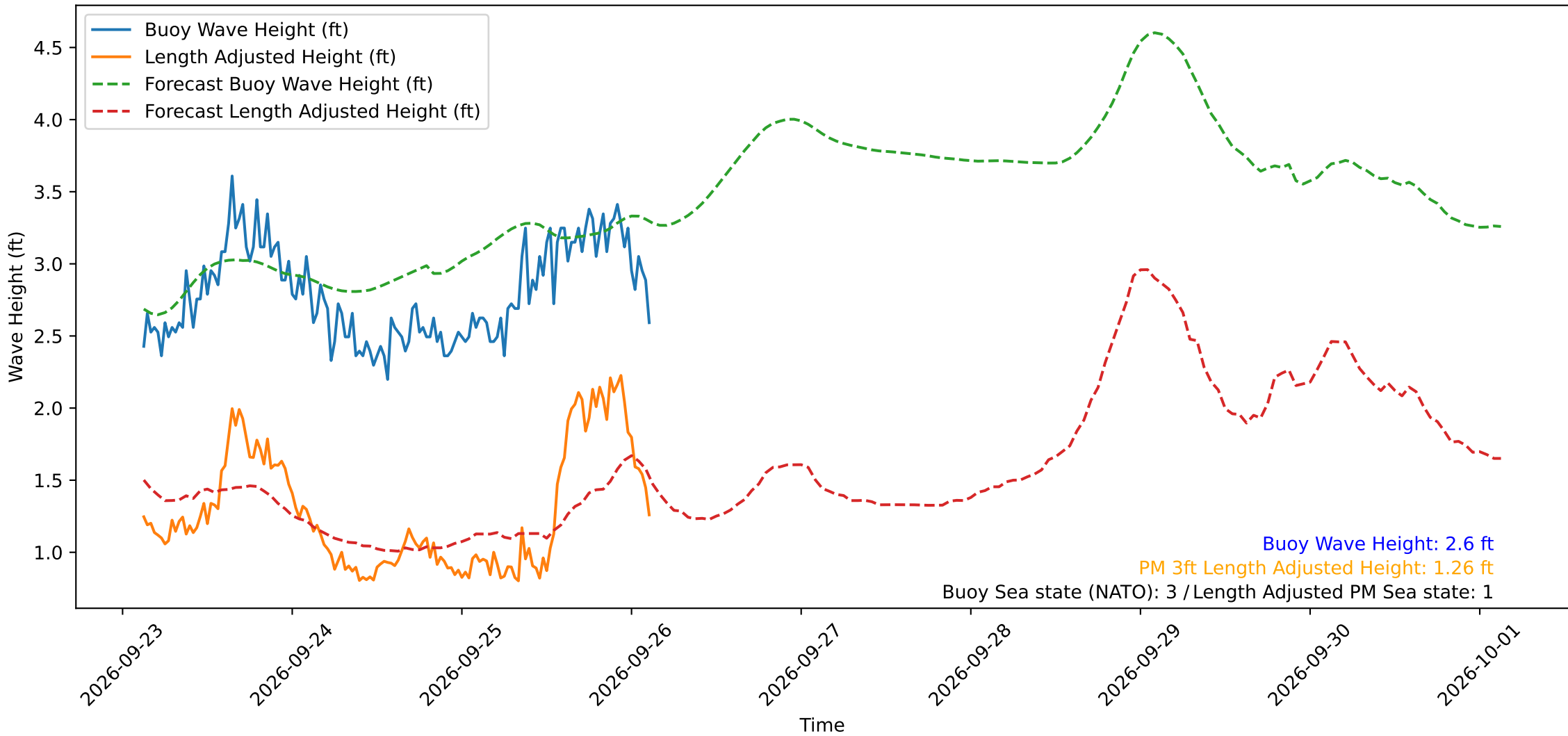
Wave Heights over Time for Oceanside Harbor at 2026-09-26 03:10:30
