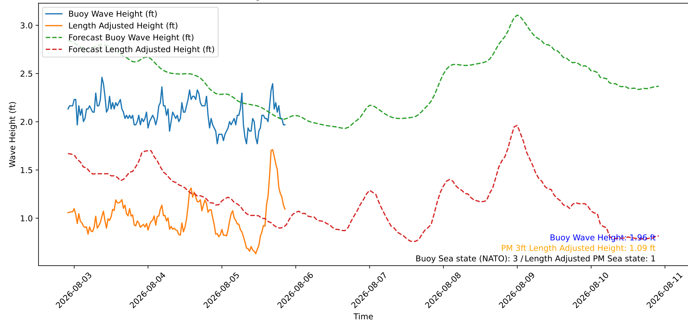
Wave Heights over Time for Red Beach at 2026-08-05 21:30:46
