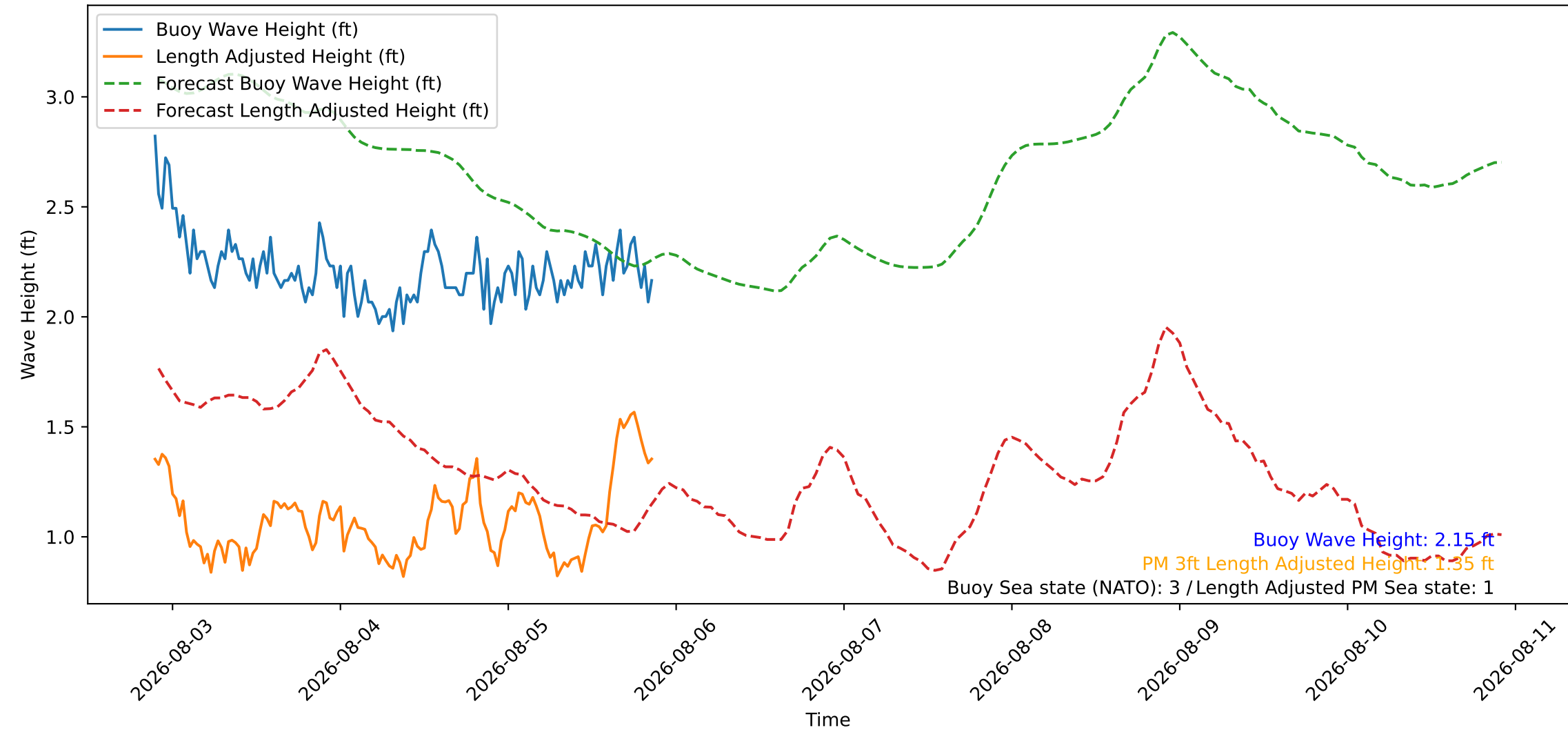
Wave Heights over Time for Green Beach at 2026-08-05 21:31:08
