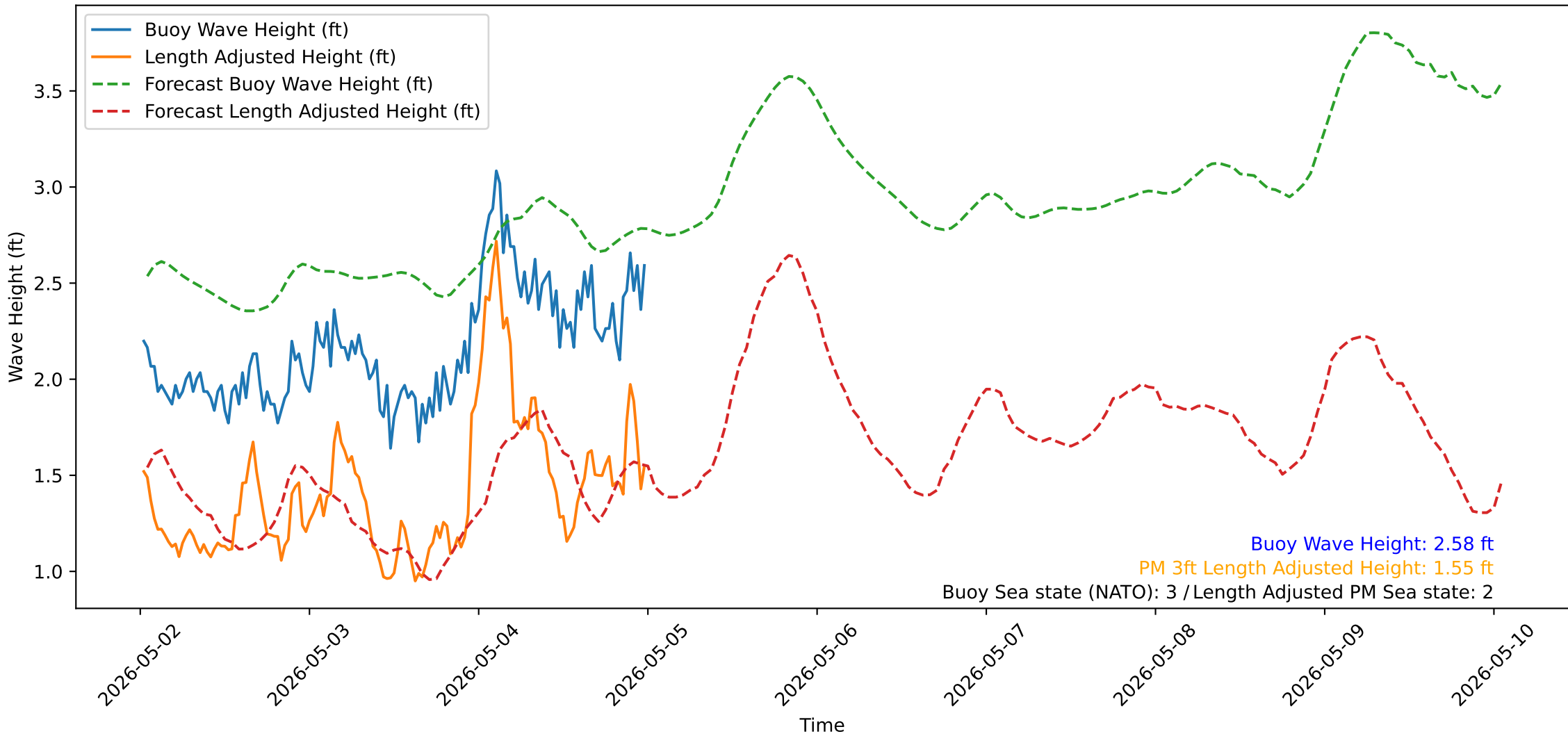
Wave Heights over Time for Oceanside Harbor at 2026-05-05 00:30:31
