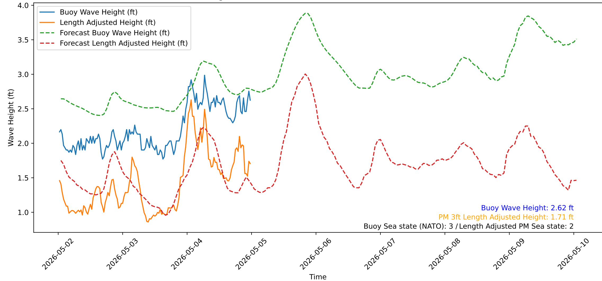
Wave Heights over Time for Green Beach at 2026-05-05 00:31:12
