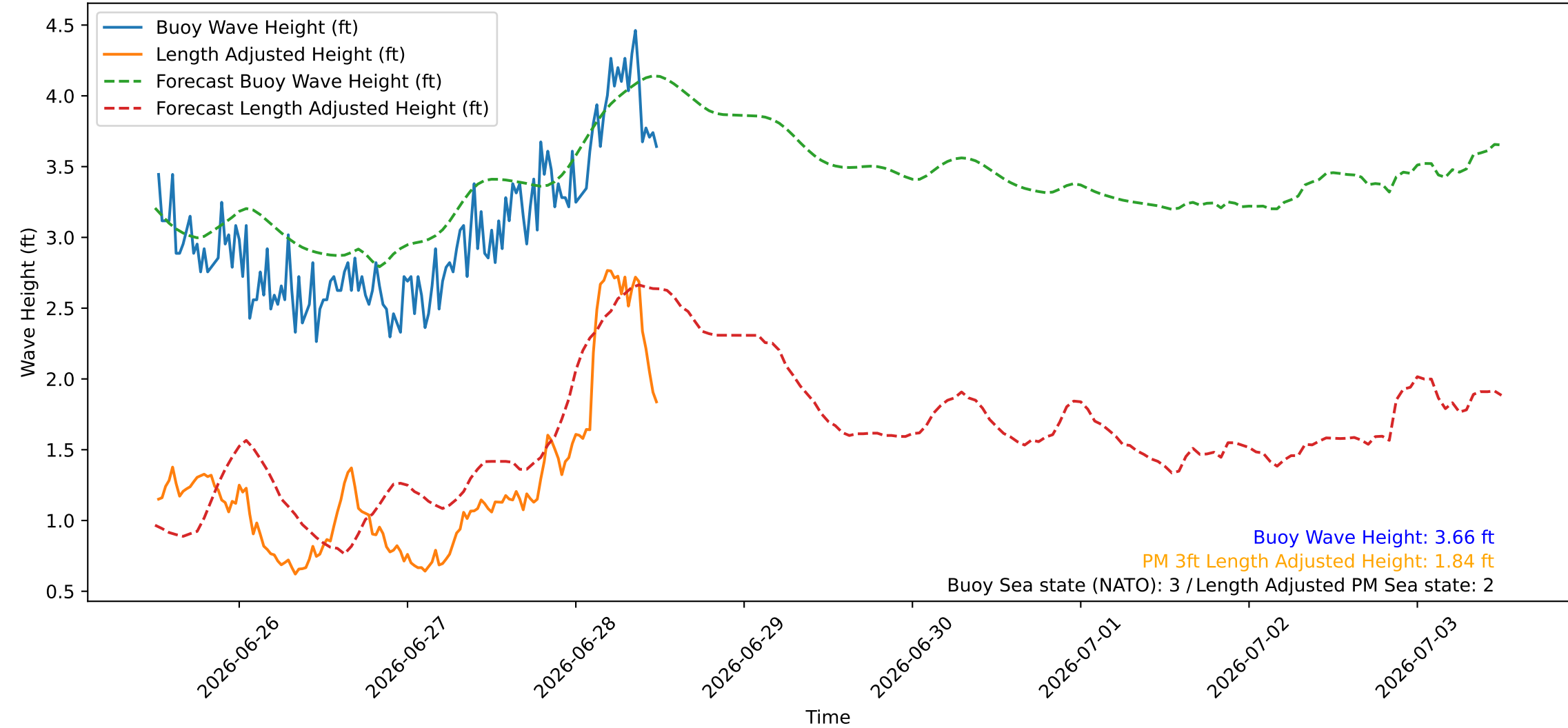
Wave Heights over Time for Red Beach at 2026-06-28 12:10:46
