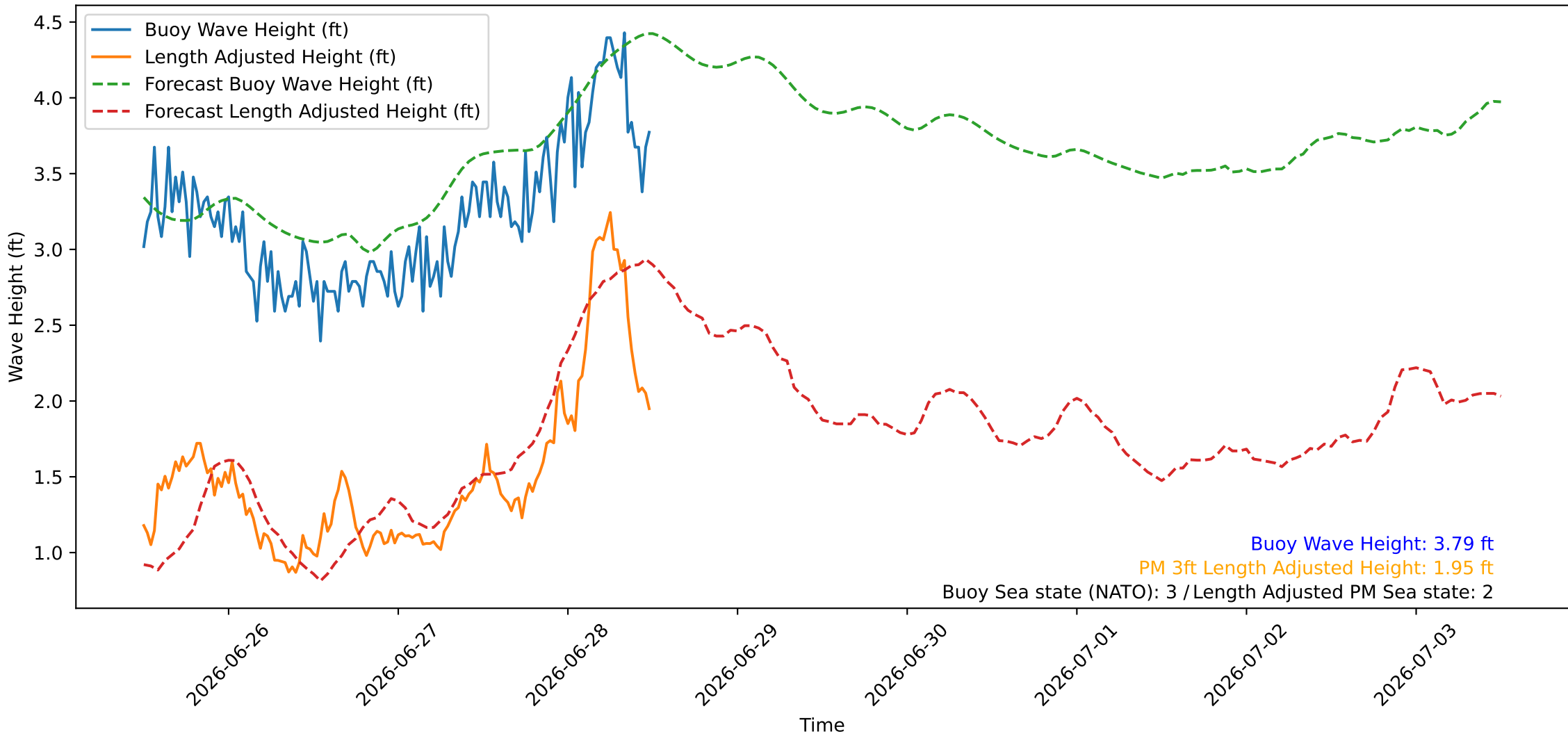
Wave Heights over Time for Oceanside Harbor at 2026-06-28 12:10:27
