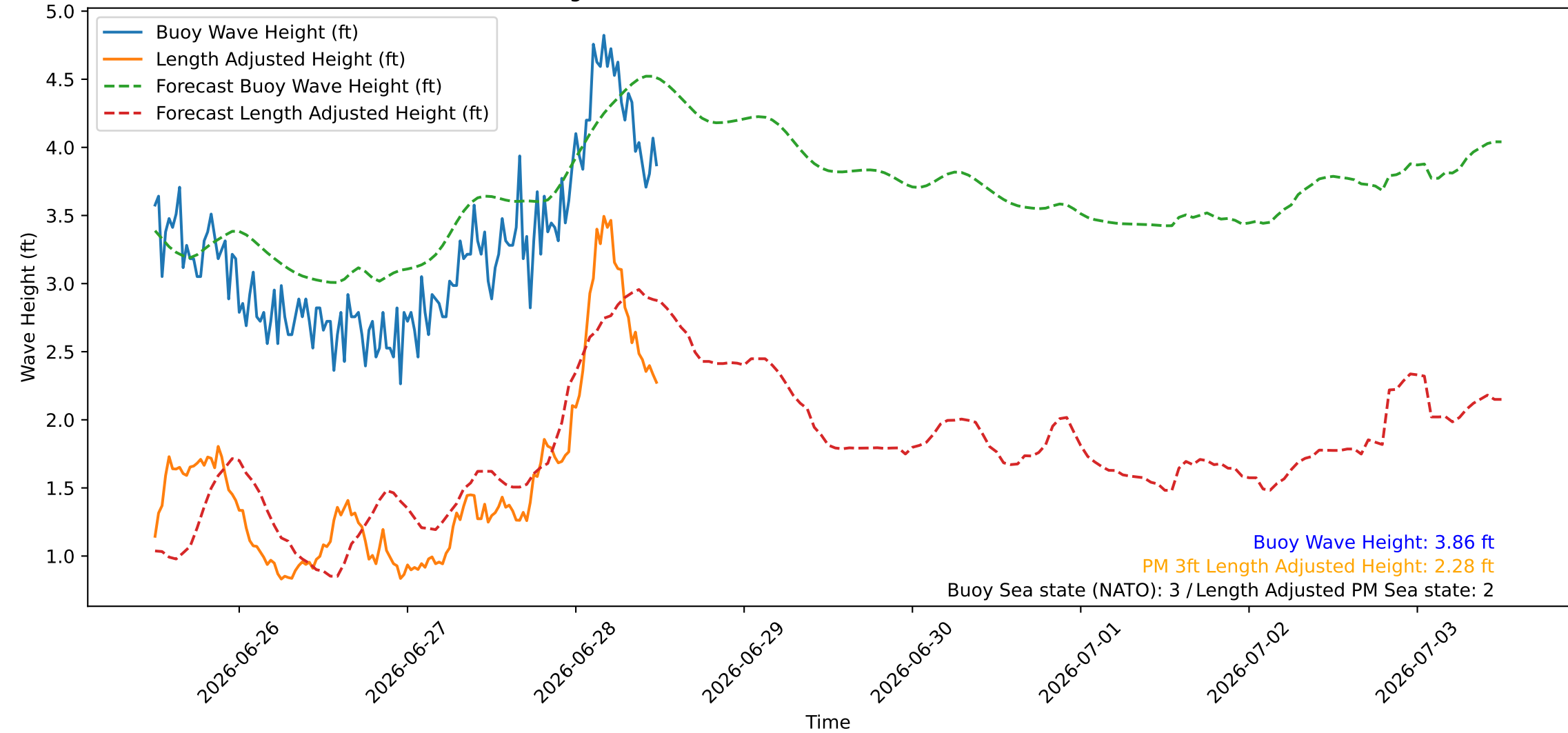
Wave Heights over Time for Green Beach at 2026-06-28 12:11:09
