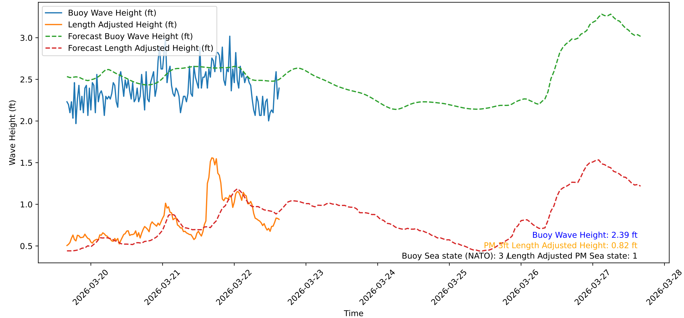
Wave Heights over Time for Oceanside Harbor at 2026-03-22 15:50:31
