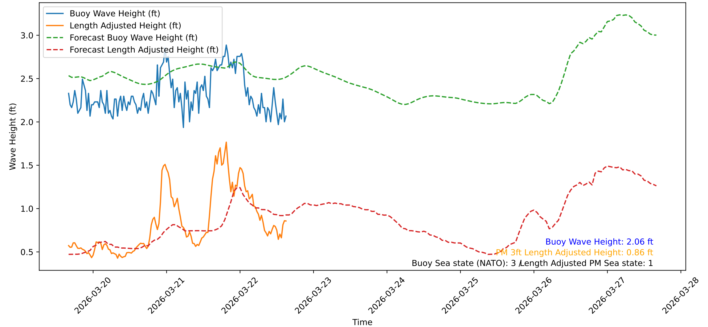
Wave Heights over Time for Green Beach at 2026-03-22 15:51:09
