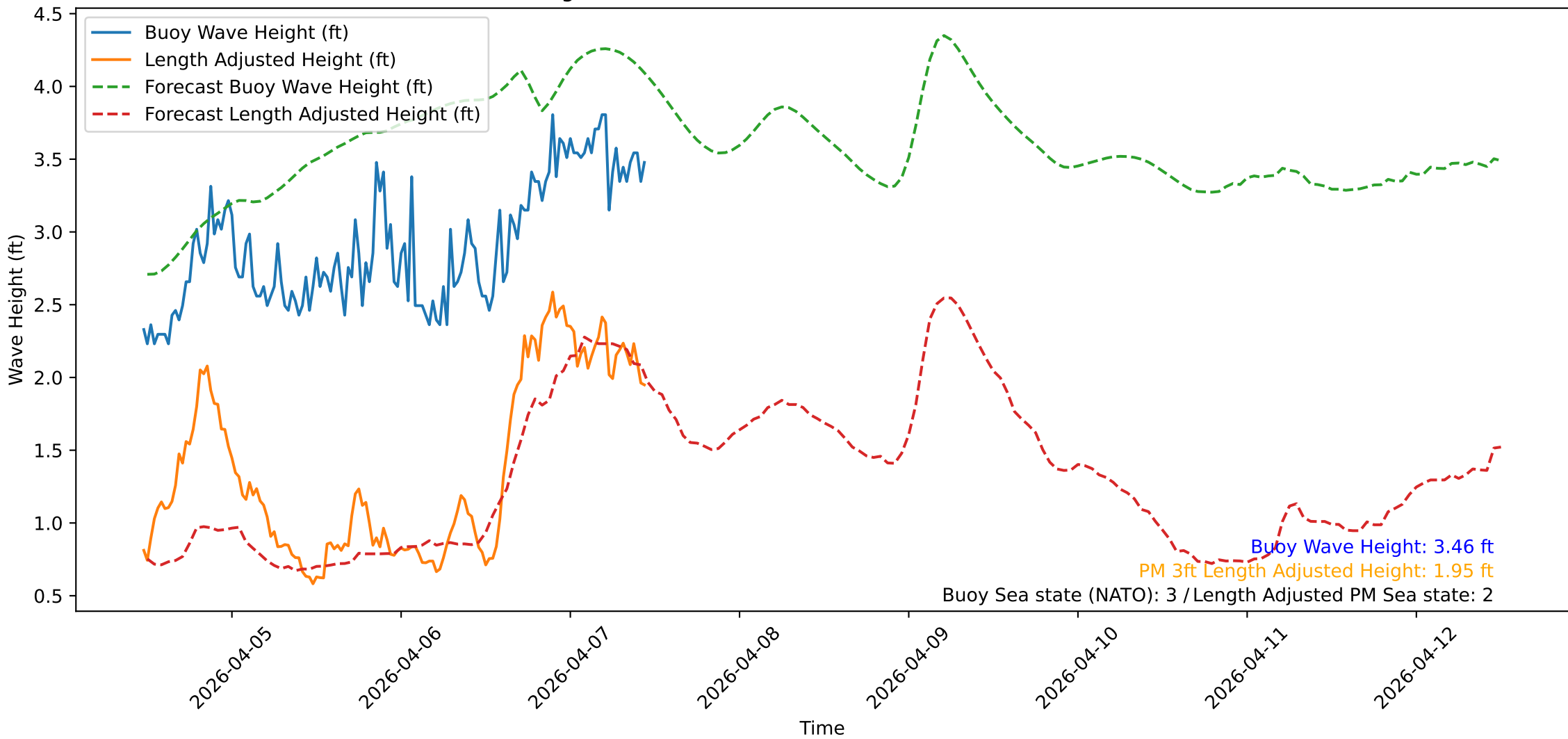
Wave Heights over Time for Green Beach at 2026-04-07 11:31:09
