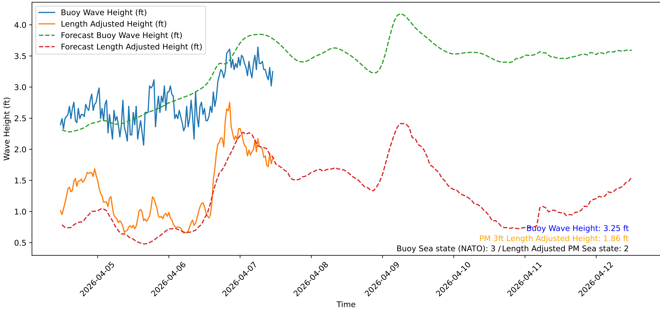
Wave Heights over Time for Oceanside Harbor at 2026-04-07 11:30:31
