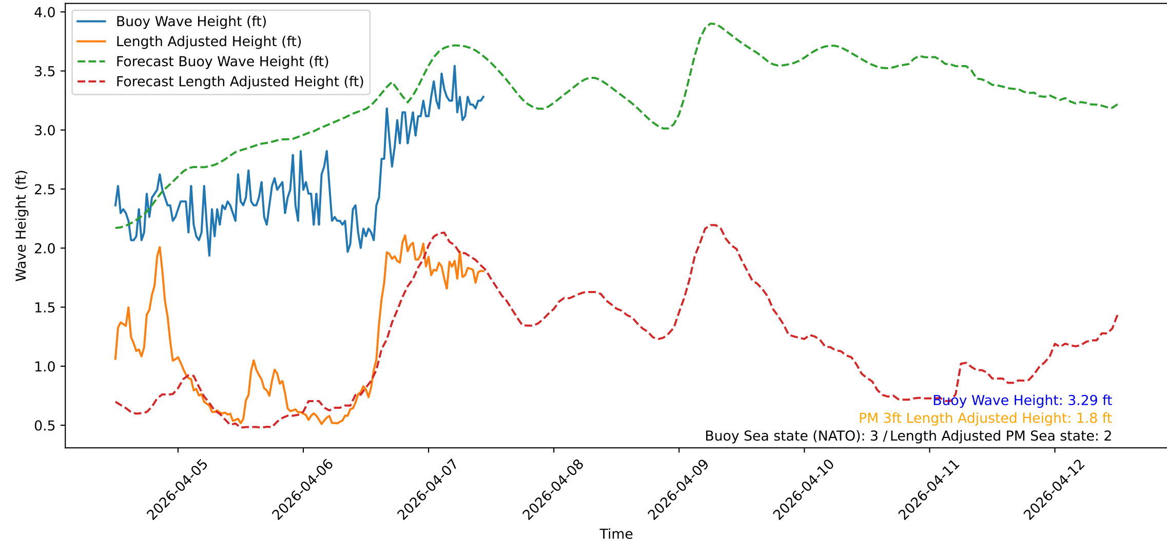
Wave Heights over Time for Red Beach at 2026-04-07 11:30:47
