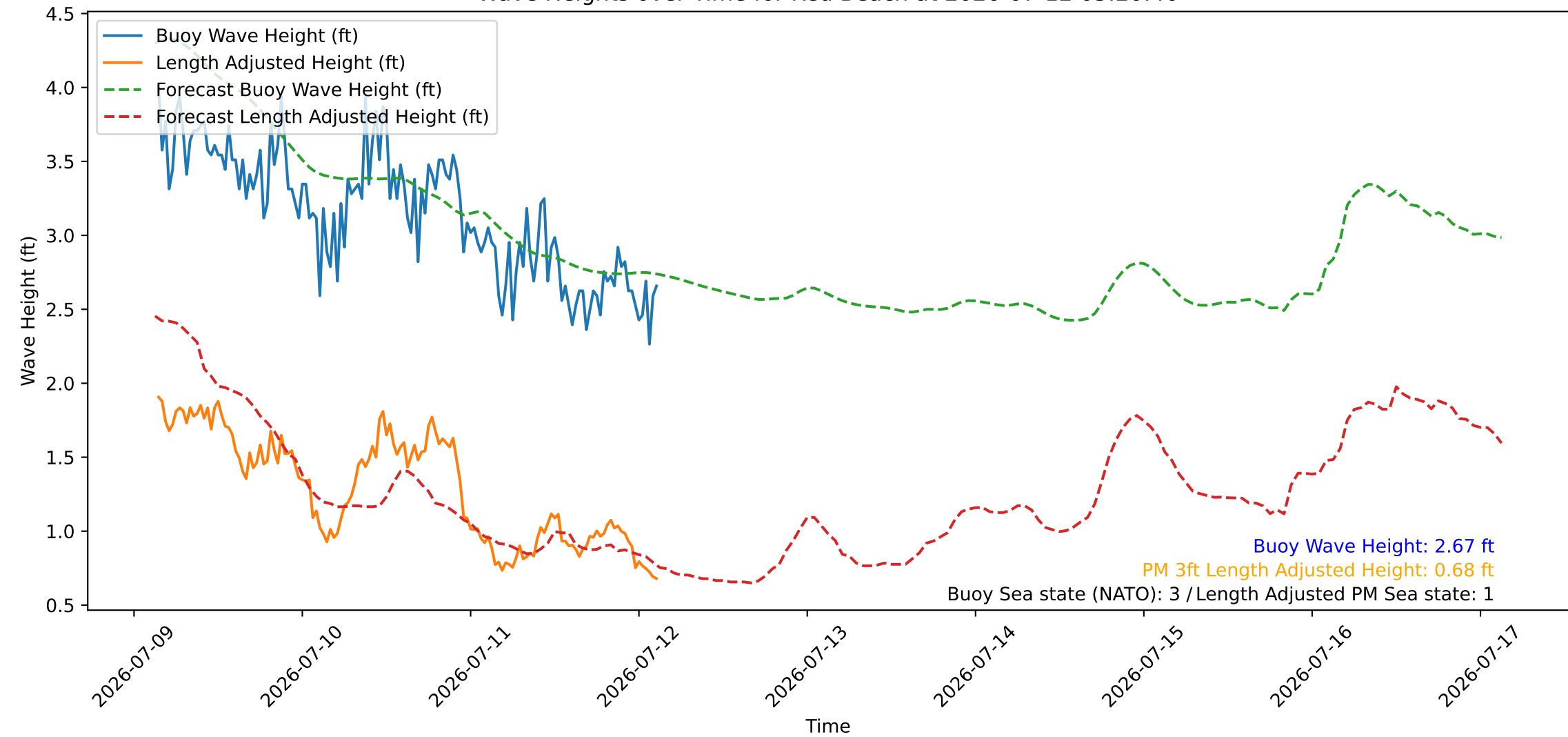
Wave Heights over Time for Red Beach at 2026-07-12 03:20:46
