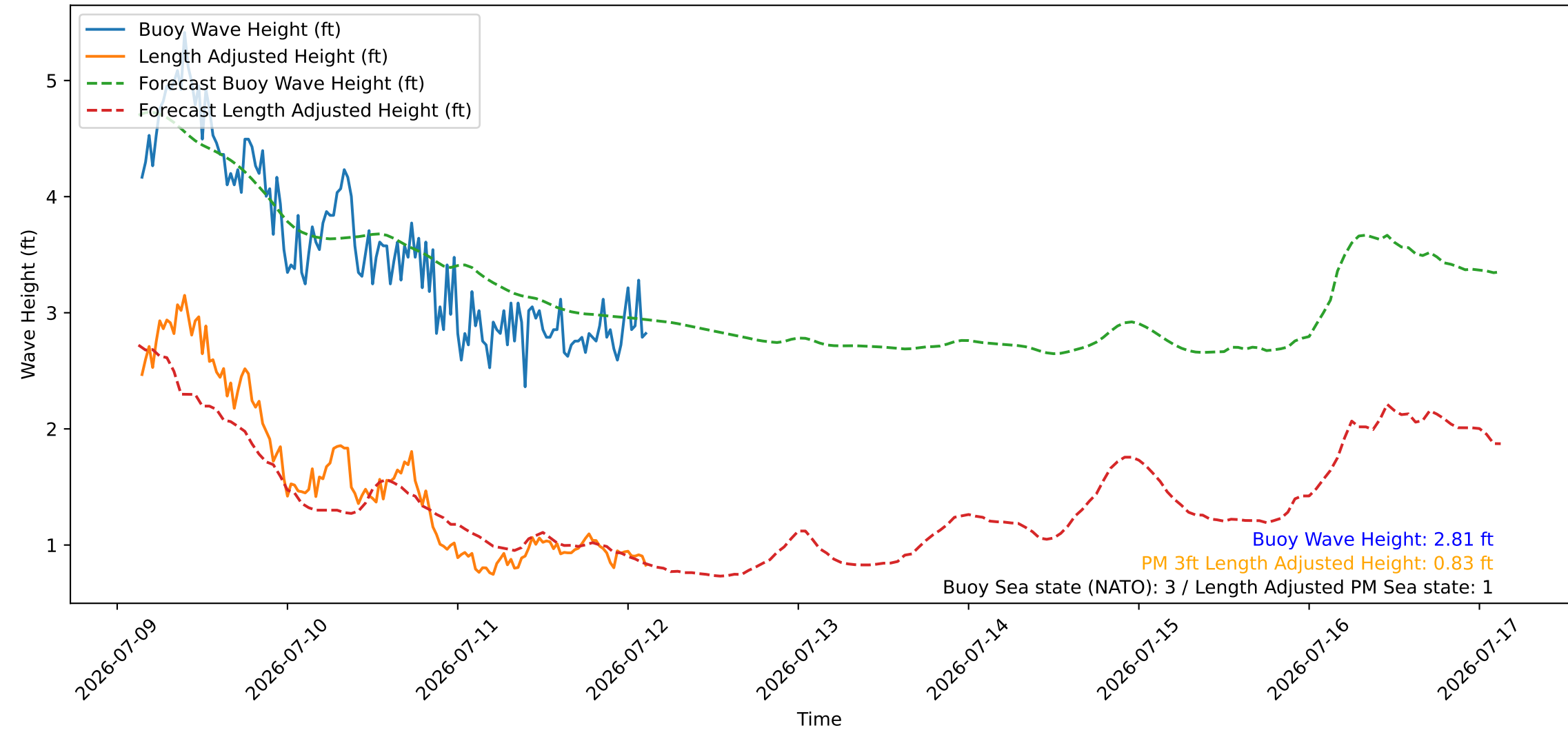
Wave Heights over Time for Oceanside Harbor at 2026-07-12 03:20:26
