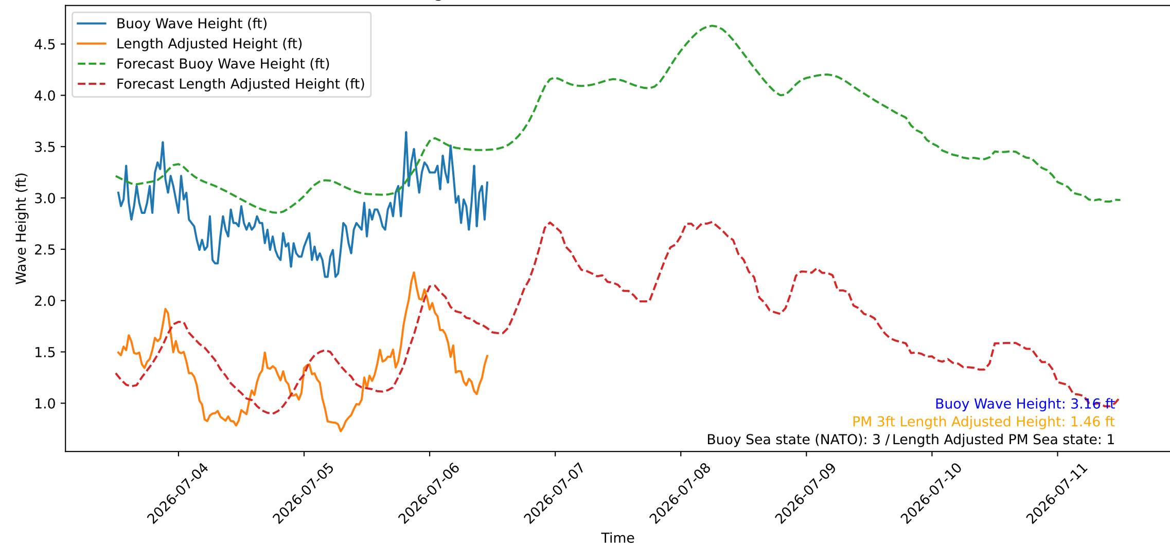
Wave Heights over Time for Red Beach at 2026-07-06 12:00:45
