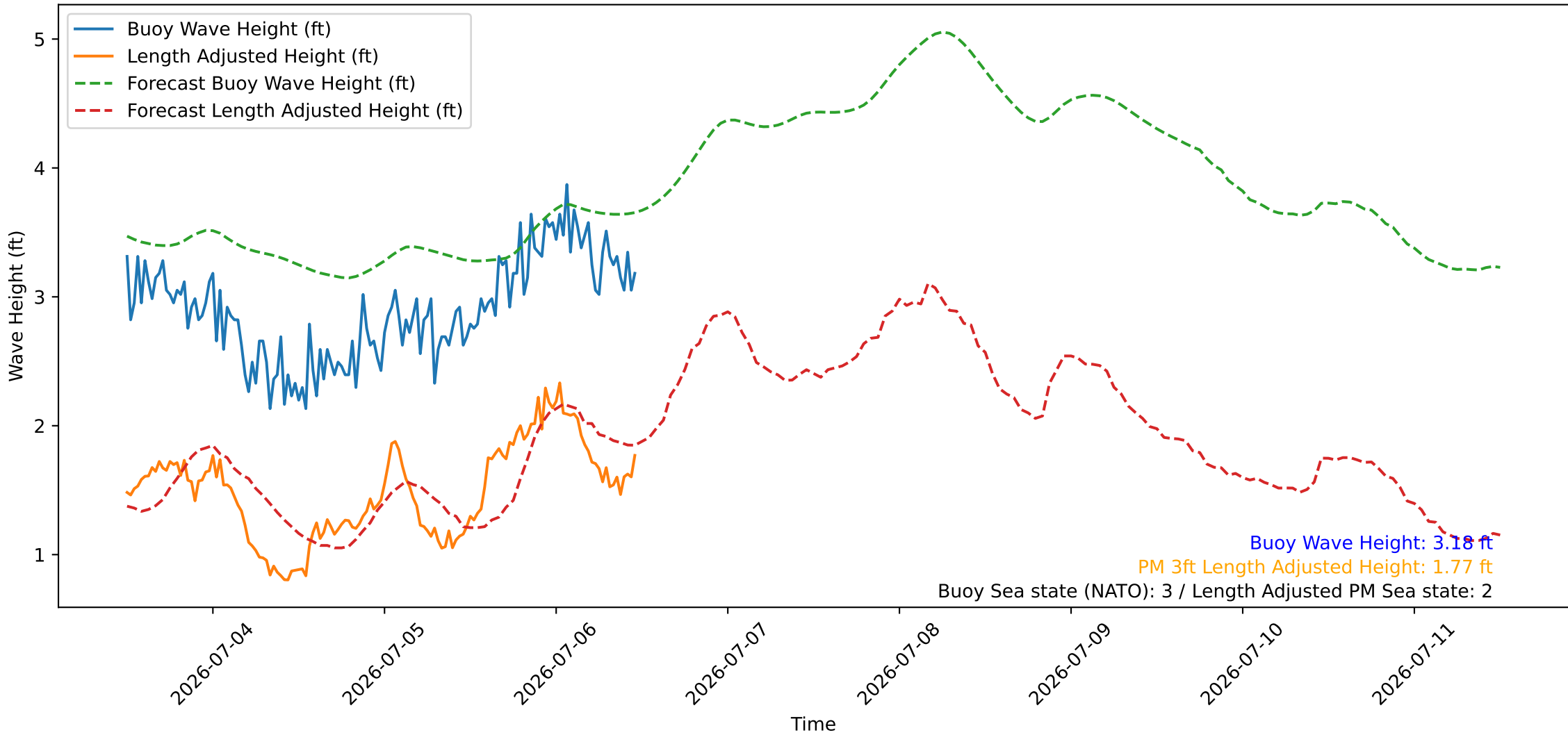
Wave Heights over Time for Oceanside Harbor at 2026-07-06 12:00:26
