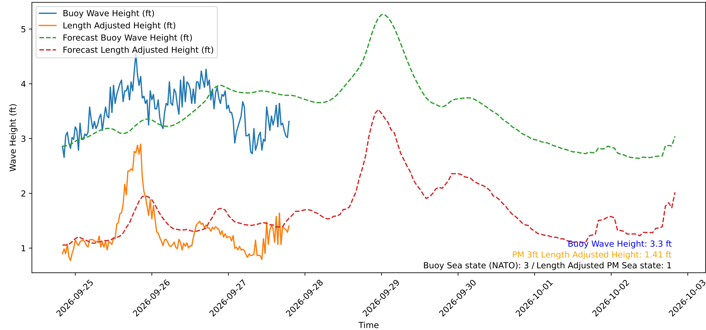
Wave Heights over Time for Green Beach at 2026-09-27 19:51:19
