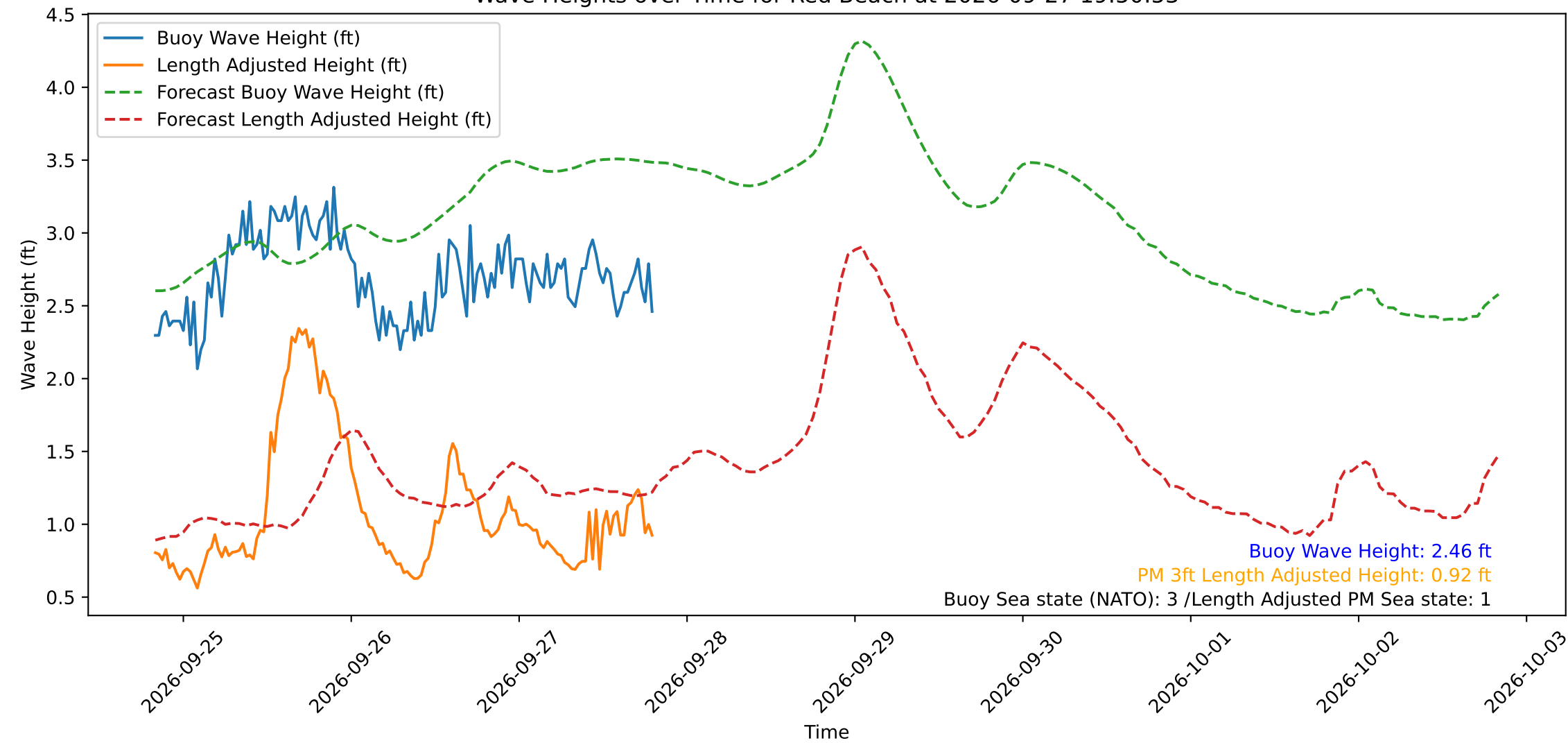
Wave Heights over Time for Red Beach at 2026-09-27 19:50:53
