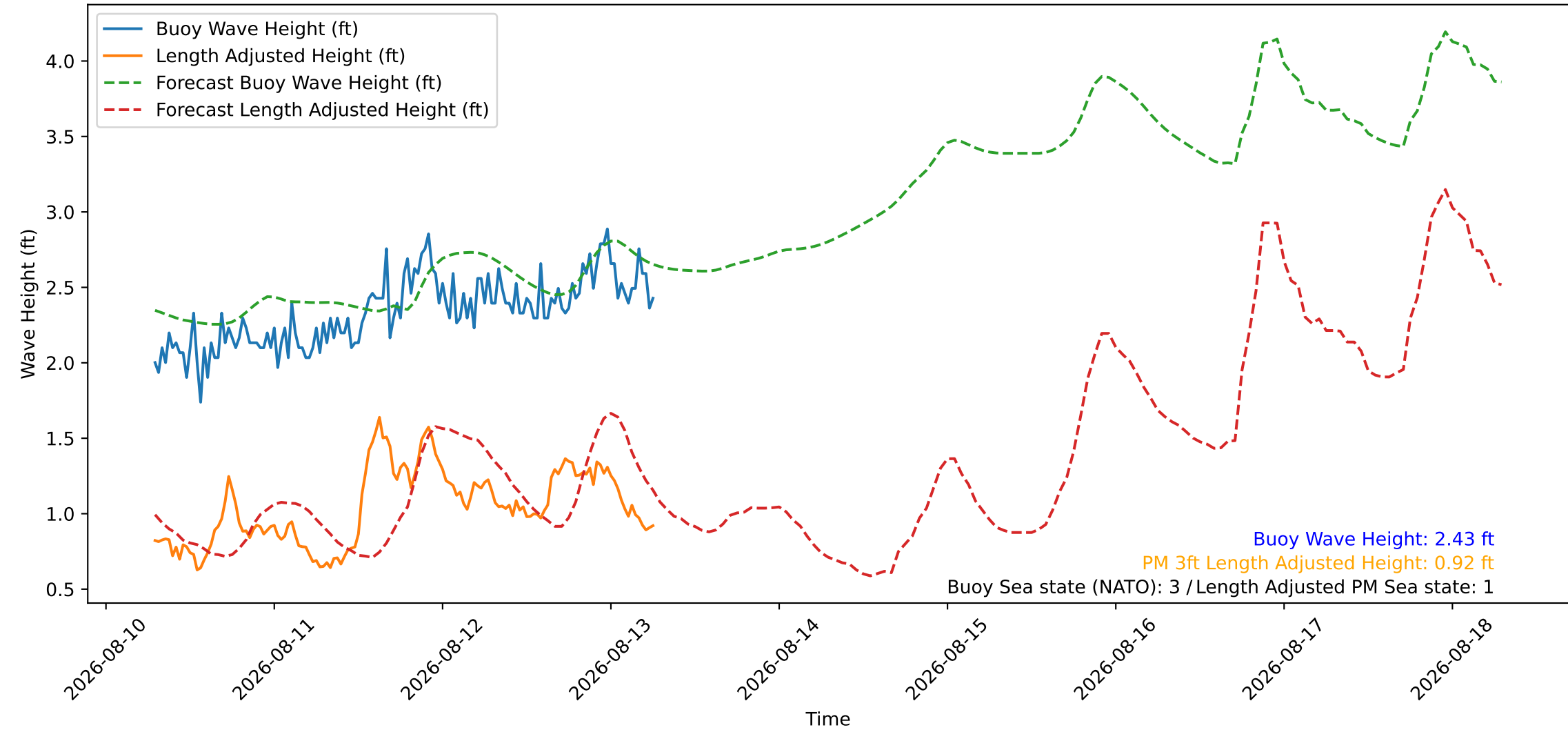
Wave Heights over Time for Red Beach at 2026-08-13 06:50:47
