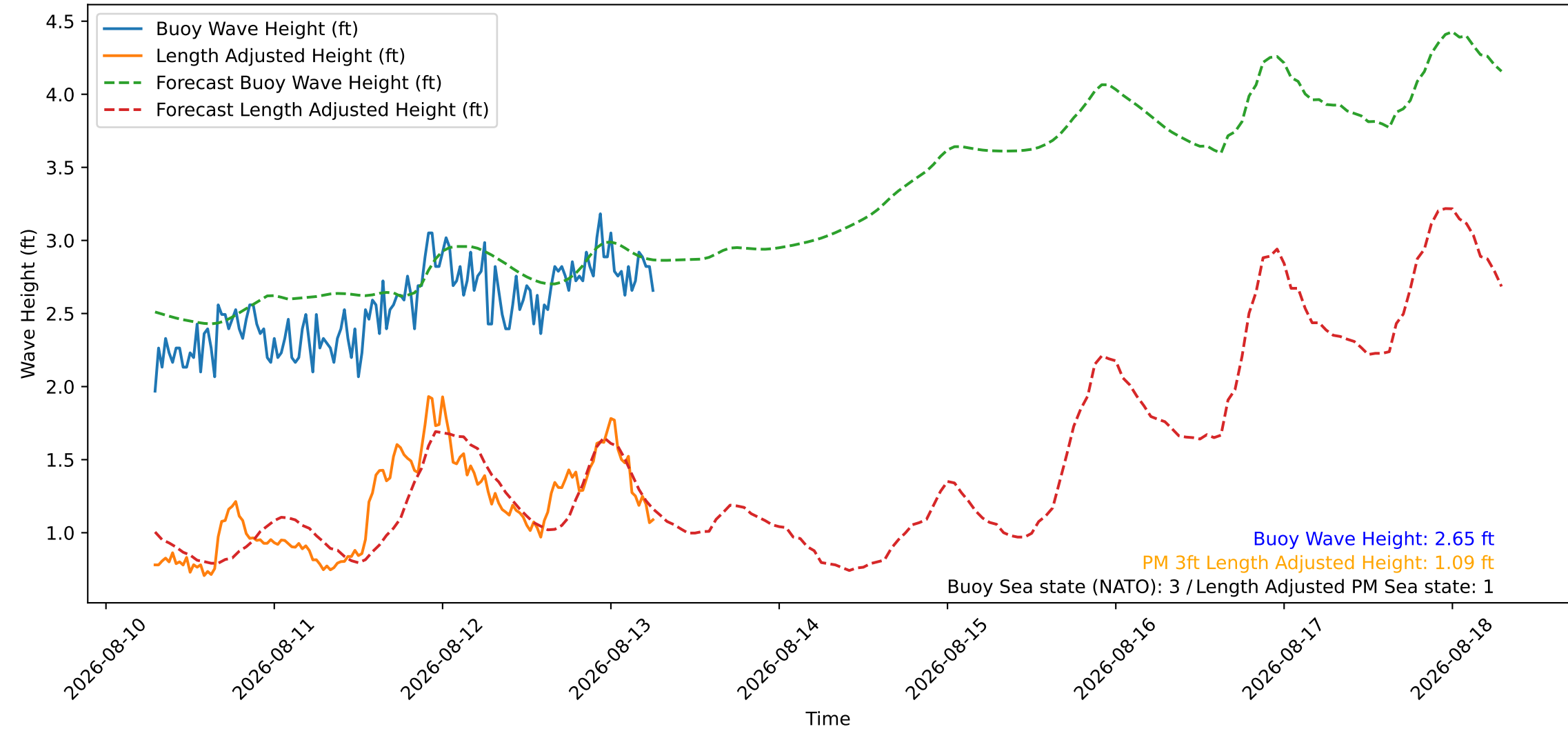
Wave Heights over Time for Oceanside Harbor at 2026-08-13 06:50:27
