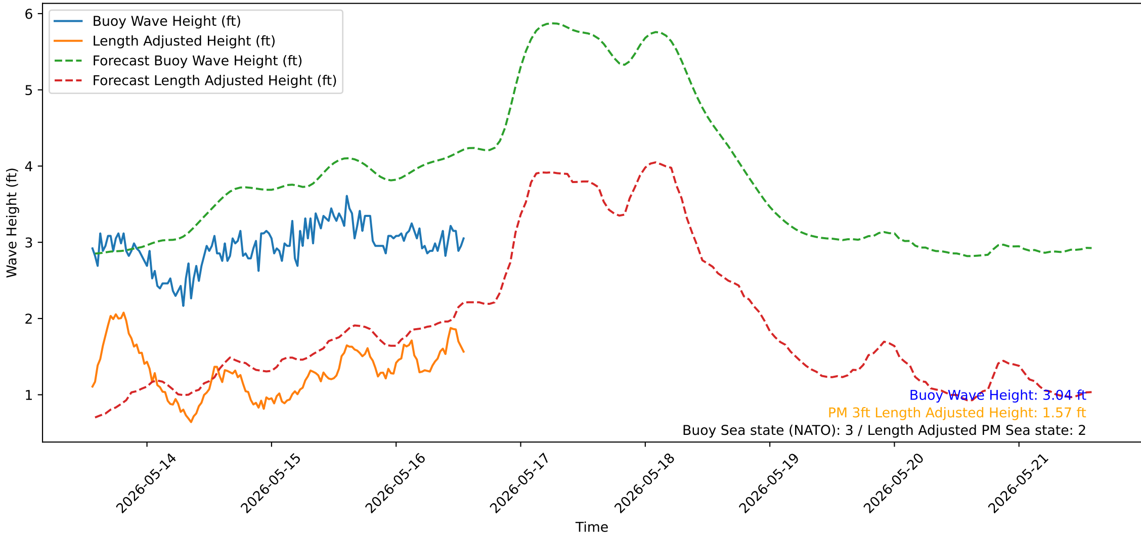
Wave Heights over Time for Oceanside Harbor at 2026-05-16 13:40:32
