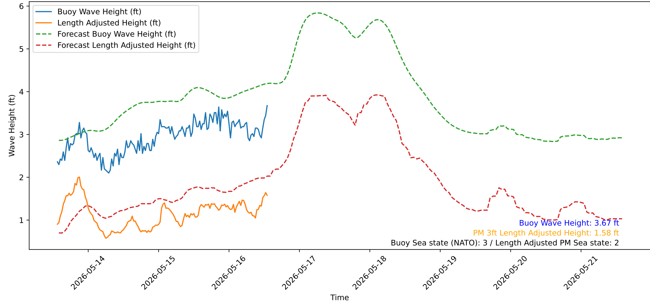
Wave Heights over Time for Green Beach at 2026-05-16 13:41:14
