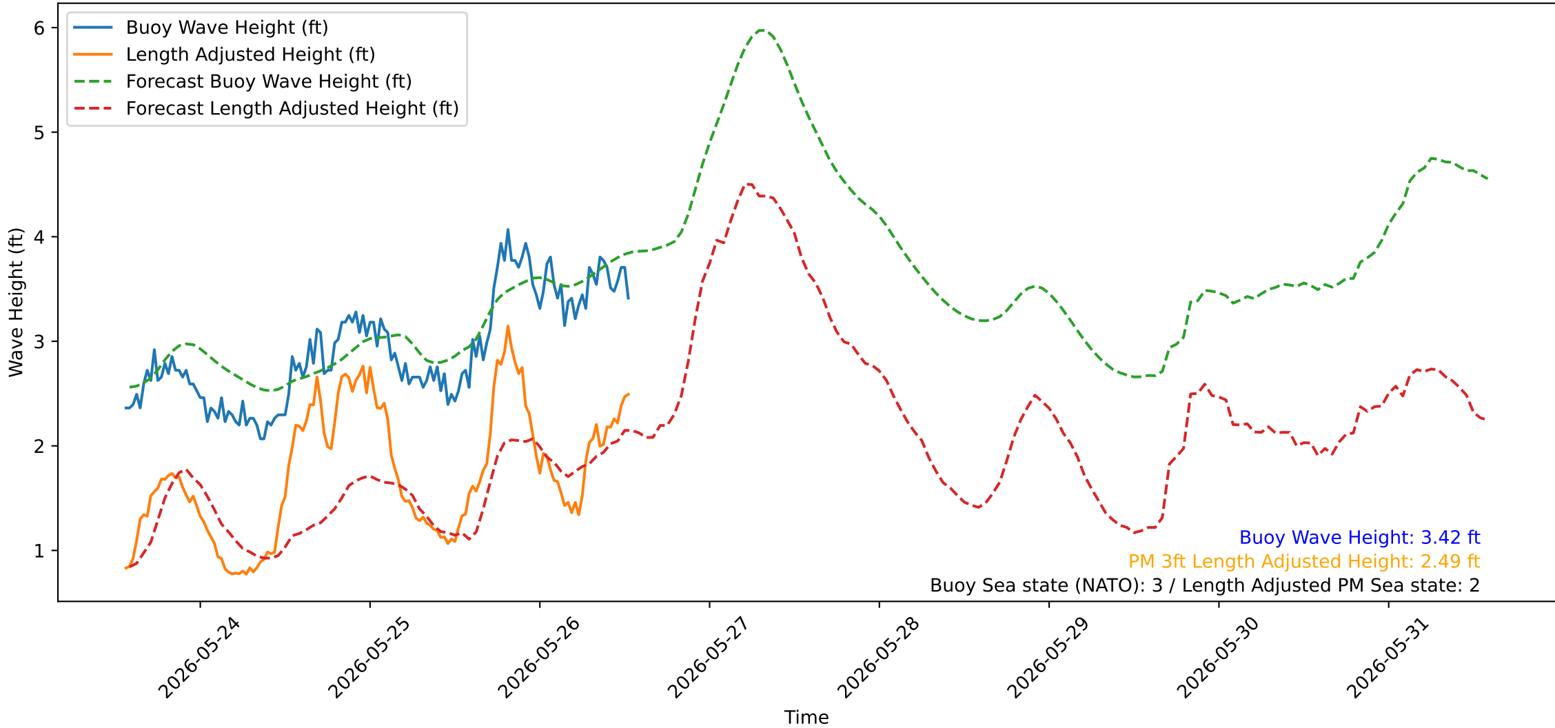
Wave Heights over Time for Green Beach at 2026-05-26 13:41:10
