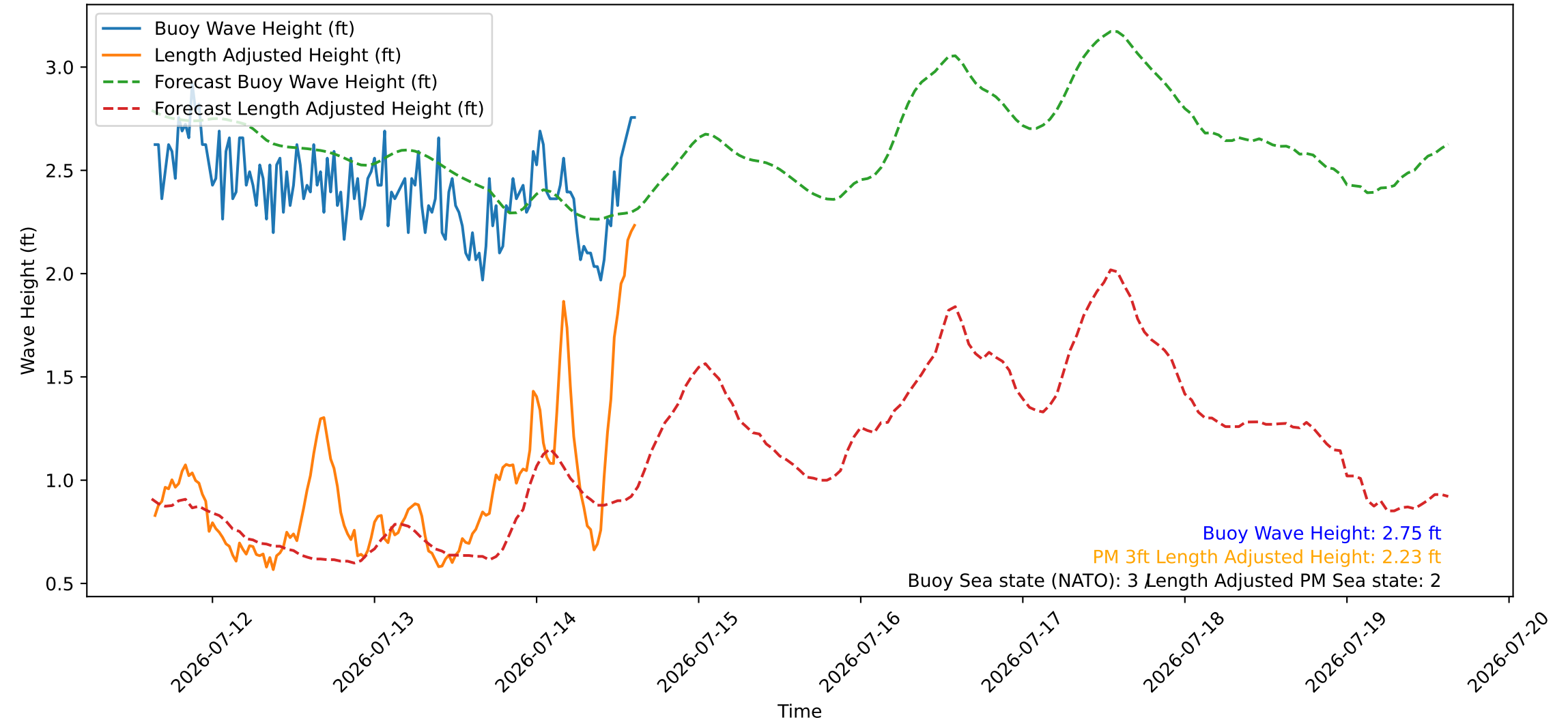
Wave Heights over Time for Red Beach at 2026-07-14 15:20:47
