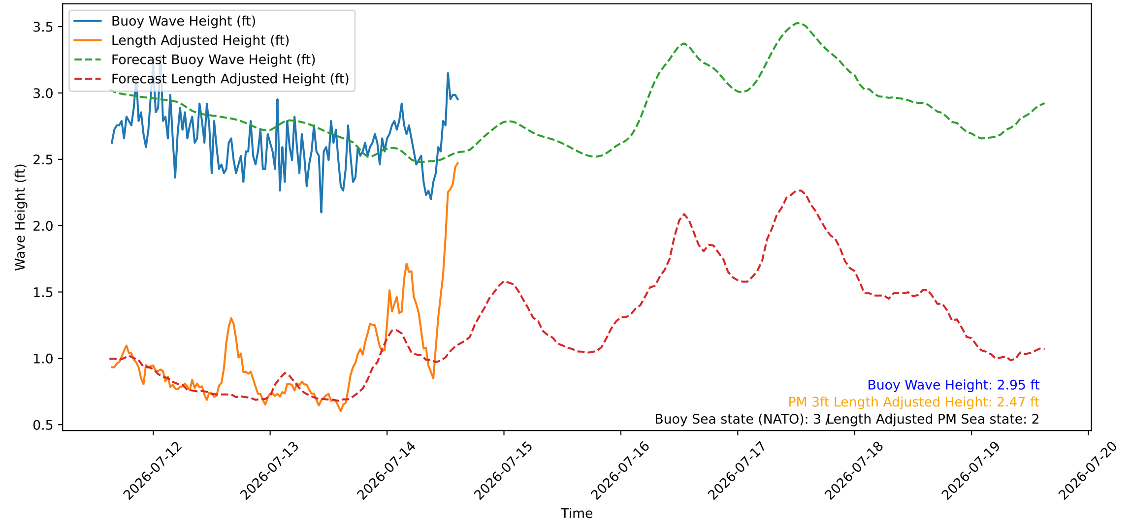
Wave Heights over Time for Oceanside Harbor at 2026-07-14 15:20:26
