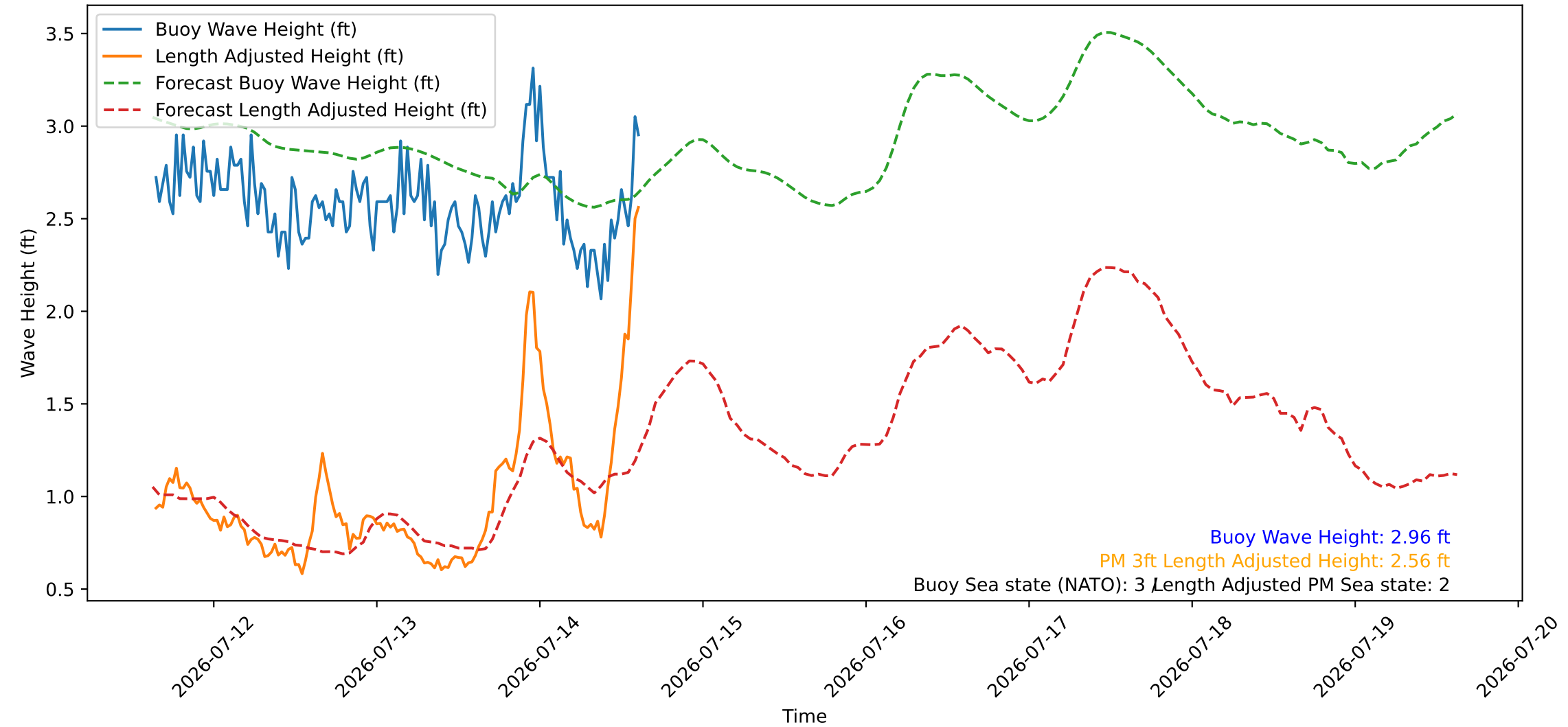
Wave Heights over Time for Green Beach at 2026-07-14 15:21:10
