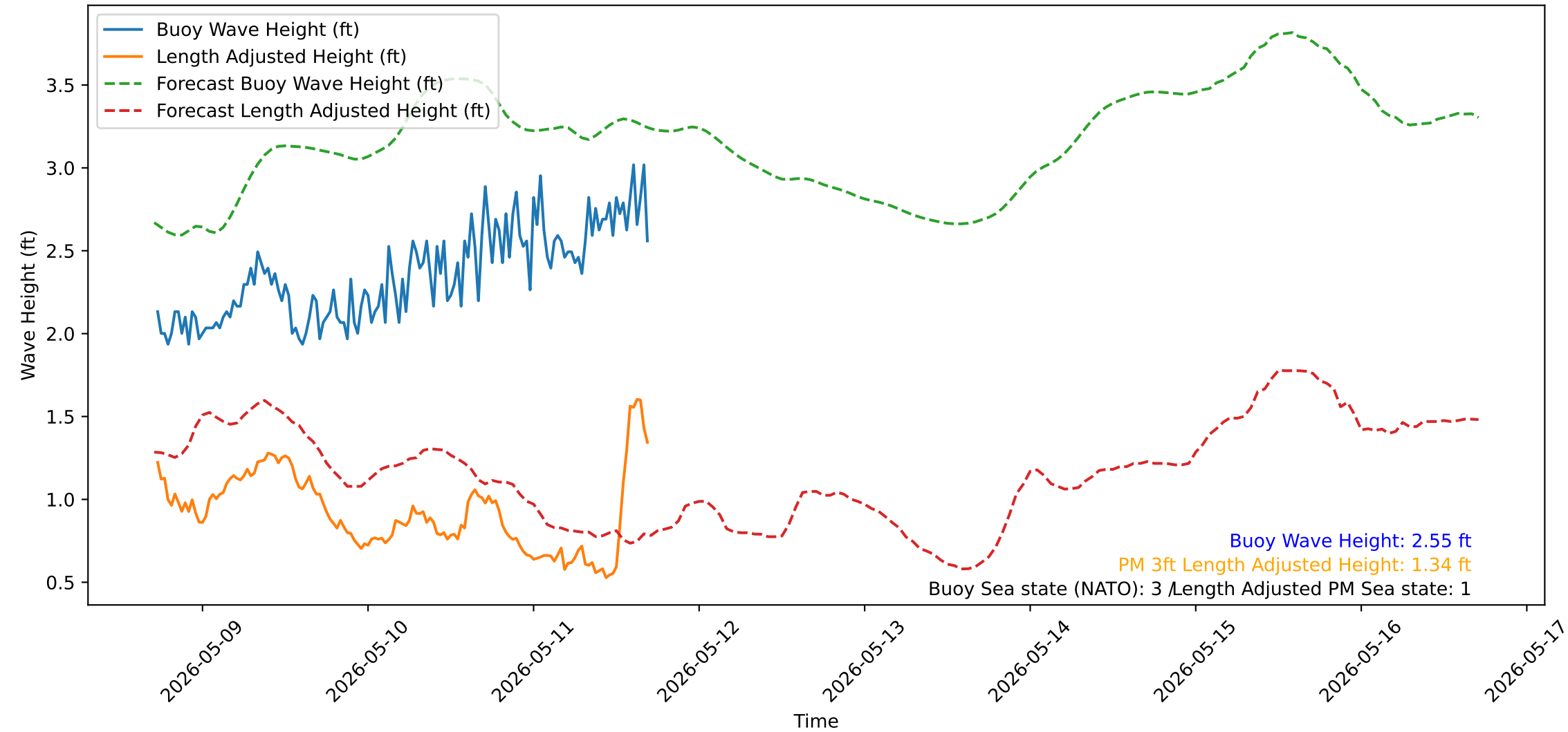
Wave Heights over Time for Red Beach at 2026-05-11 17:20:51
