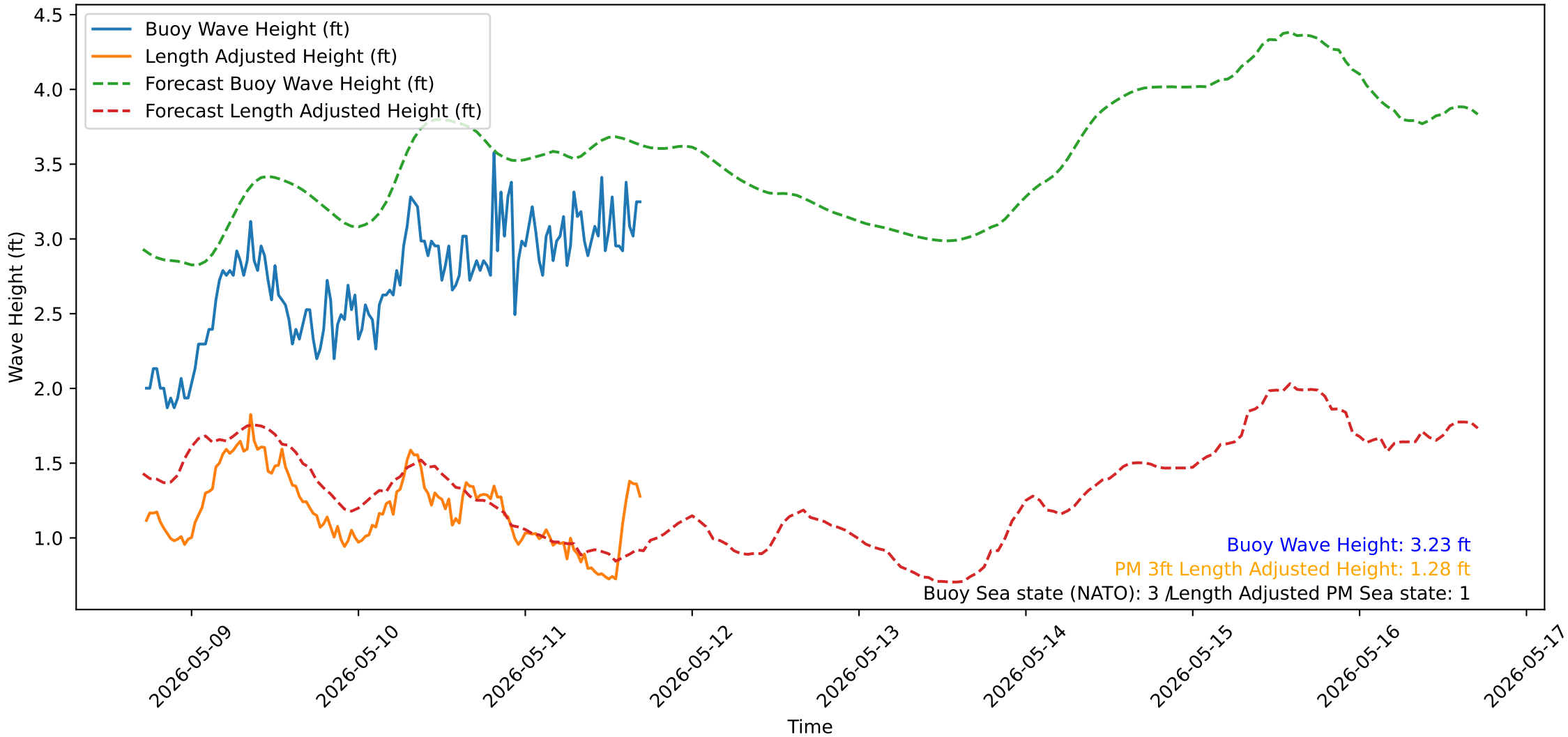
Wave Heights over Time for Oceanside Harbor at 2026-05-11 17:20:31
