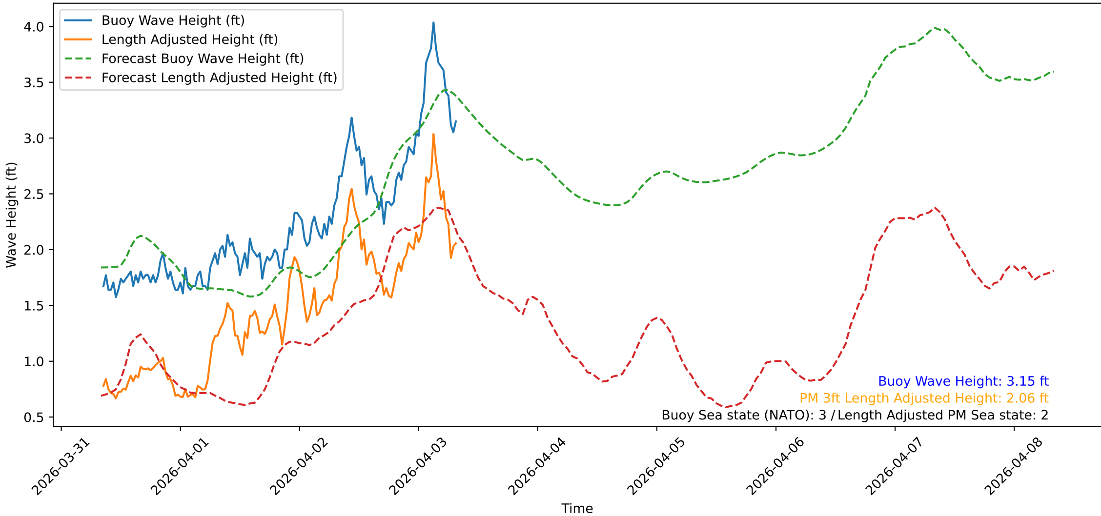
Wave Heights over Time for Oceanside Harbor at 2026-04-03 08:20:32
