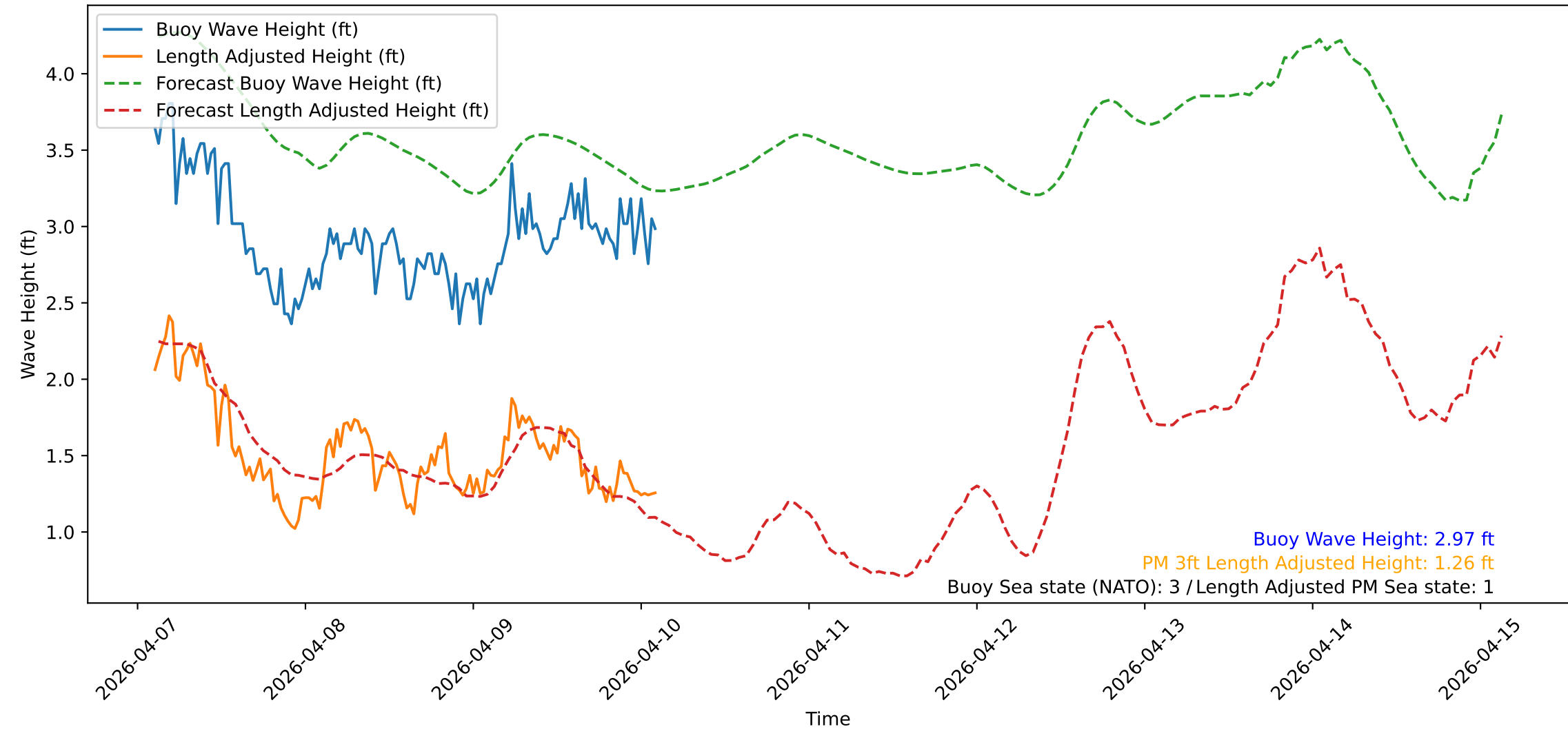
Wave Heights over Time for Green Beach at 2026-04-10 02:41:13
