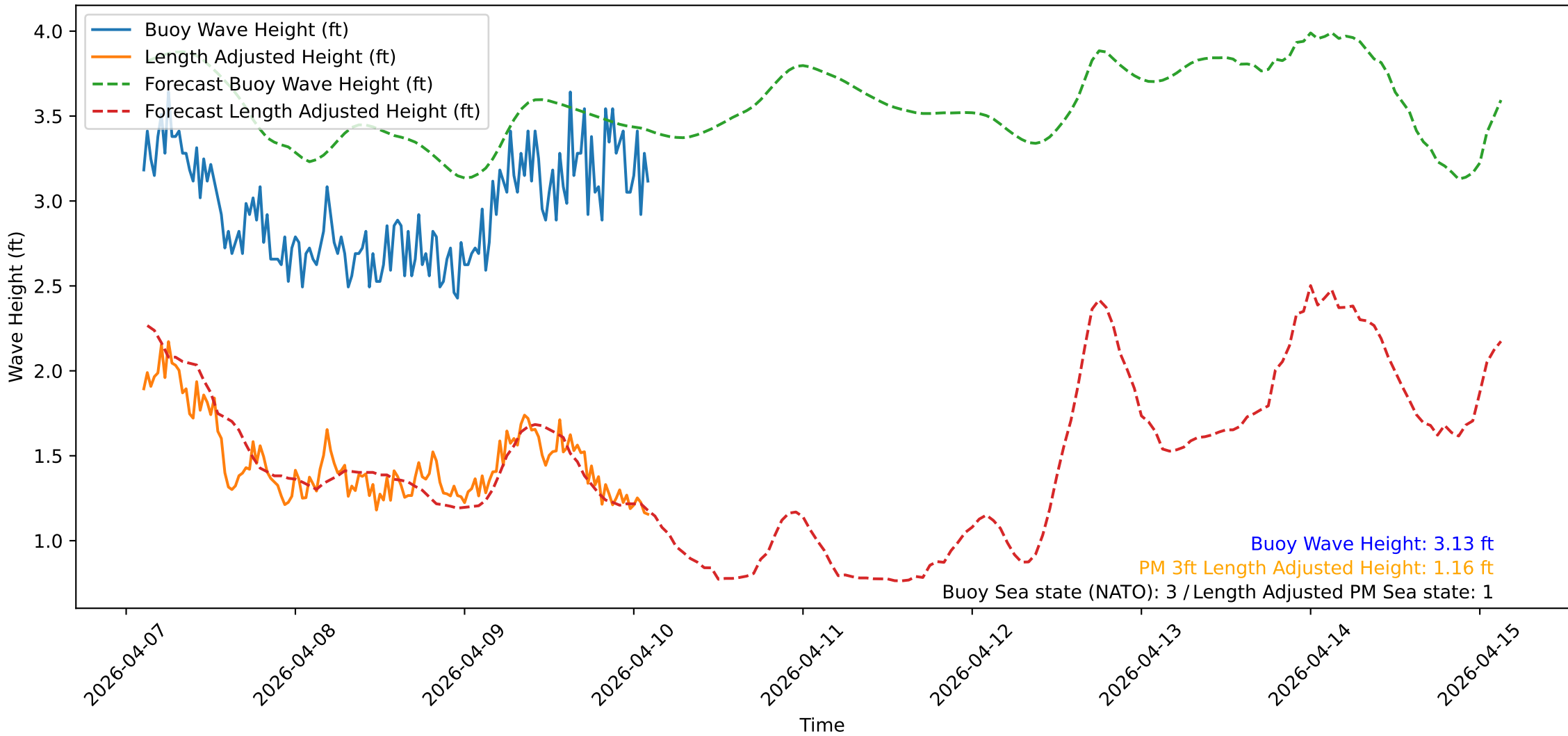
Wave Heights over Time for Oceanside Harbor at 2026-04-10 02:40:31
