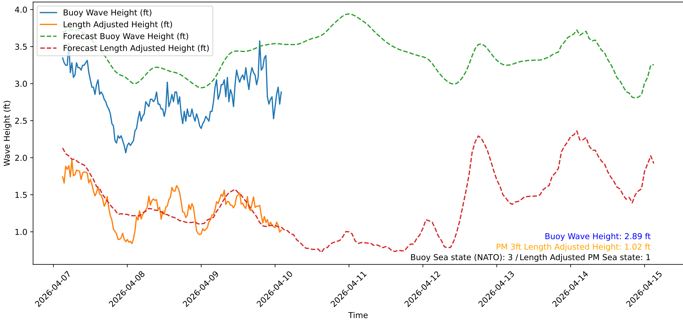
Wave Heights over Time for Red Beach at 2026-04-10 02:40:51
