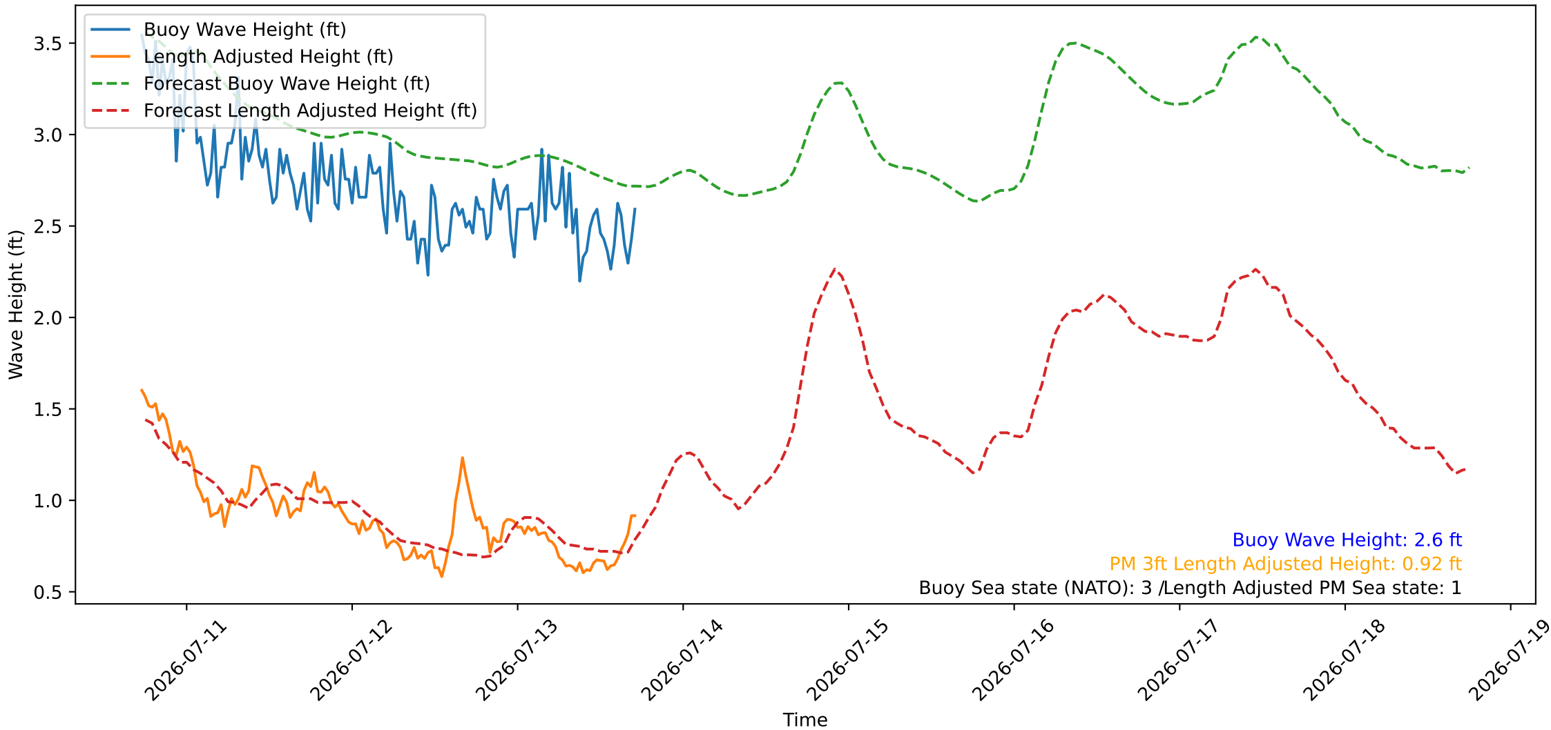
Wave Heights over Time for Green Beach at 2026-07-13 17:41:09
