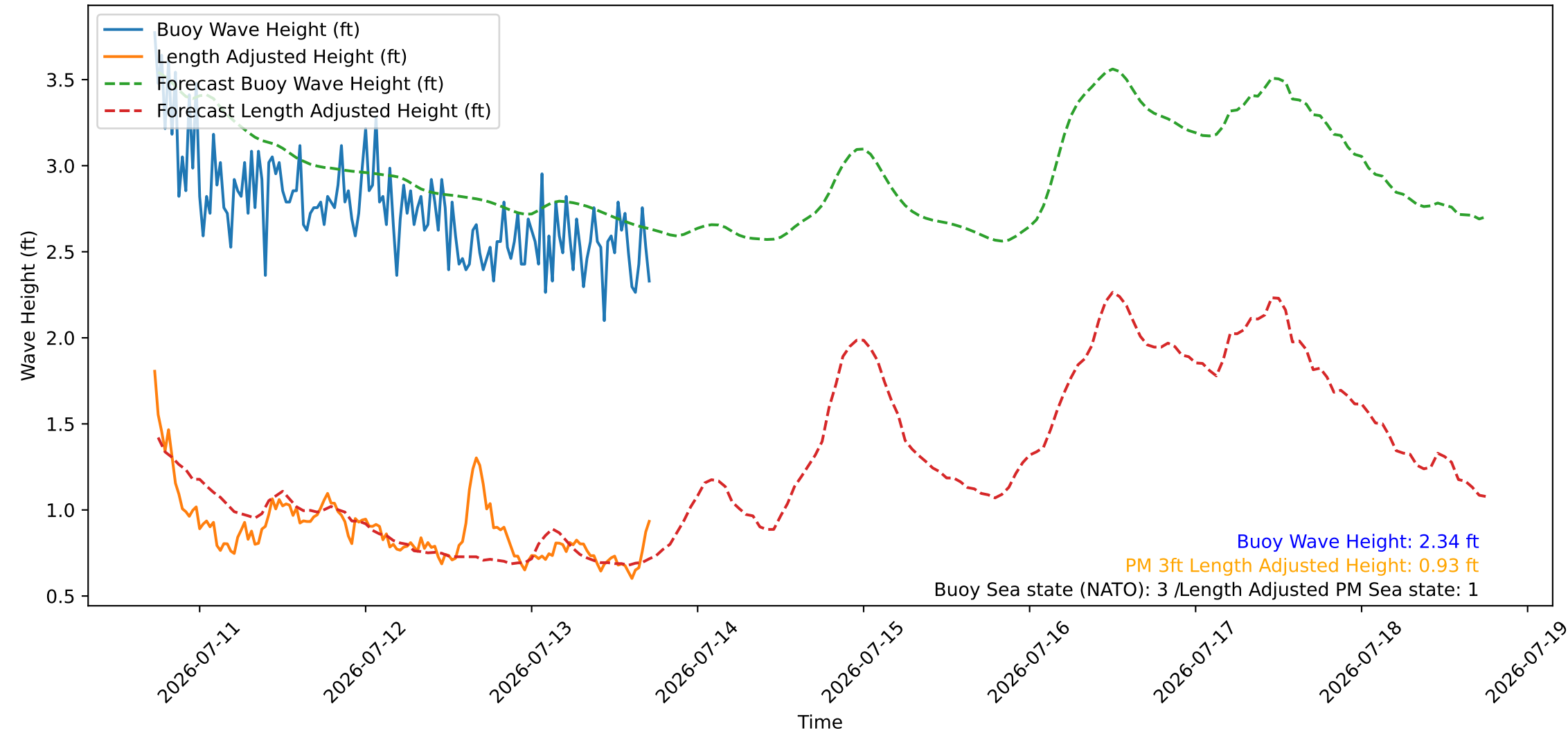
Wave Heights over Time for Oceanside Harbor at 2026-07-13 17:40:26
