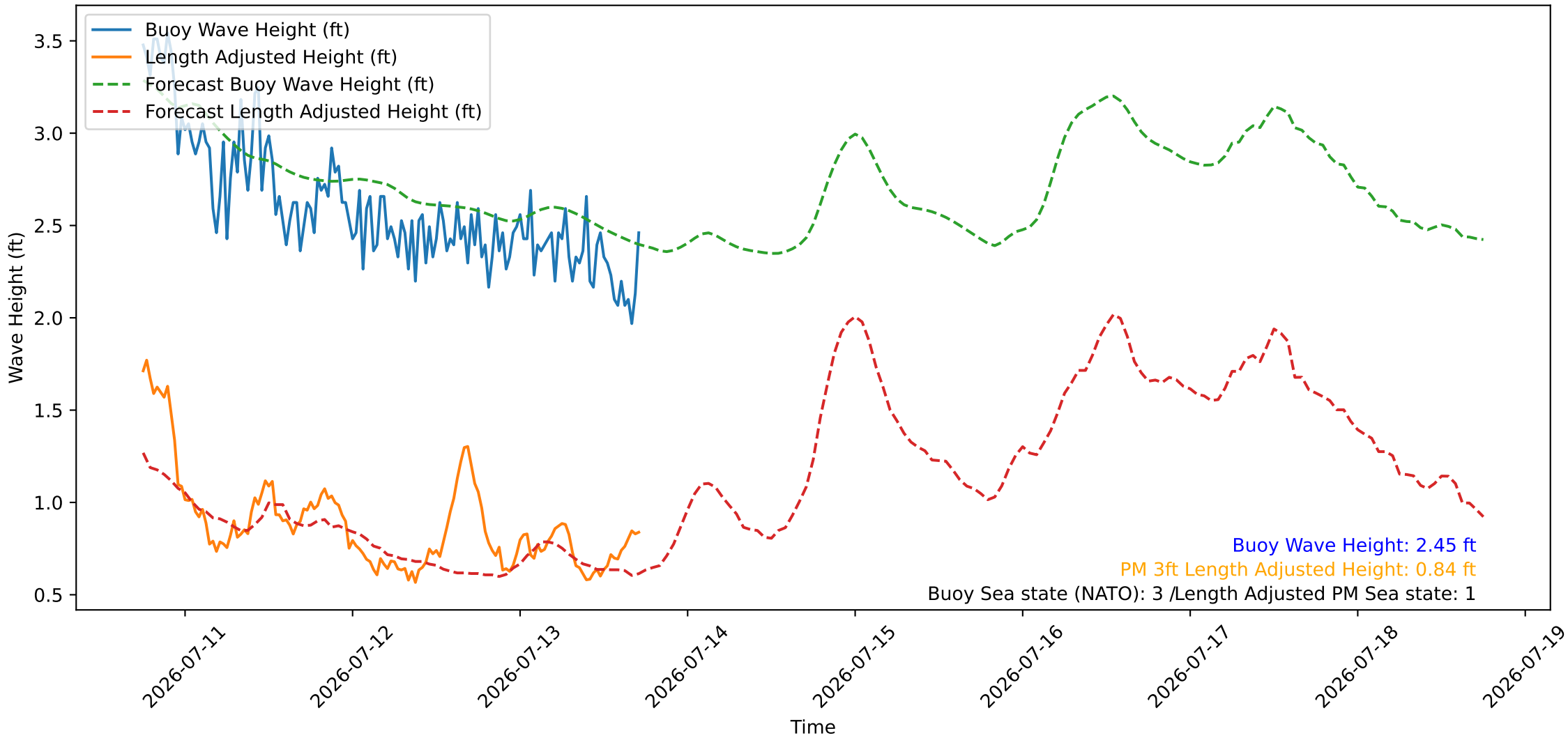
Wave Heights over Time for Red Beach at 2026-07-13 17:40:46
