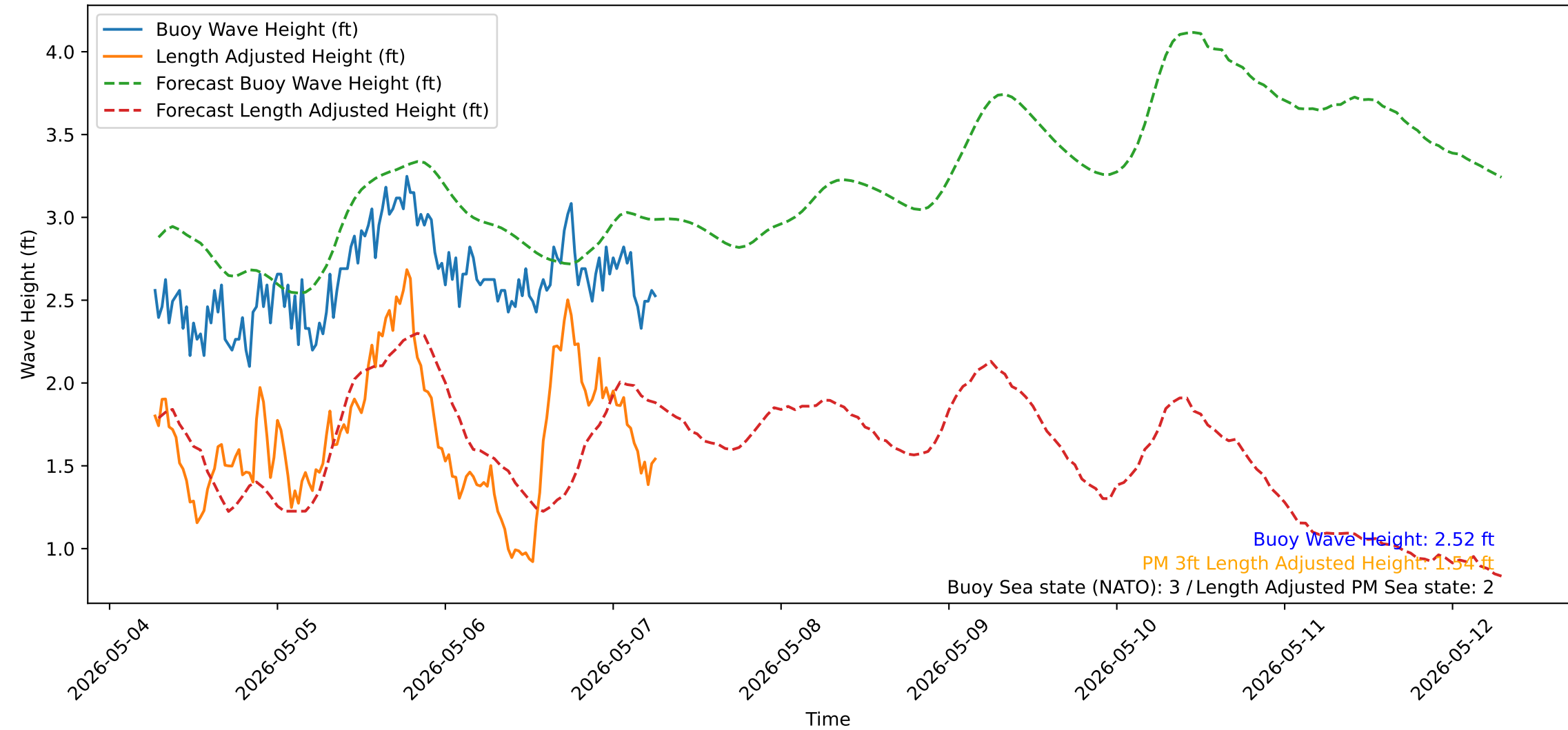
Wave Heights over Time for Oceanside Harbor at 2026-05-07 06:40:31
