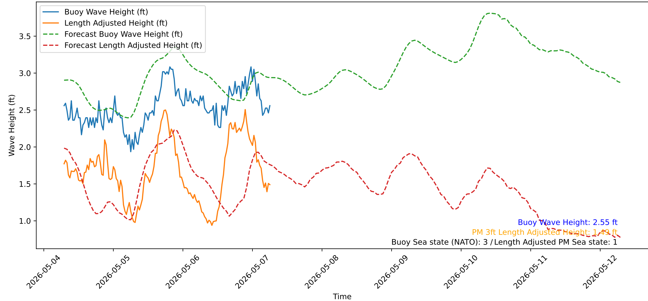
Wave Heights over Time for Red Beach at 2026-05-07 06:40:50
