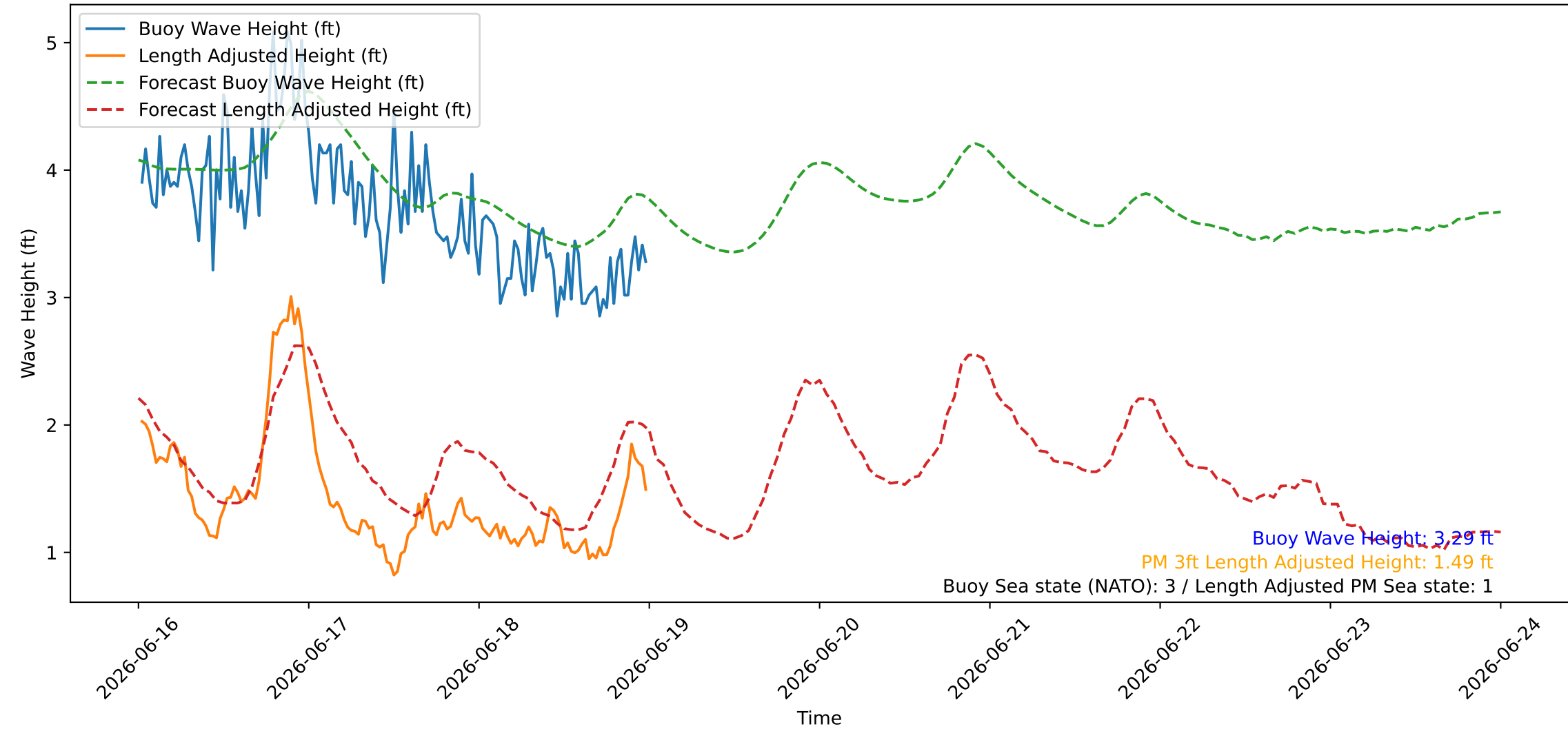
Wave Heights over Time for Green Beach at 2026-06-19 00:21:09
