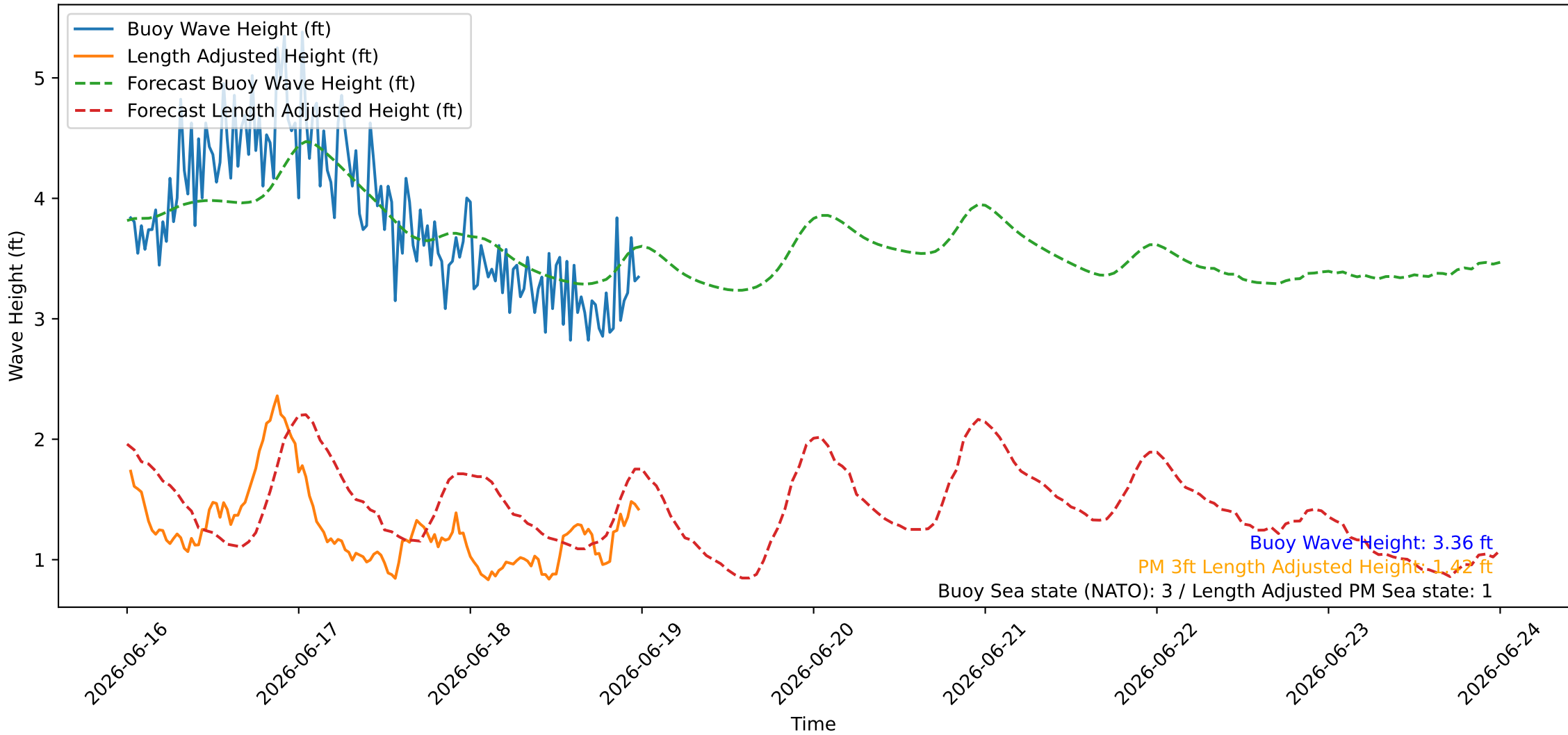
Wave Heights over Time for Red Beach at 2026-06-19 00:20:47
