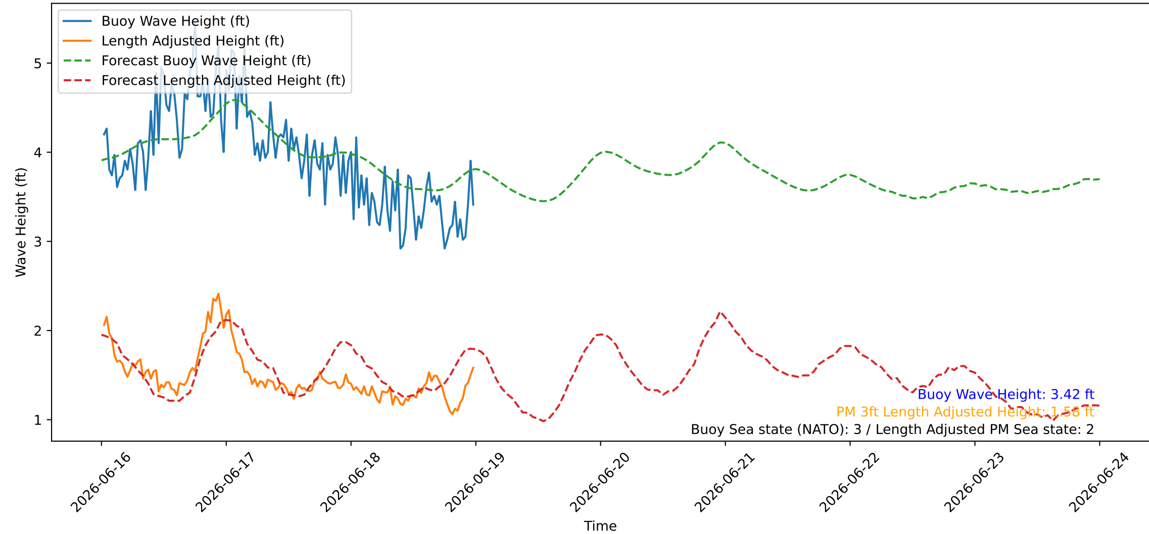
Wave Heights over Time for Oceanside Harbor at 2026-06-19 00:20:26
