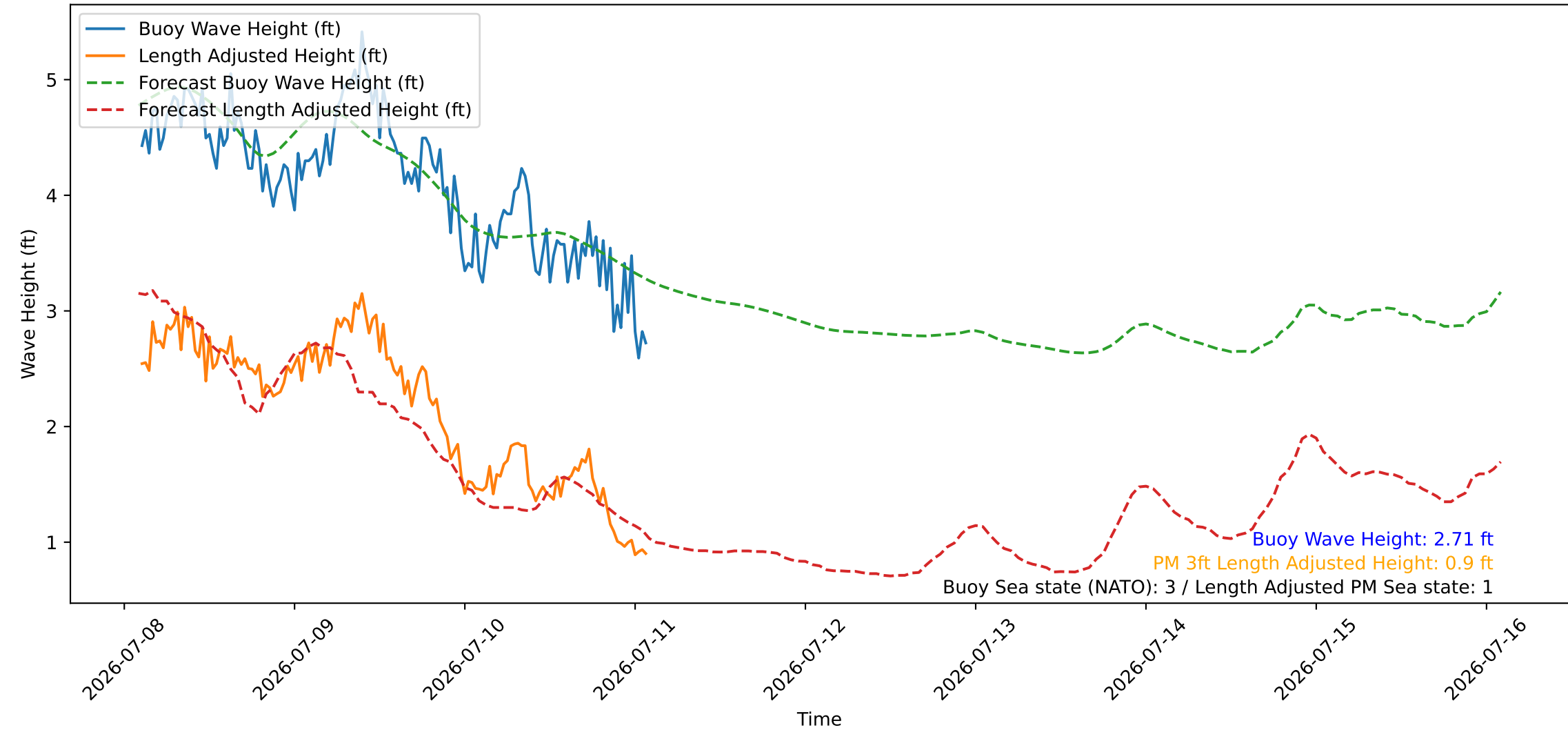
Wave Heights over Time for Oceanside Harbor at 2026-07-11 02:20:26
