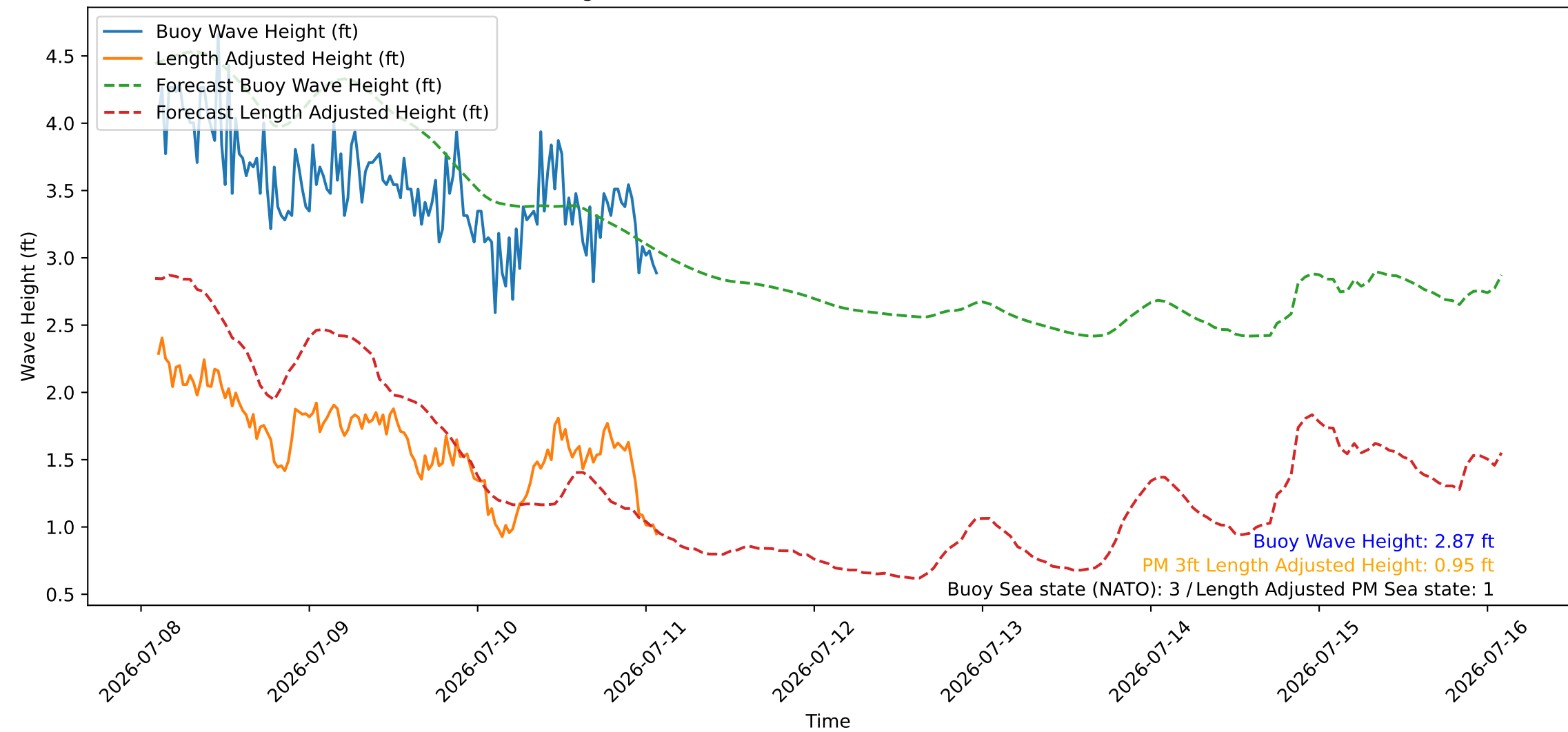
Wave Heights over Time for Red Beach at 2026-07-11 02:20:46
