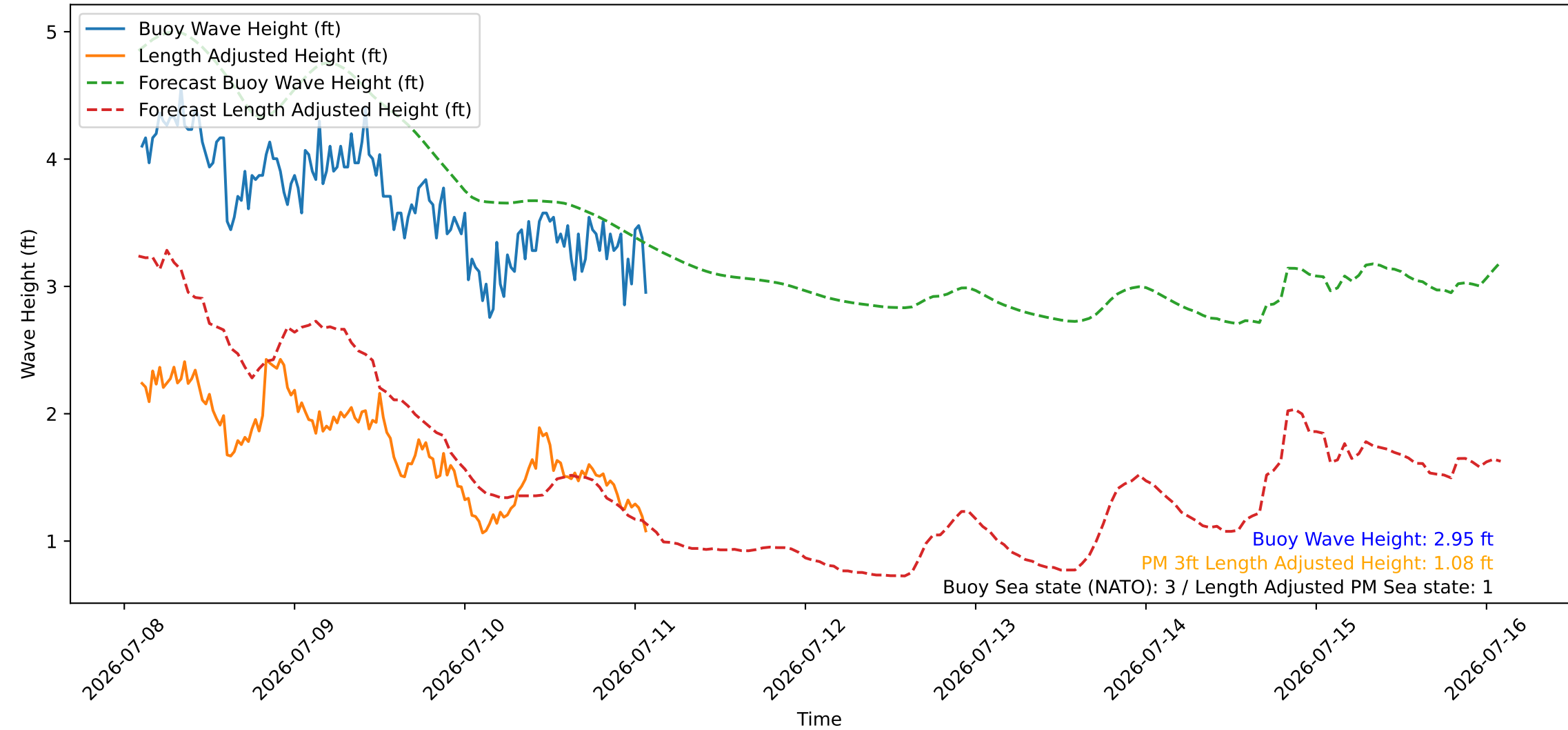
Wave Heights over Time for Green Beach at 2026-07-11 02:21:08
