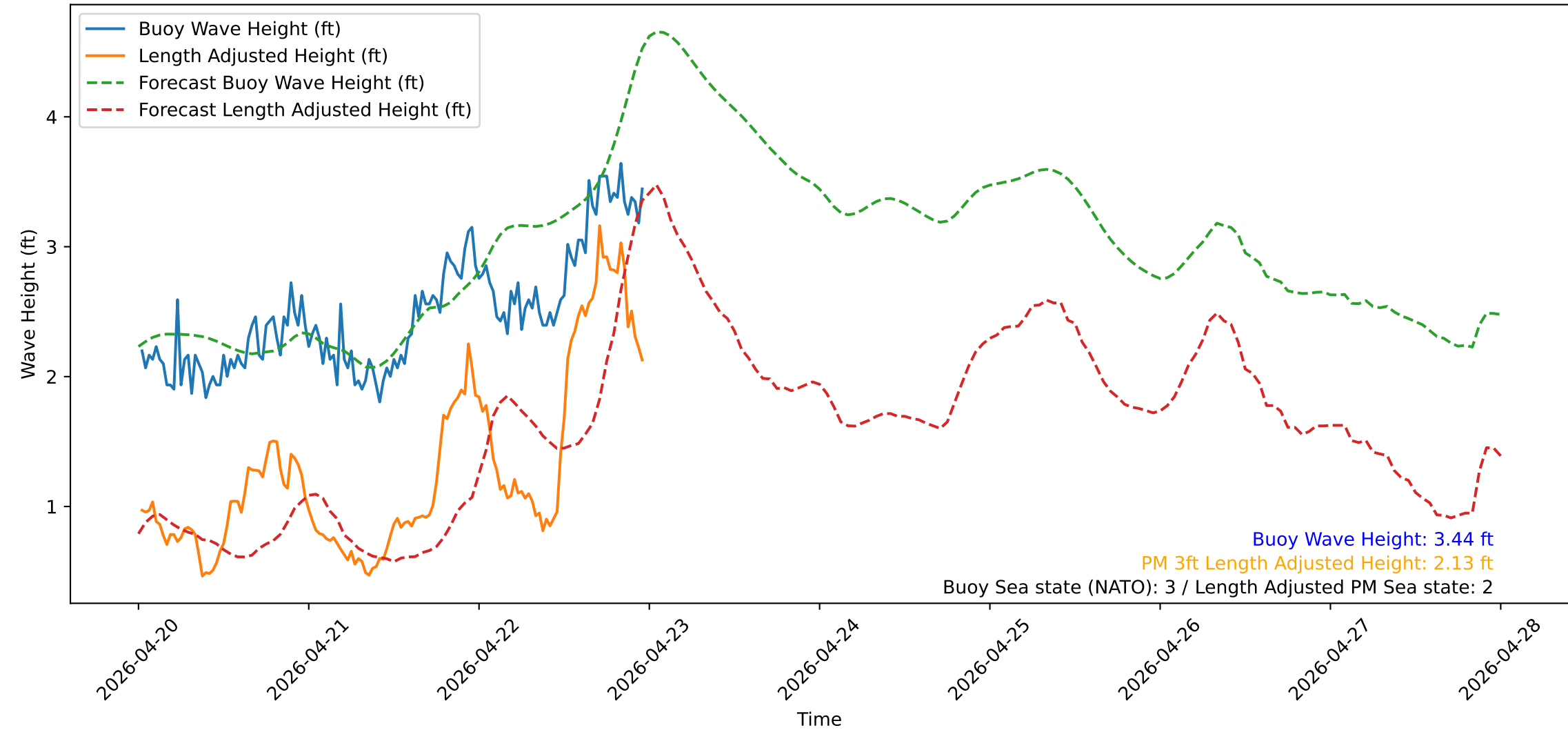
Wave Heights over Time for Red Beach at 2026-04-23 00:00:50
