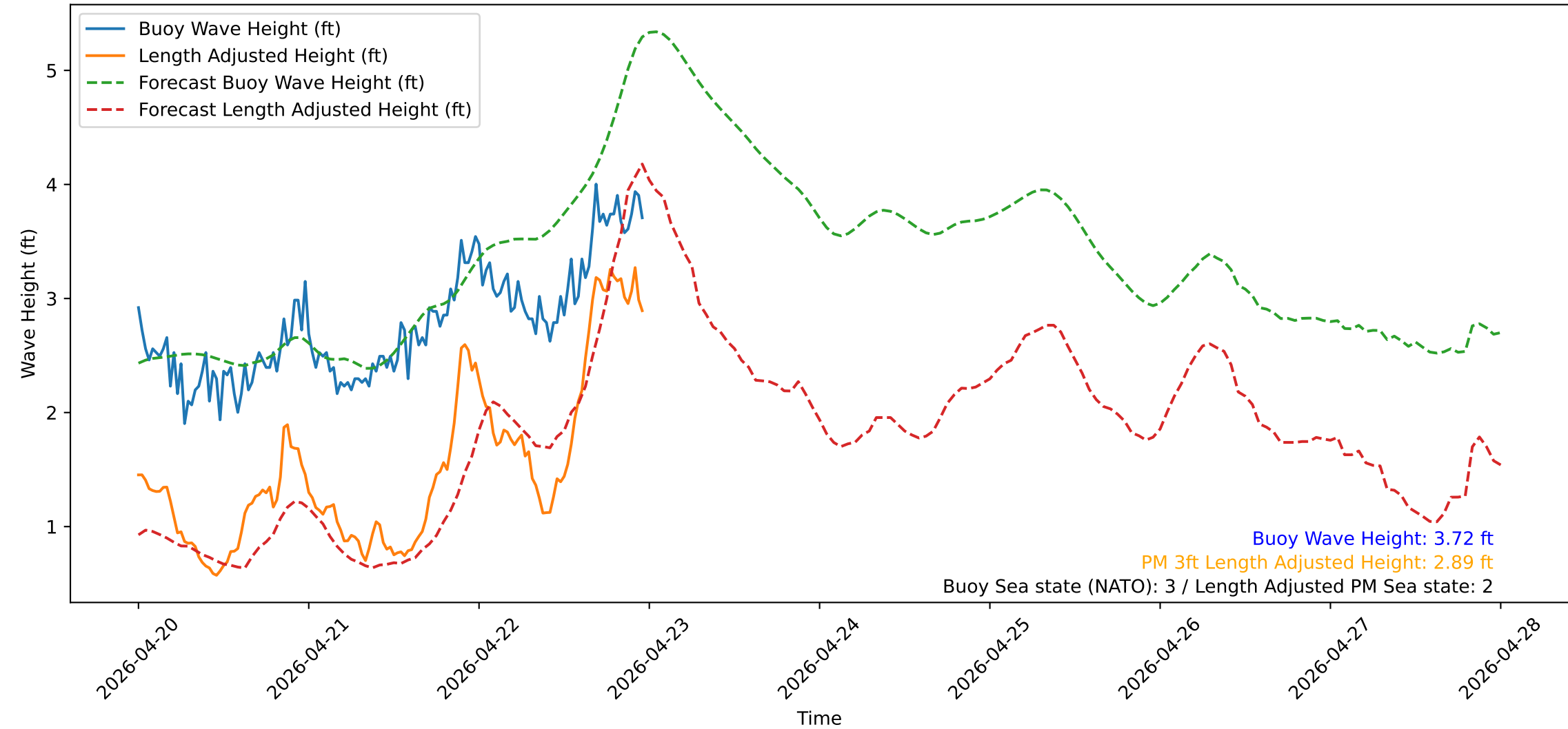
Wave Heights over Time for Green Beach at 2026-04-23 00:01:12
