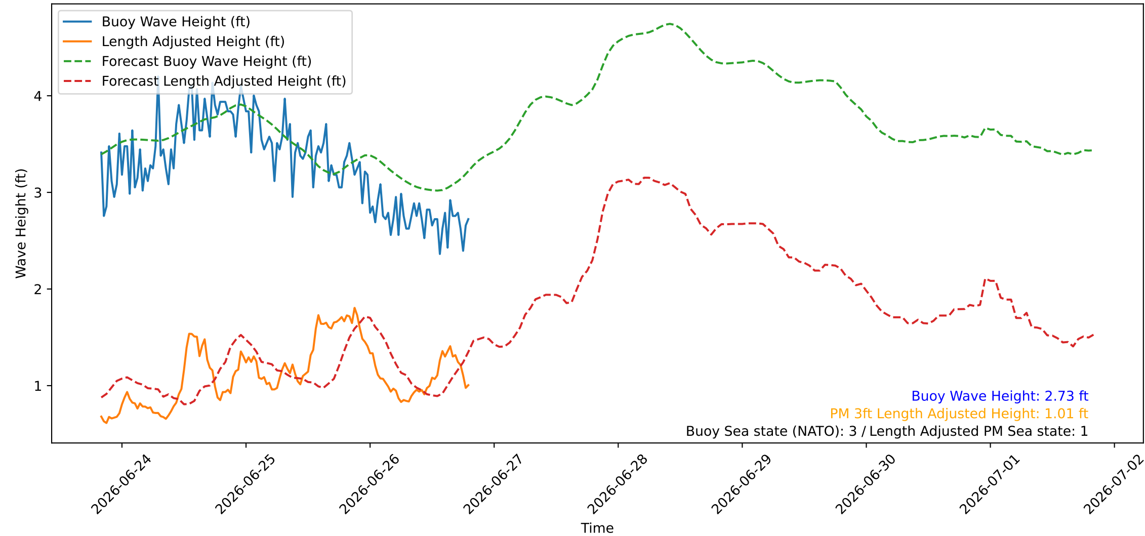
Wave Heights over Time for Green Beach at 2026-06-26 20:01:07
