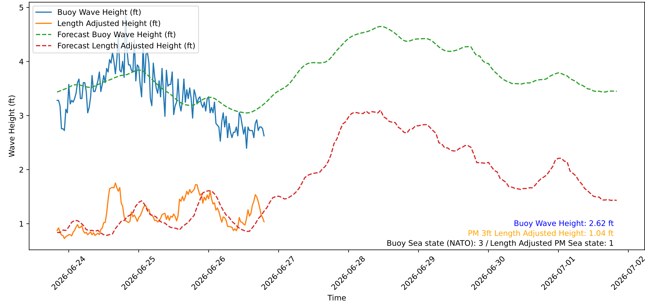
Wave Heights over Time for Oceanside Harbor at 2026-06-26 20:00:26
