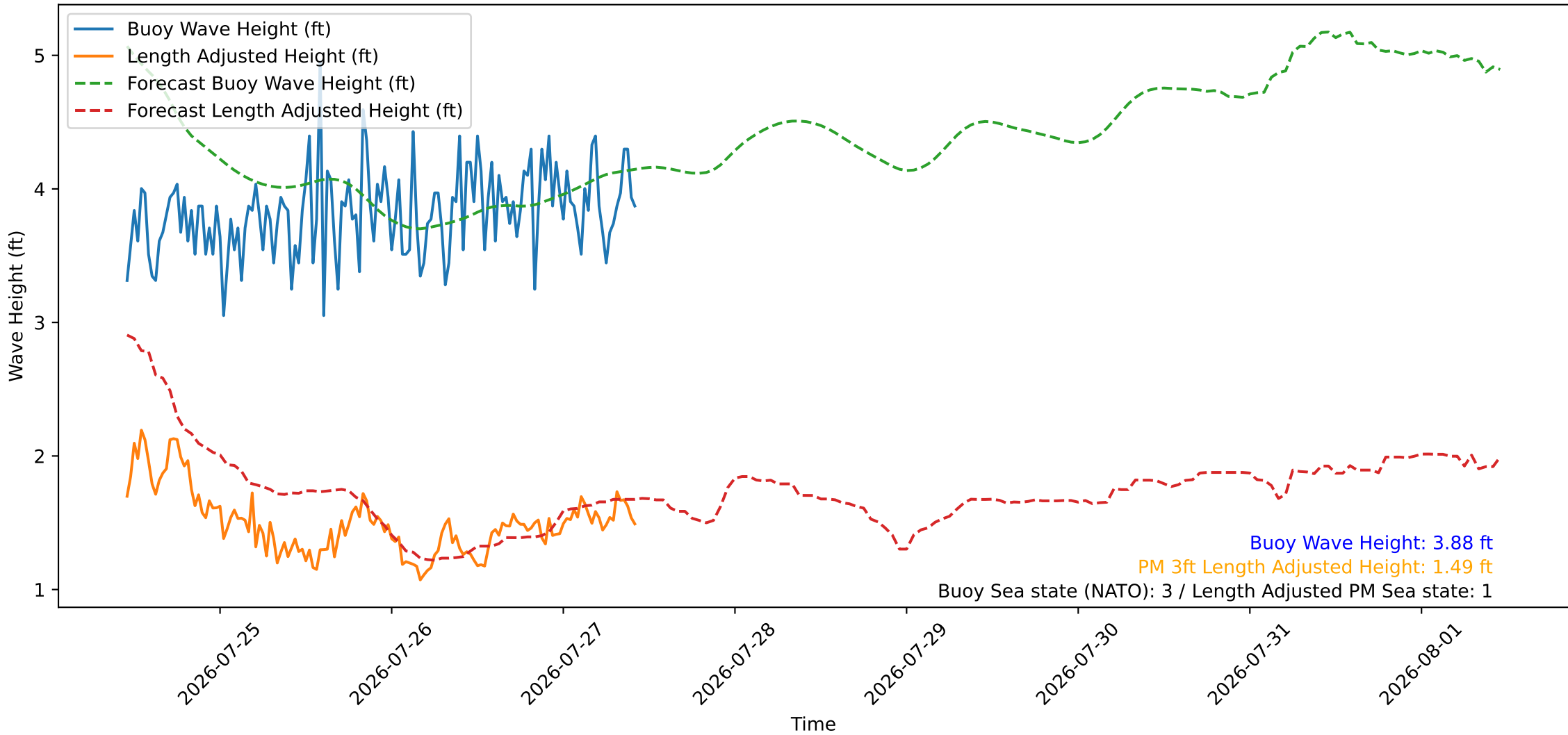
Wave Heights over Time for Oceanside Harbor at 2026-07-27 11:00:26
