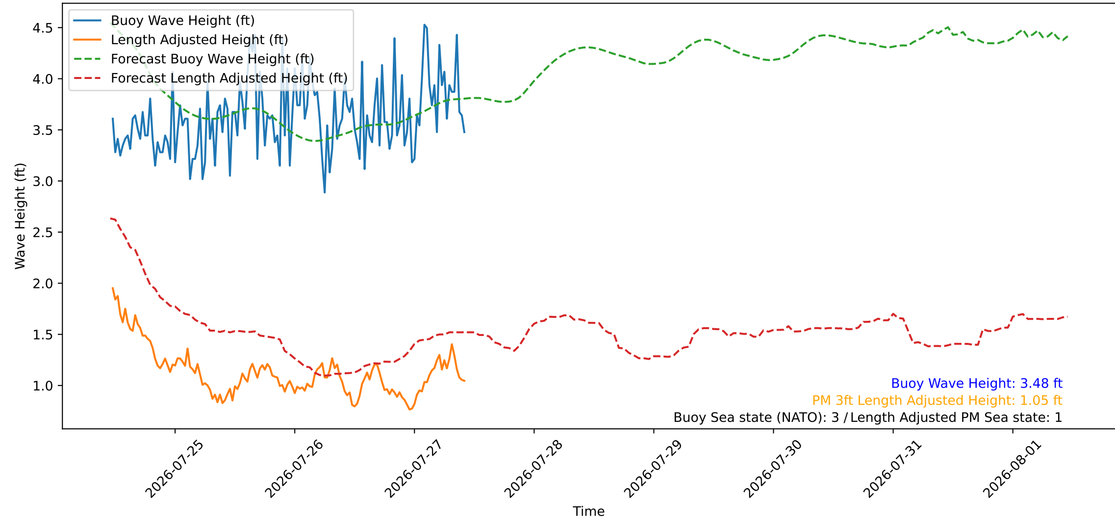
Wave Heights over Time for Red Beach at 2026-07-27 11:00:45
