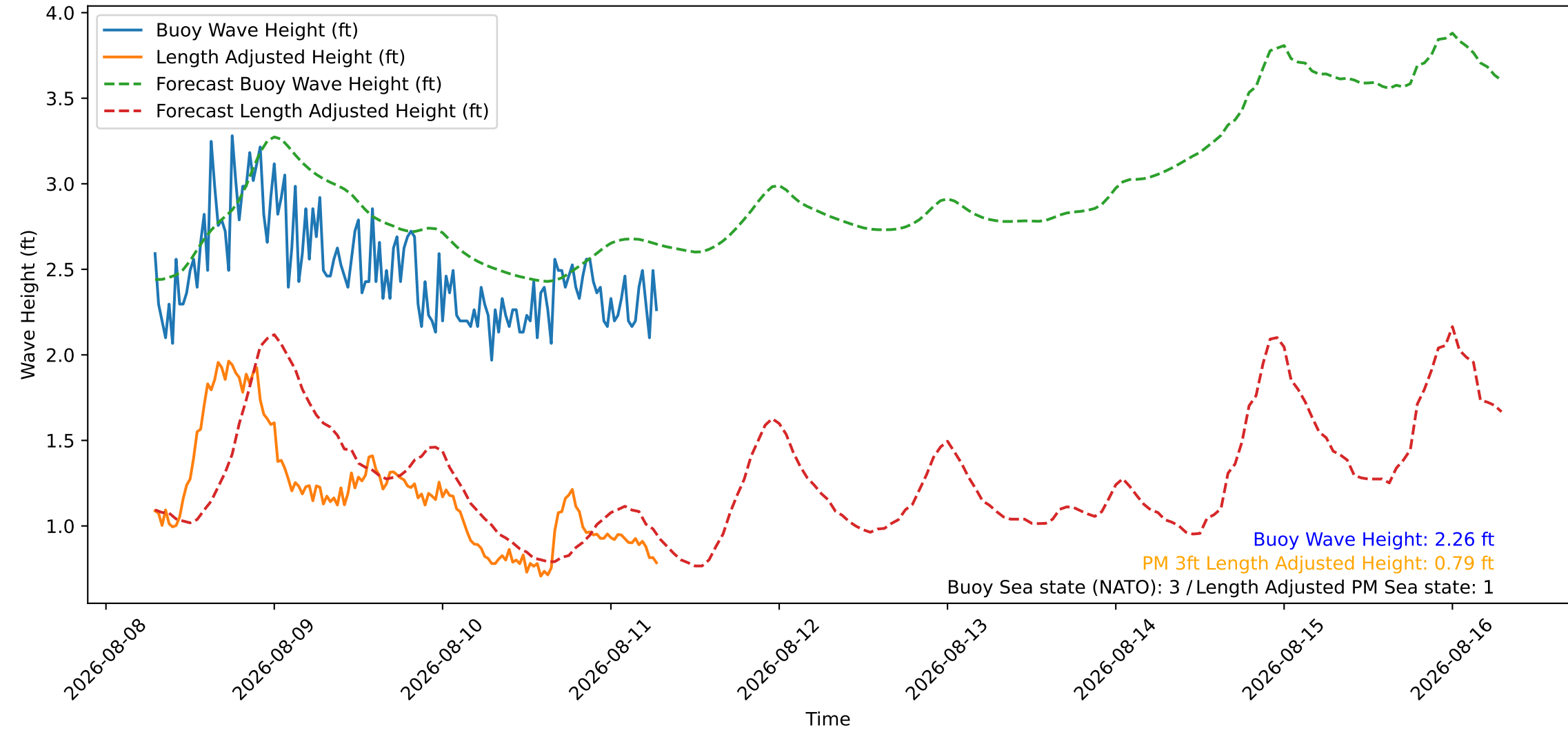
Wave Heights over Time for Oceanside Harbor at 2026-08-11 07:10:26
