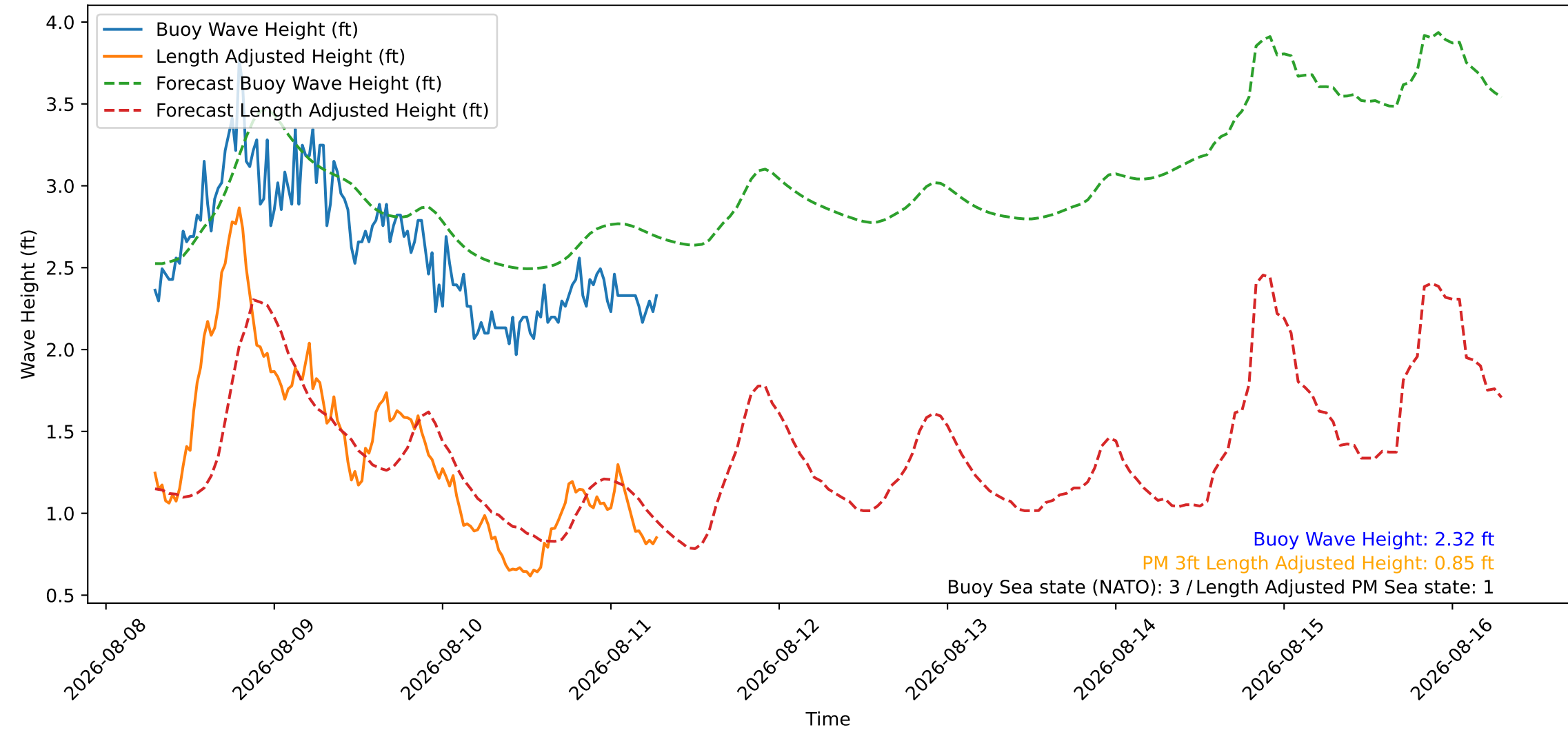
Wave Heights over Time for Green Beach at 2026-08-11 07:11:09
