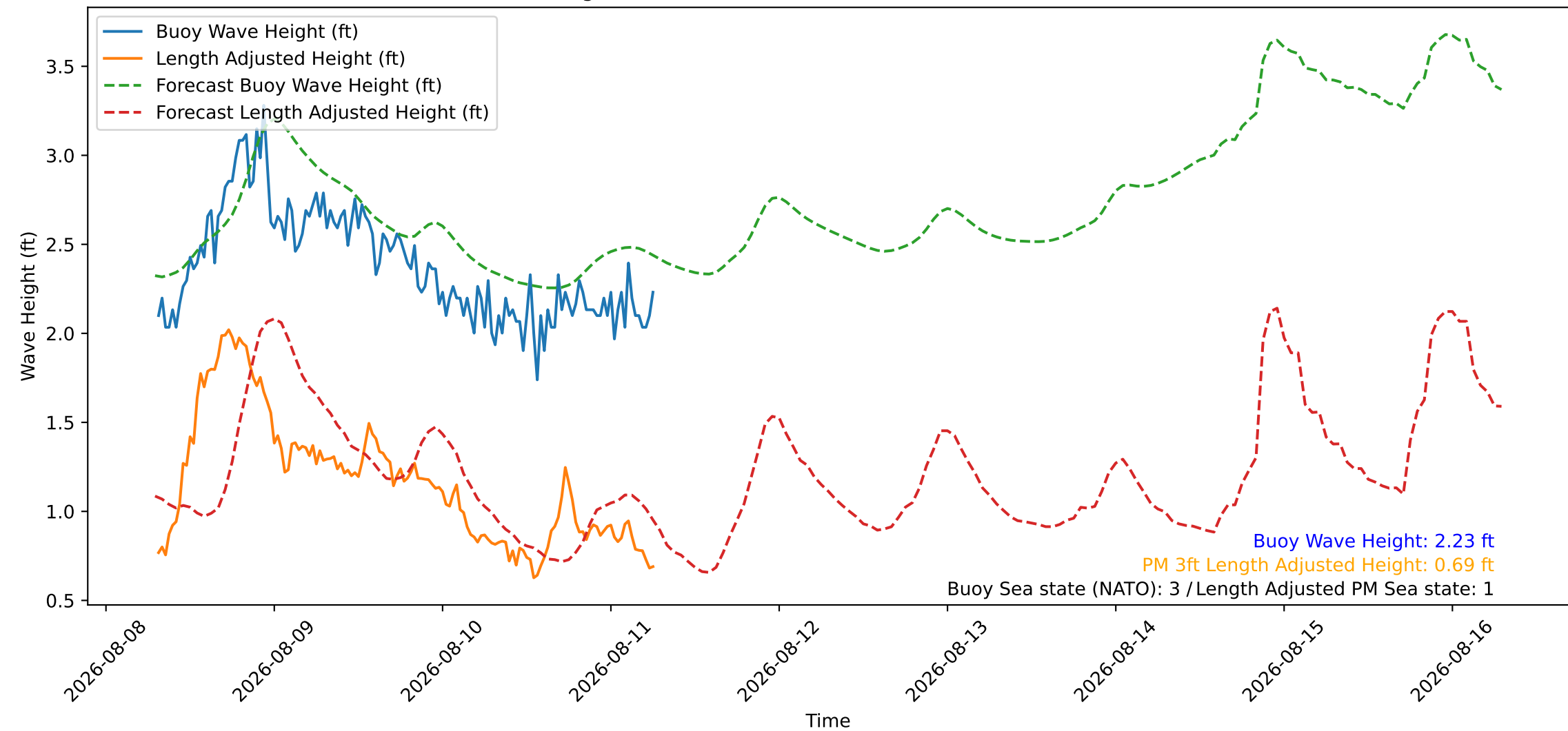
Wave Heights over Time for Red Beach at 2026-08-11 07:10:46
