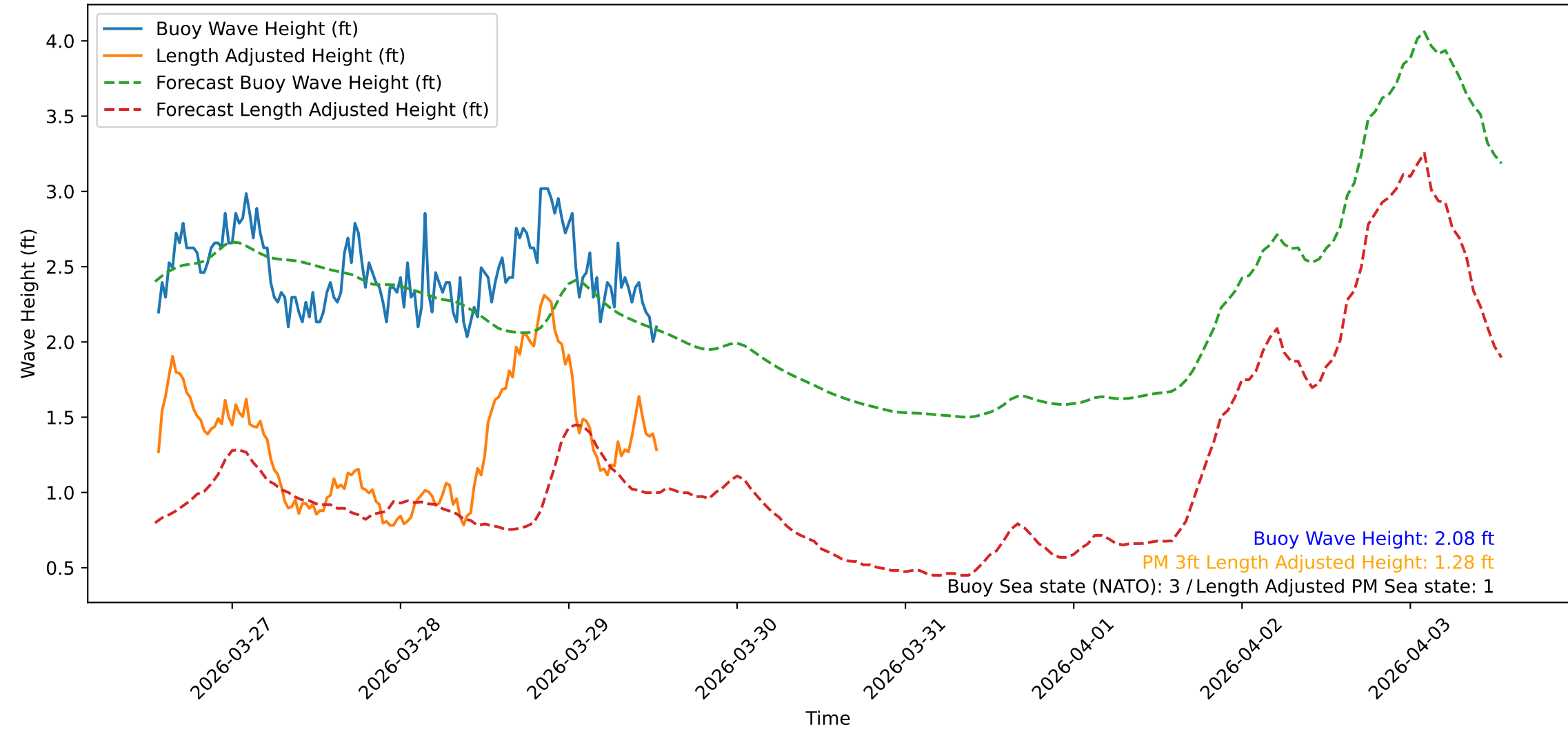
Wave Heights over Time for Red Beach at 2026-03-29 13:10:48
