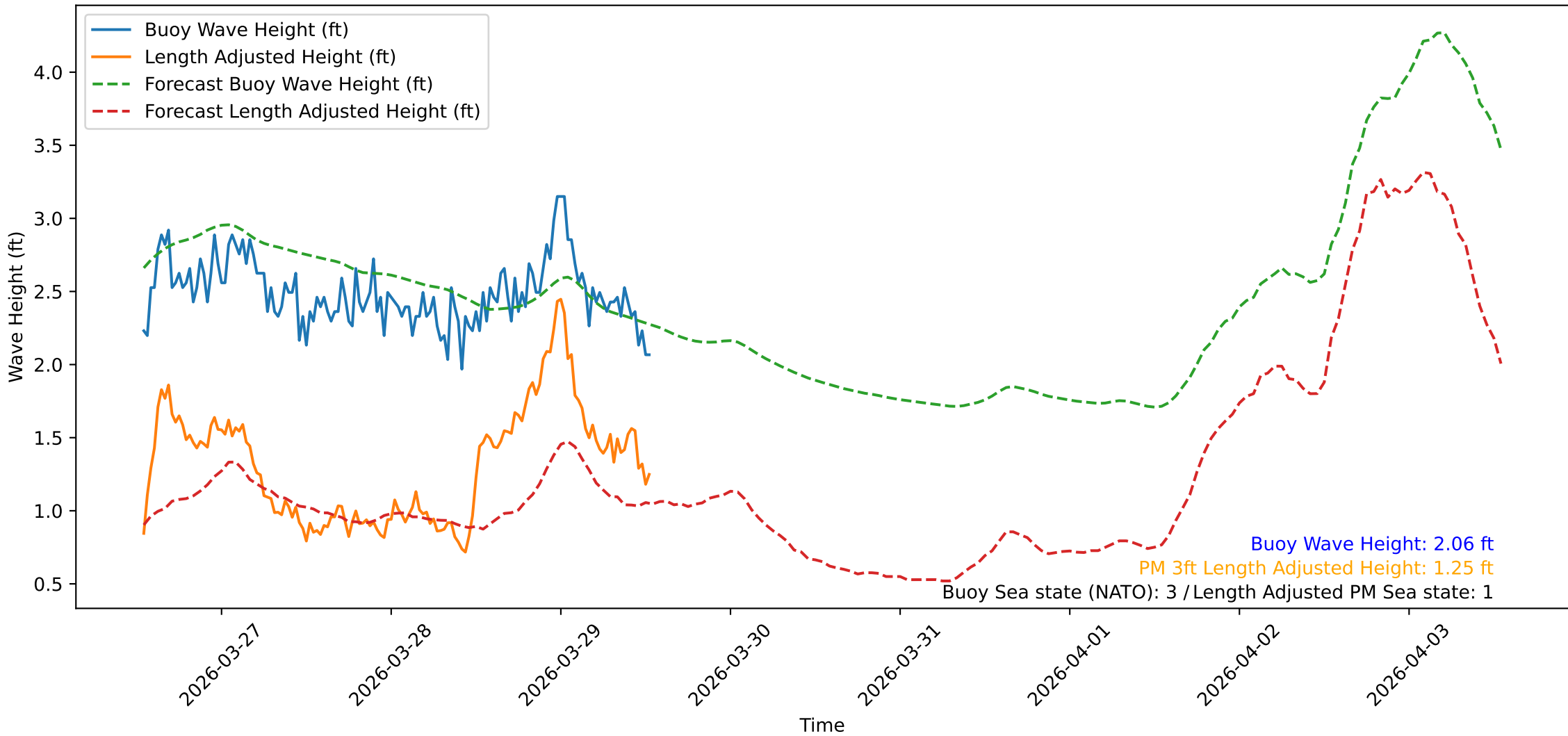
Wave Heights over Time for Oceanside Harbor at 2026-03-29 13:10:32
