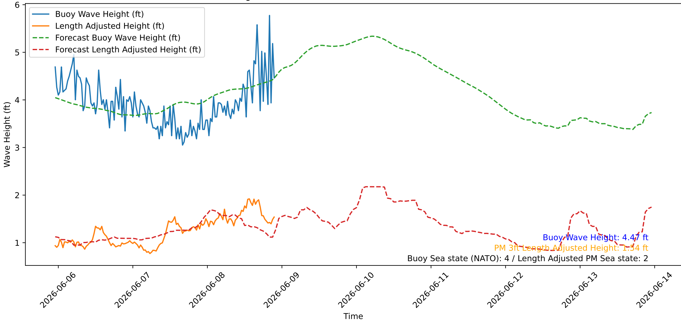
Wave Heights over Time for Red Beach at 2026-06-08 22:30:46
