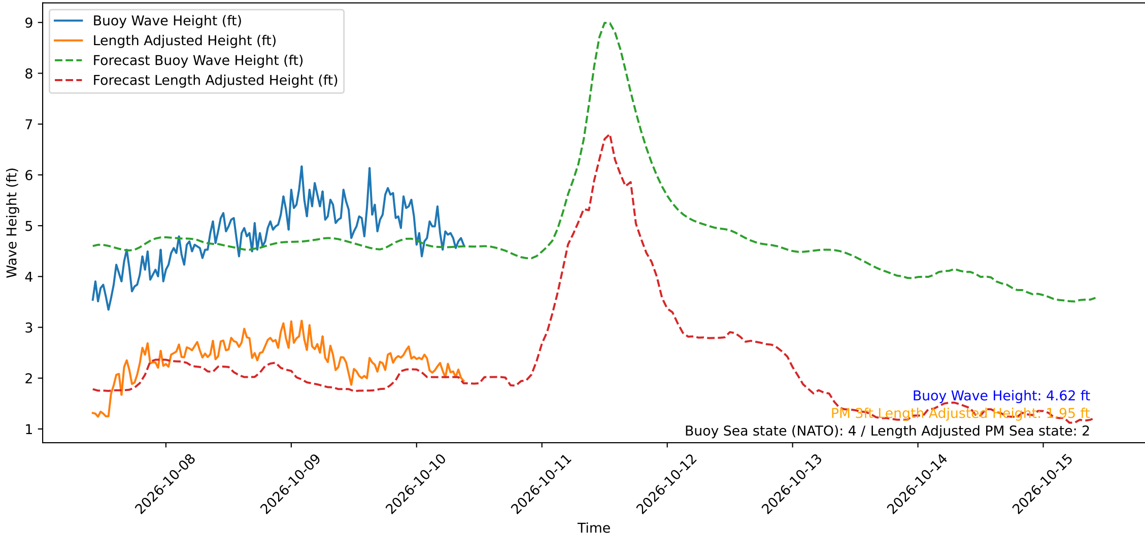
Wave Heights over Time for Green Beach at 2026-10-10 09:41:12
