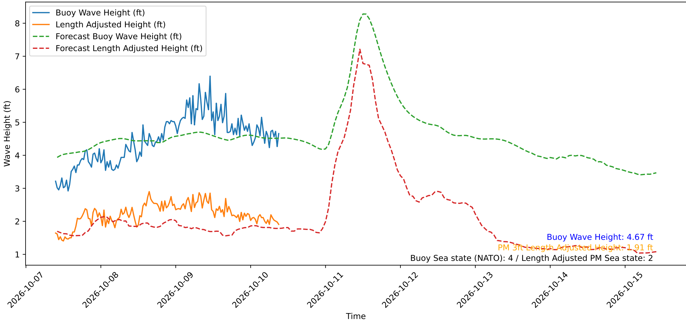
Wave Heights over Time for Oceanside Harbor at 2026-10-10 09:40:30
