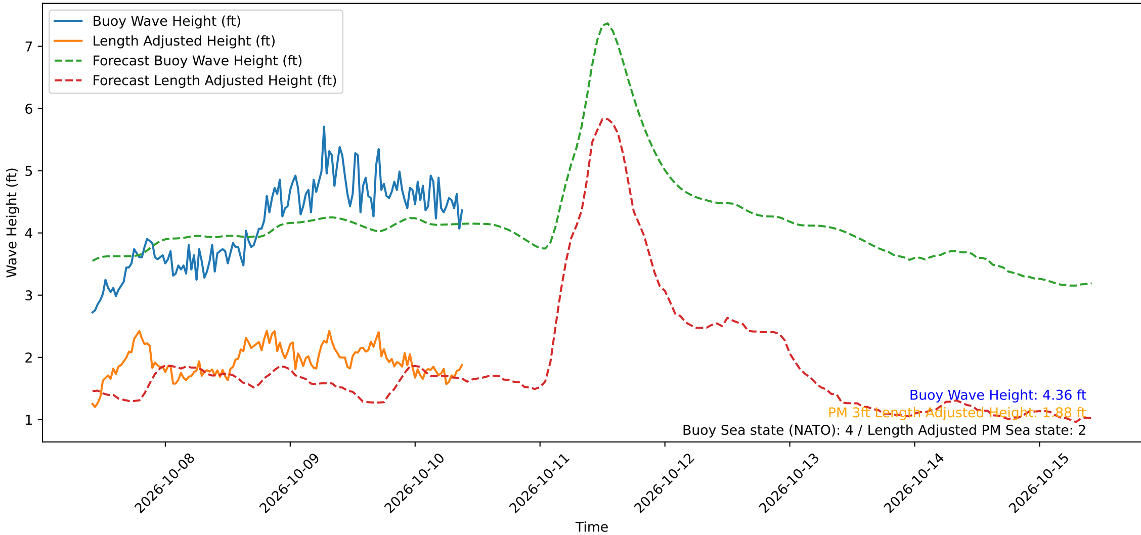
Wave Heights over Time for Red Beach at 2026-10-10 09:40:50
