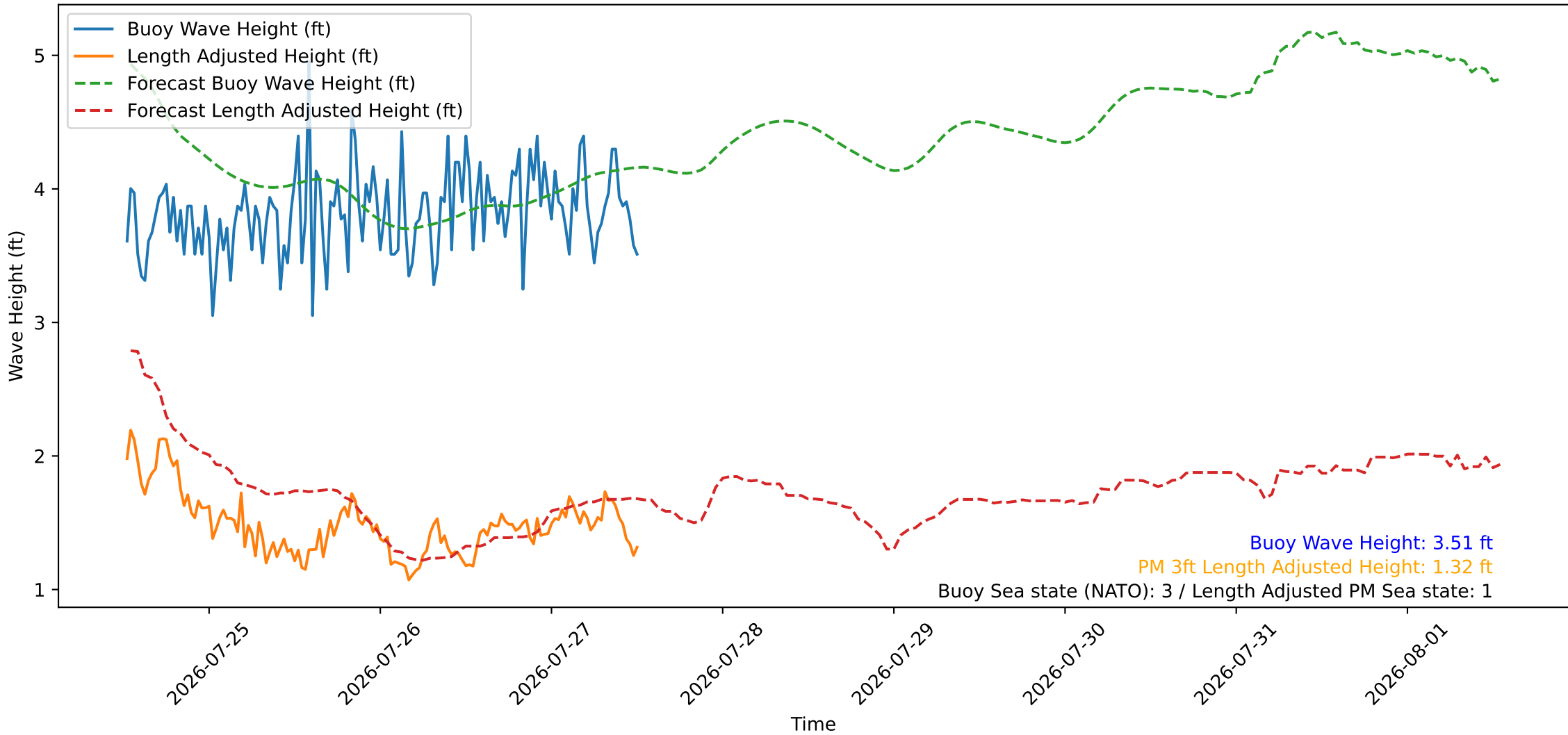
Wave Heights over Time for Oceanside Harbor at 2026-07-27 12:30:26
