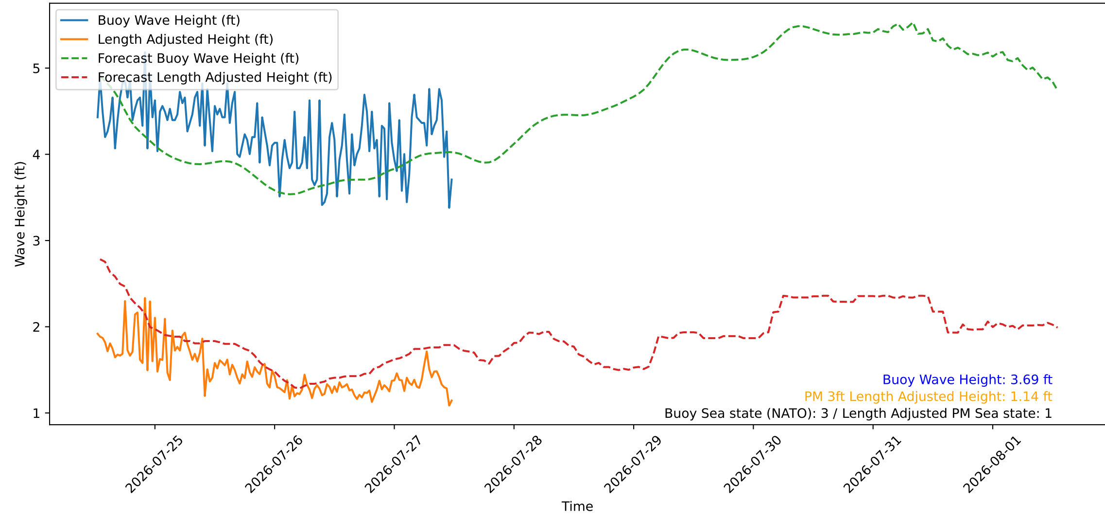
Wave Heights over Time for Green Beach at 2026-07-27 12:31:09
