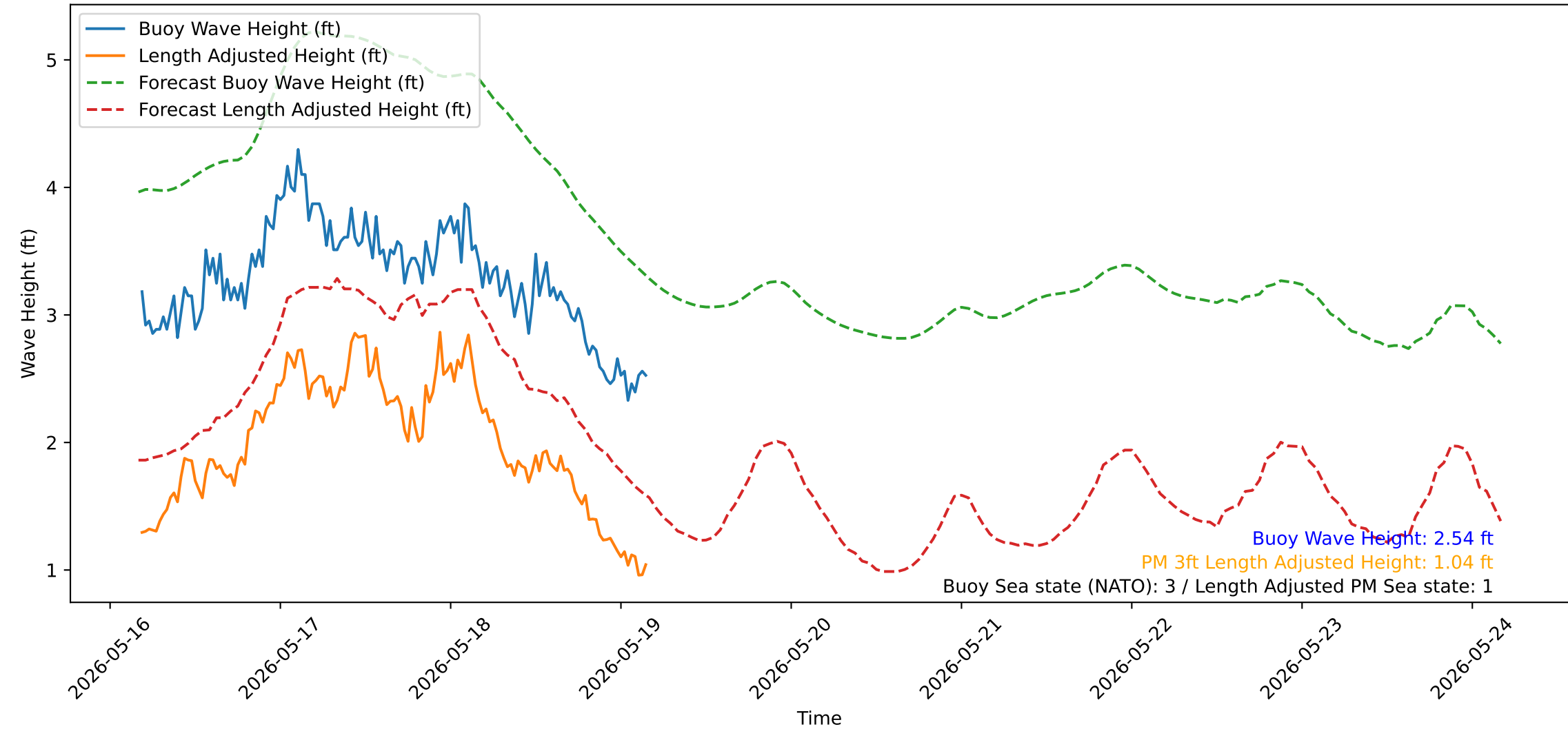
Wave Heights over Time for Oceanside Harbor at 2026-05-19 04:20:32
