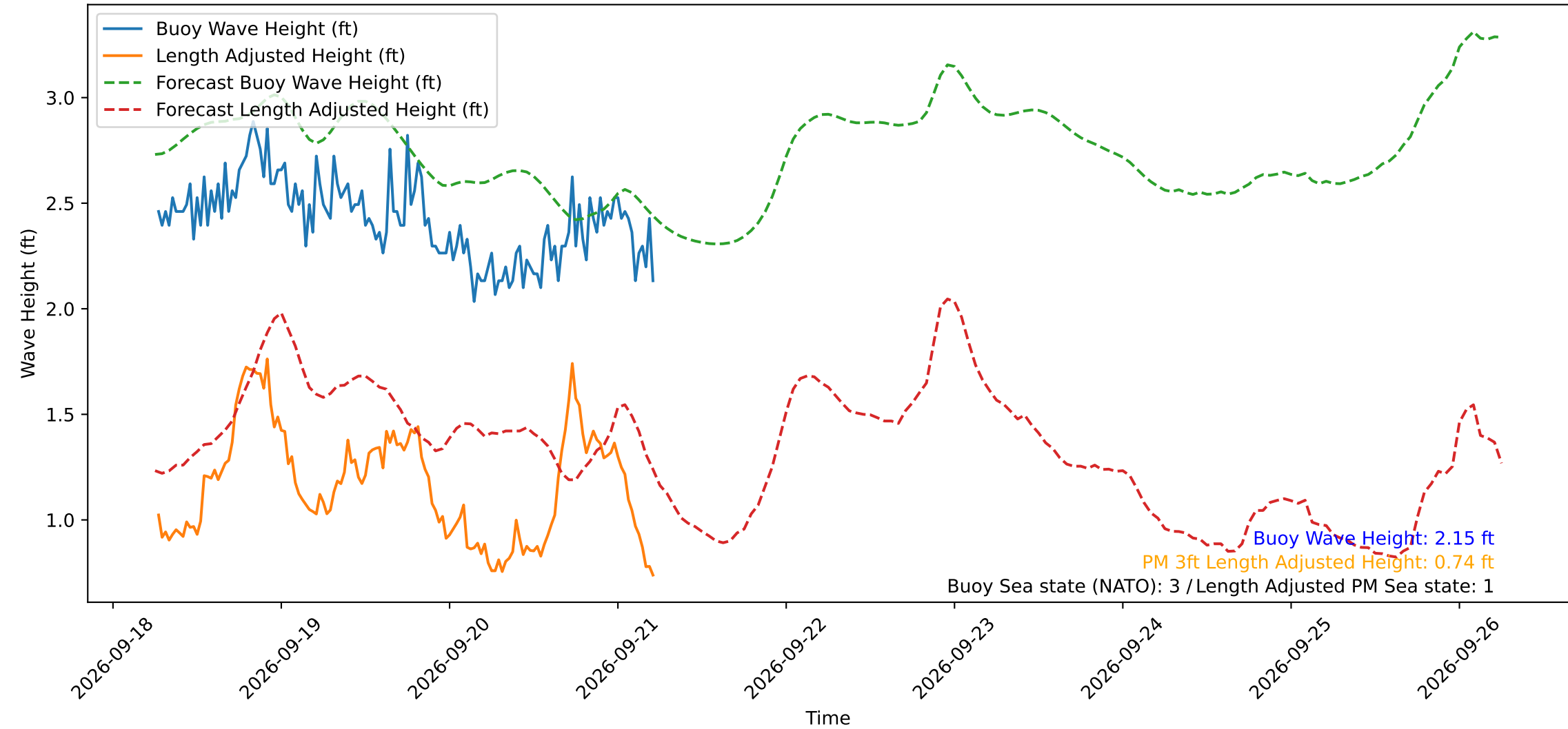
Wave Heights over Time for Red Beach at 2026-09-21 06:00:49
