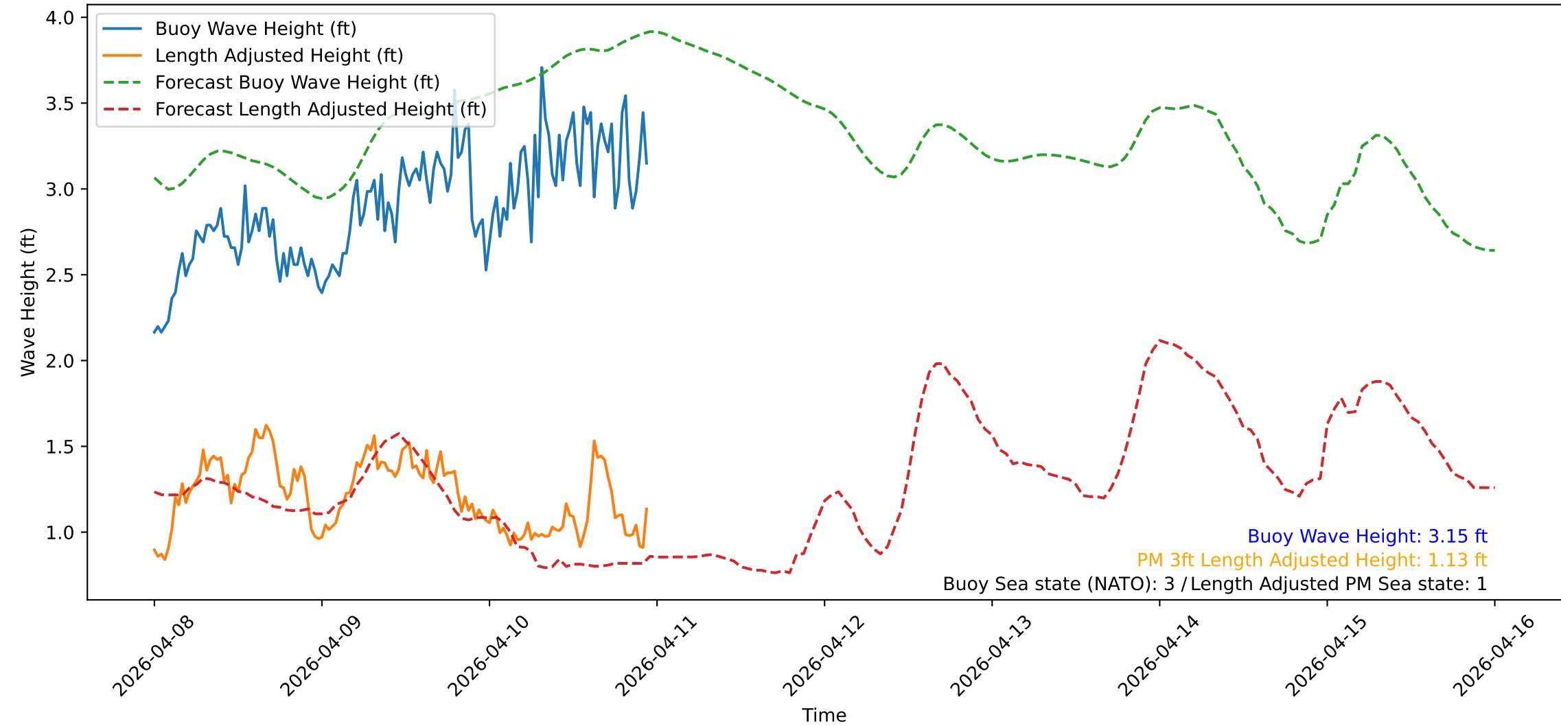
Wave Heights over Time for Red Beach at 2026-04-10 23:30:51
