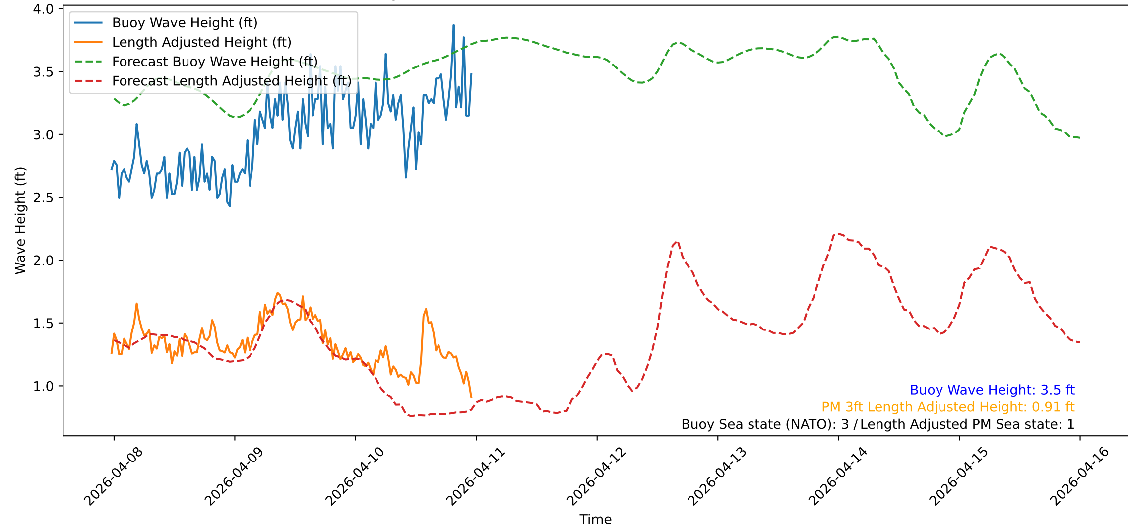
Wave Heights over Time for Oceanside Harbor at 2026-04-10 23:30:31
