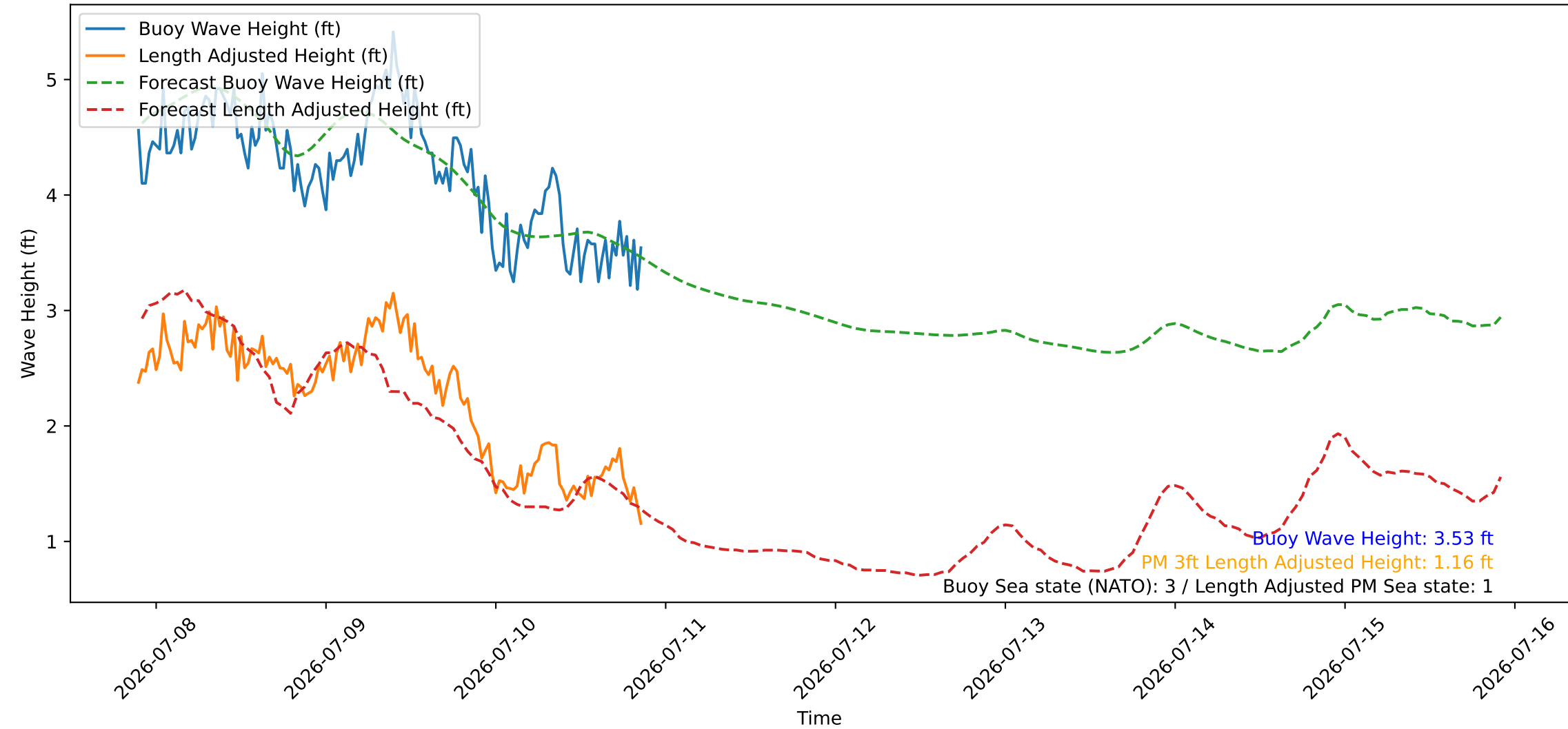
Wave Heights over Time for Oceanside Harbor at 2026-07-10 21:30:26
