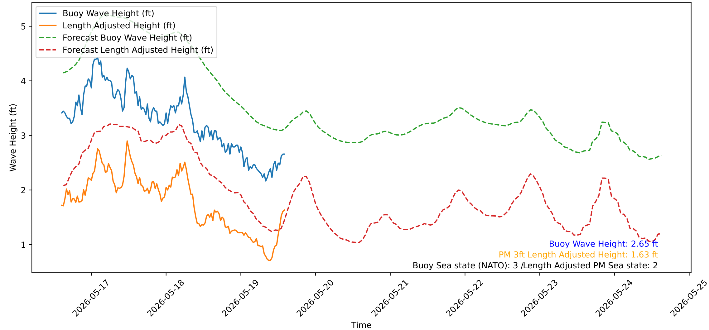
Wave Heights over Time for Green Beach at 2026-05-19 14:41:13
