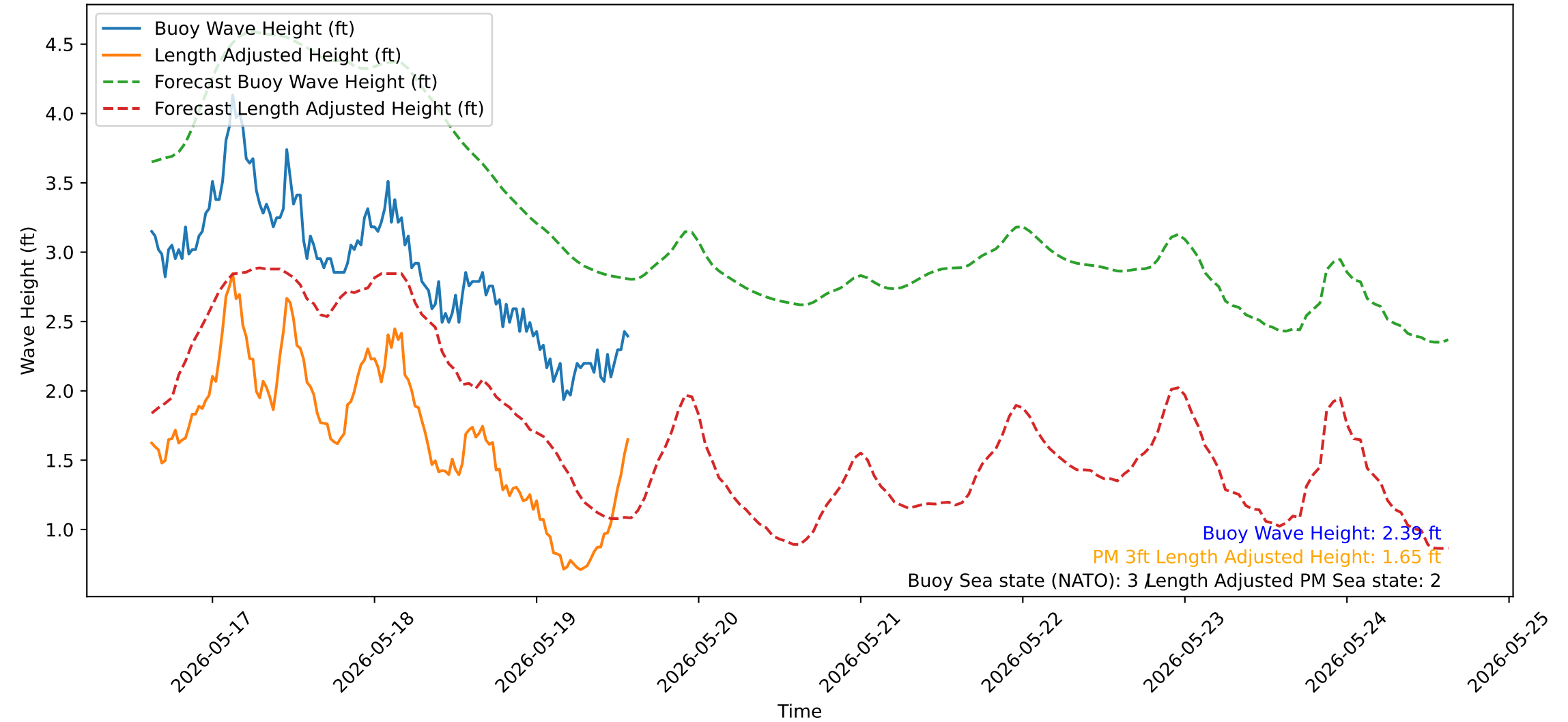
Wave Heights over Time for Red Beach at 2026-05-19 14:40:50
