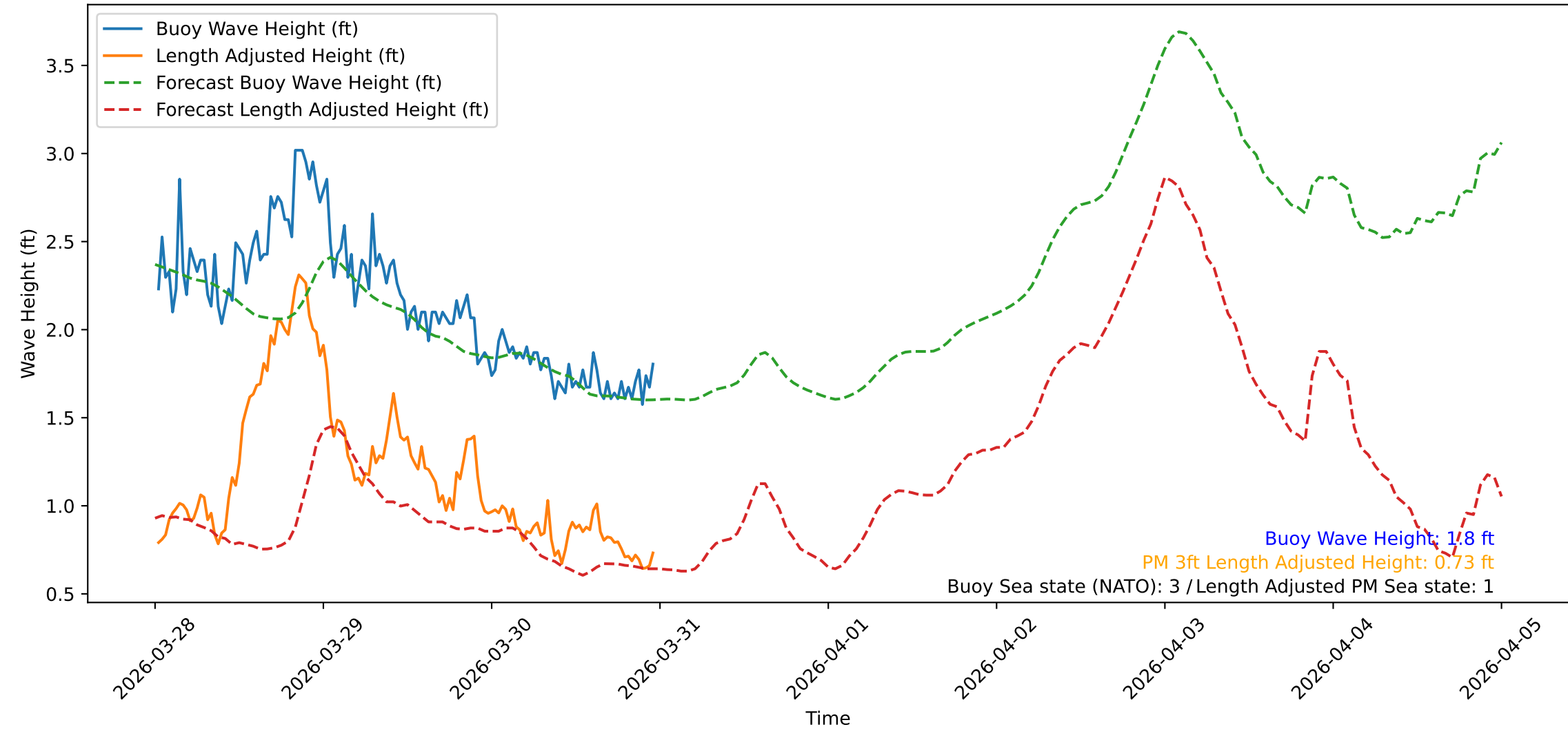
Wave Heights over Time for Red Beach at 2026-03-31 00:00:48
