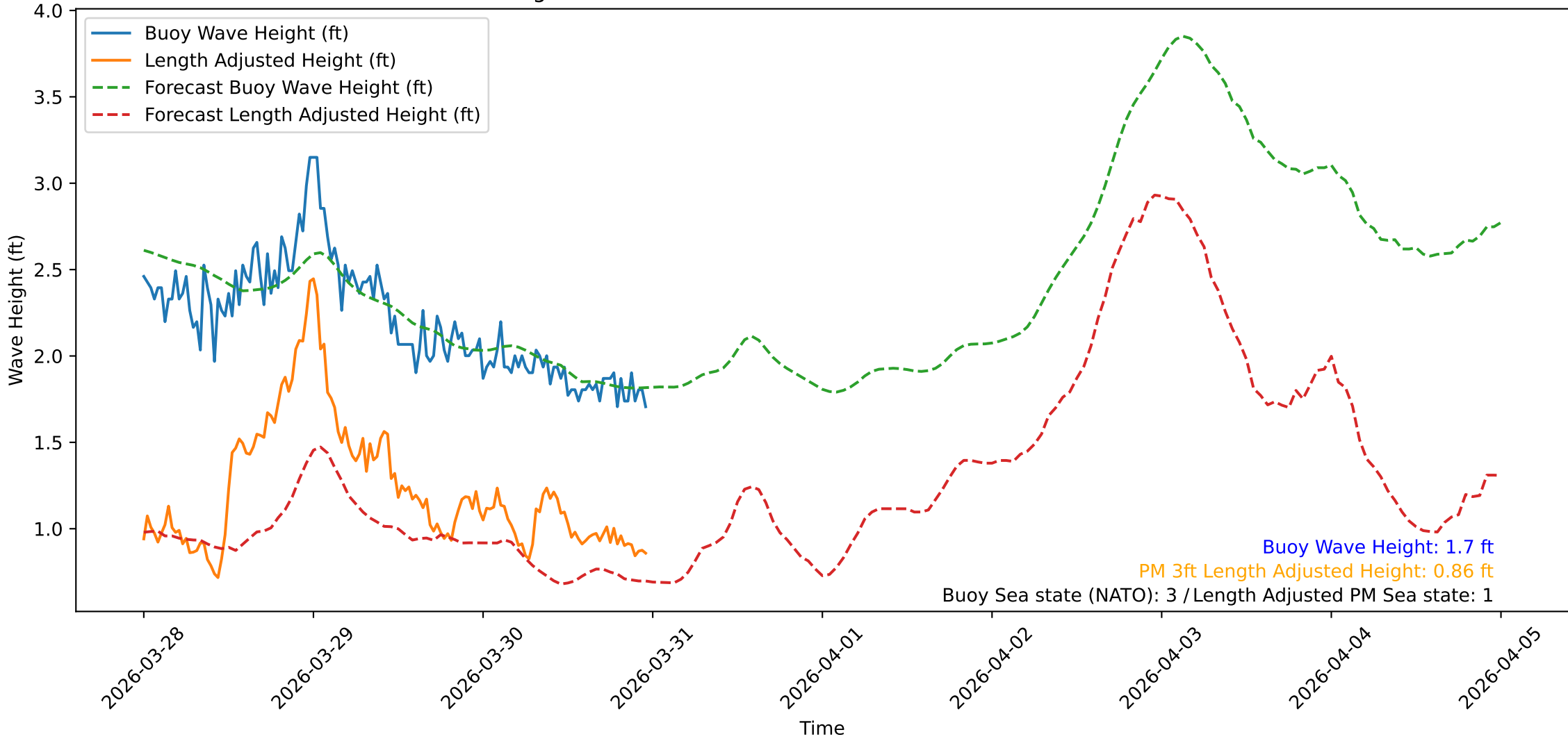
Wave Heights over Time for Oceanside Harbor at 2026-03-31 00:00:32
