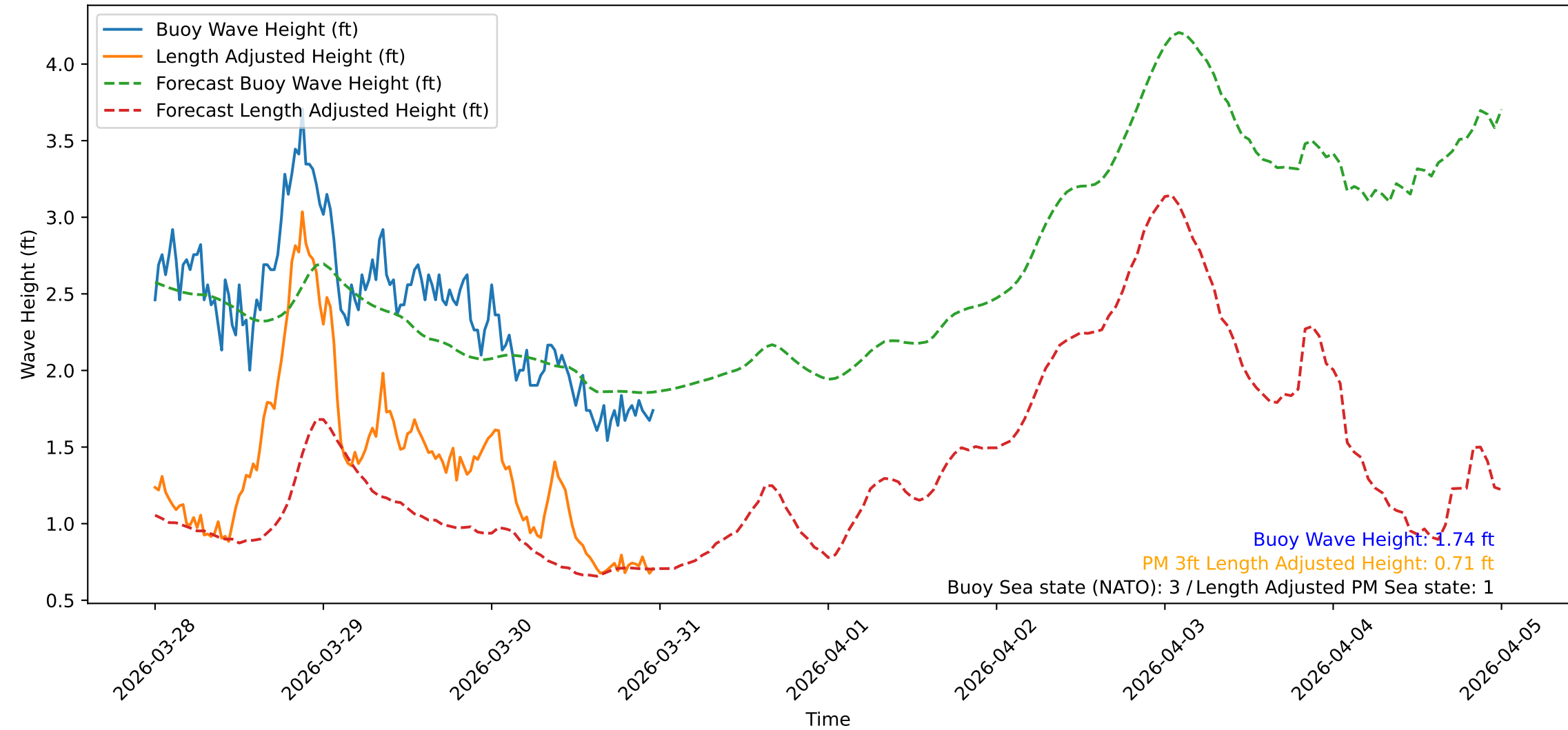
Wave Heights over Time for Green Beach at 2026-03-31 00:01:11
