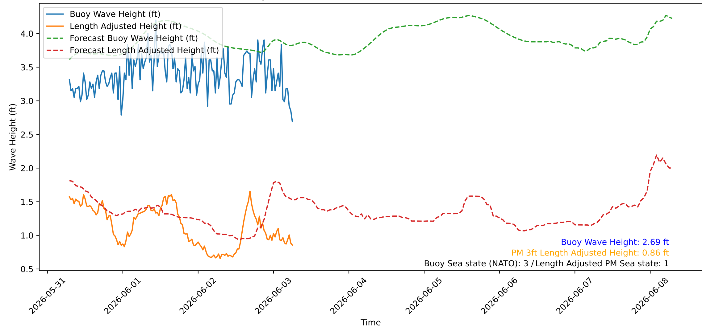
Wave Heights over Time for Red Beach at 2026-06-03 06:50:46
