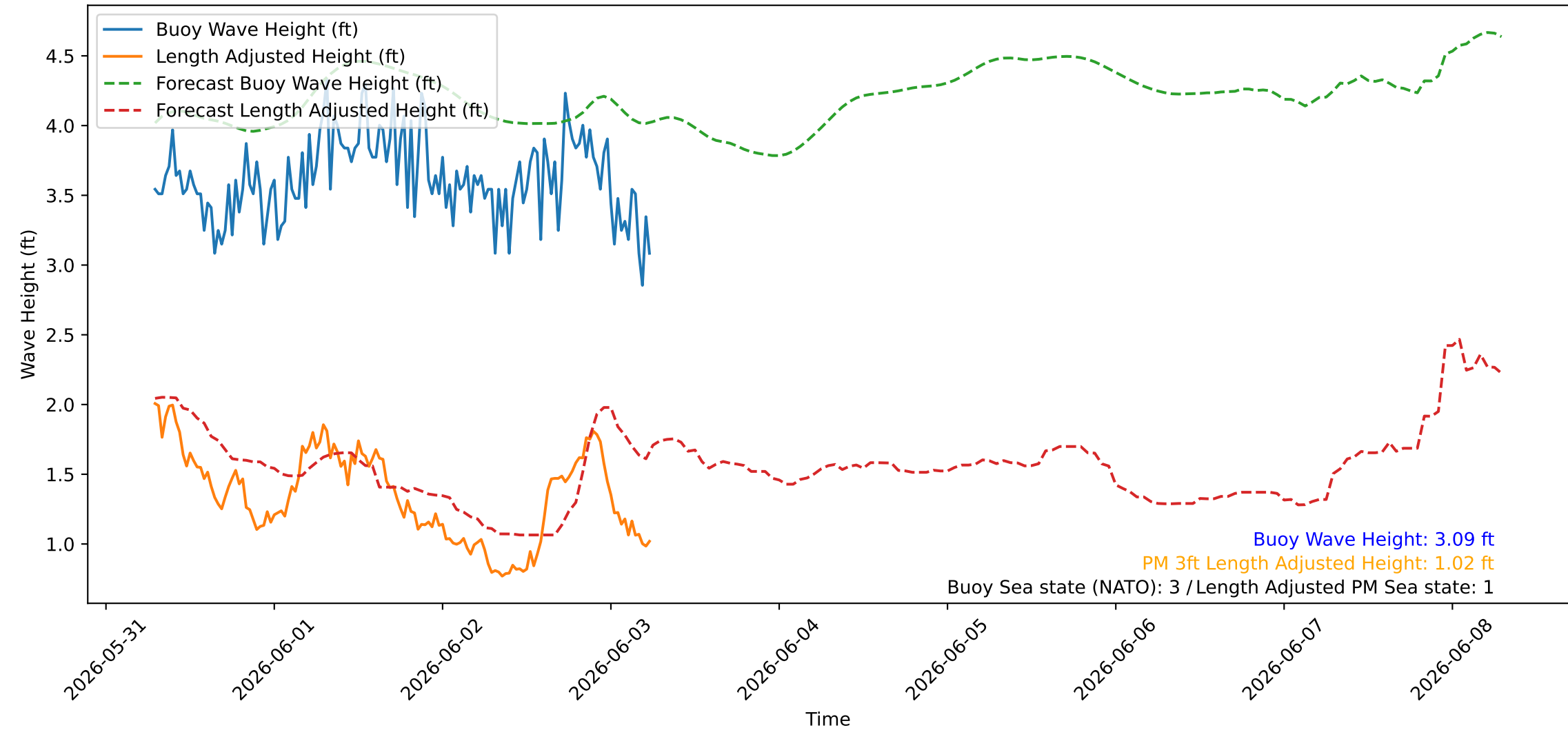
Wave Heights over Time for Green Beach at 2026-06-03 06:51:09
