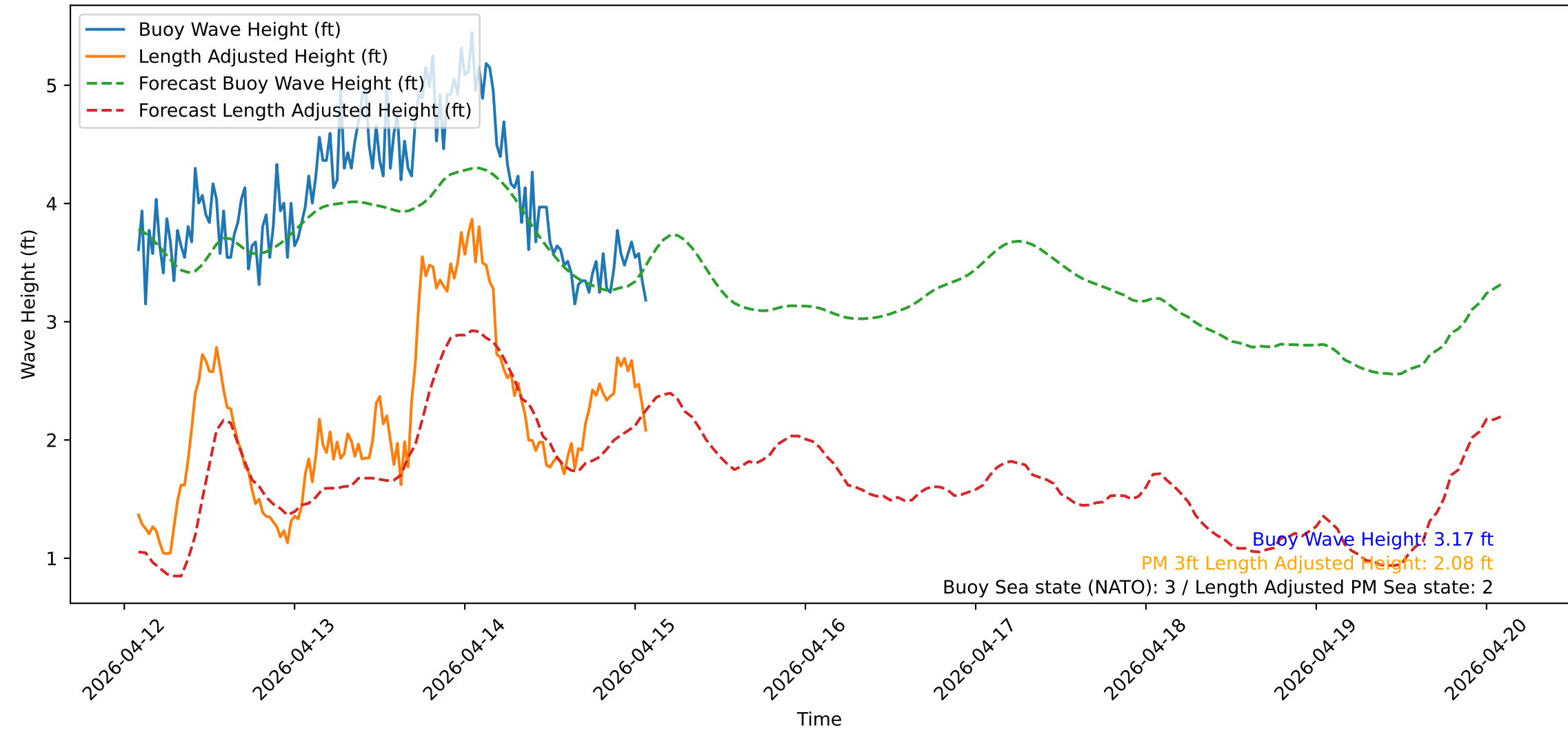
Wave Heights over Time for Oceanside Harbor at 2026-04-15 02:00:31
