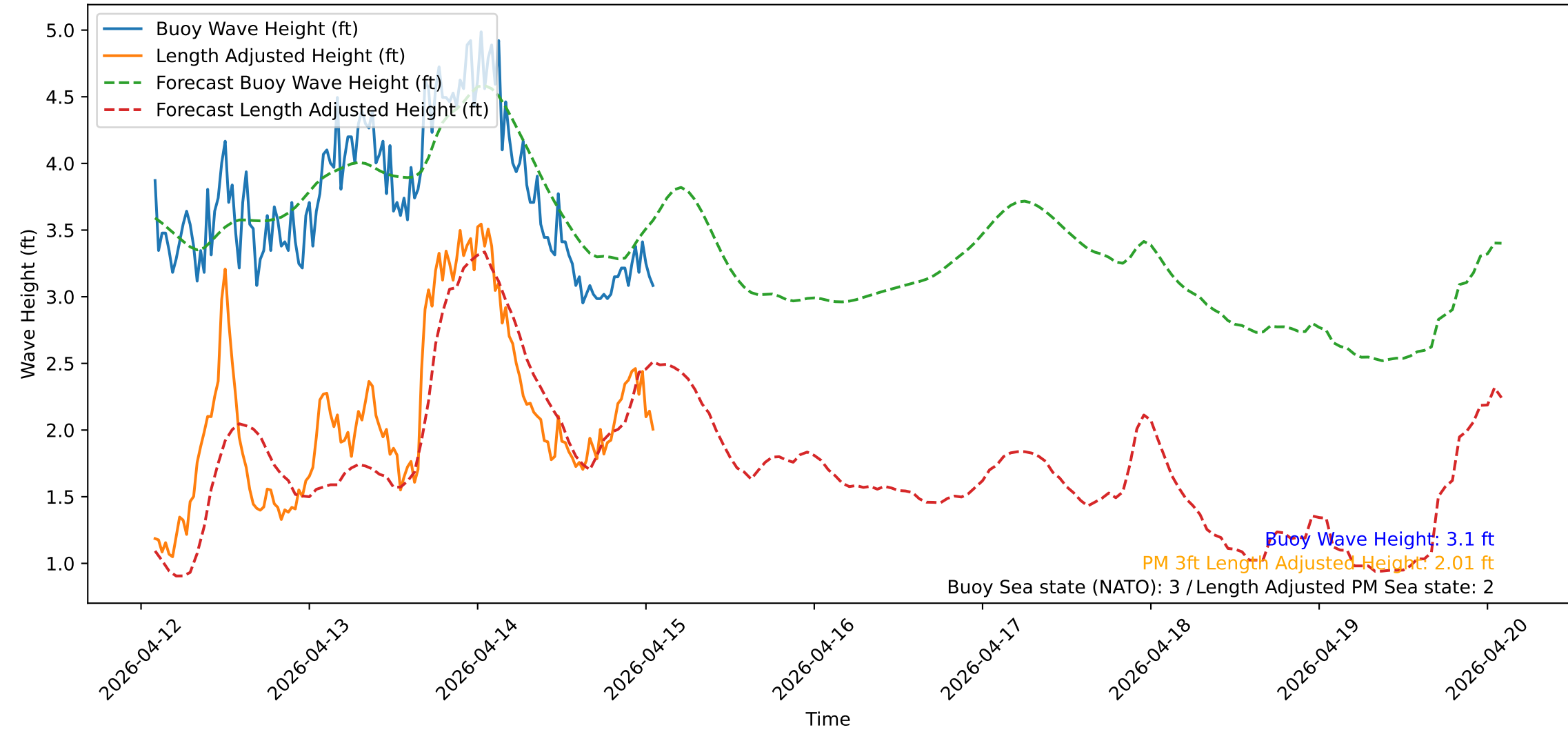
Wave Heights over Time for Green Beach at 2026-04-15 02:01:12
