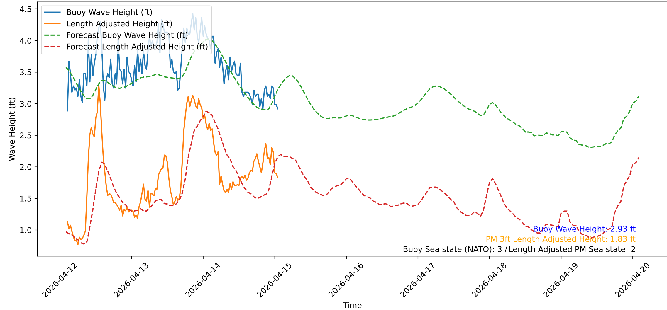
Wave Heights over Time for Red Beach at 2026-04-15 02:00:50
