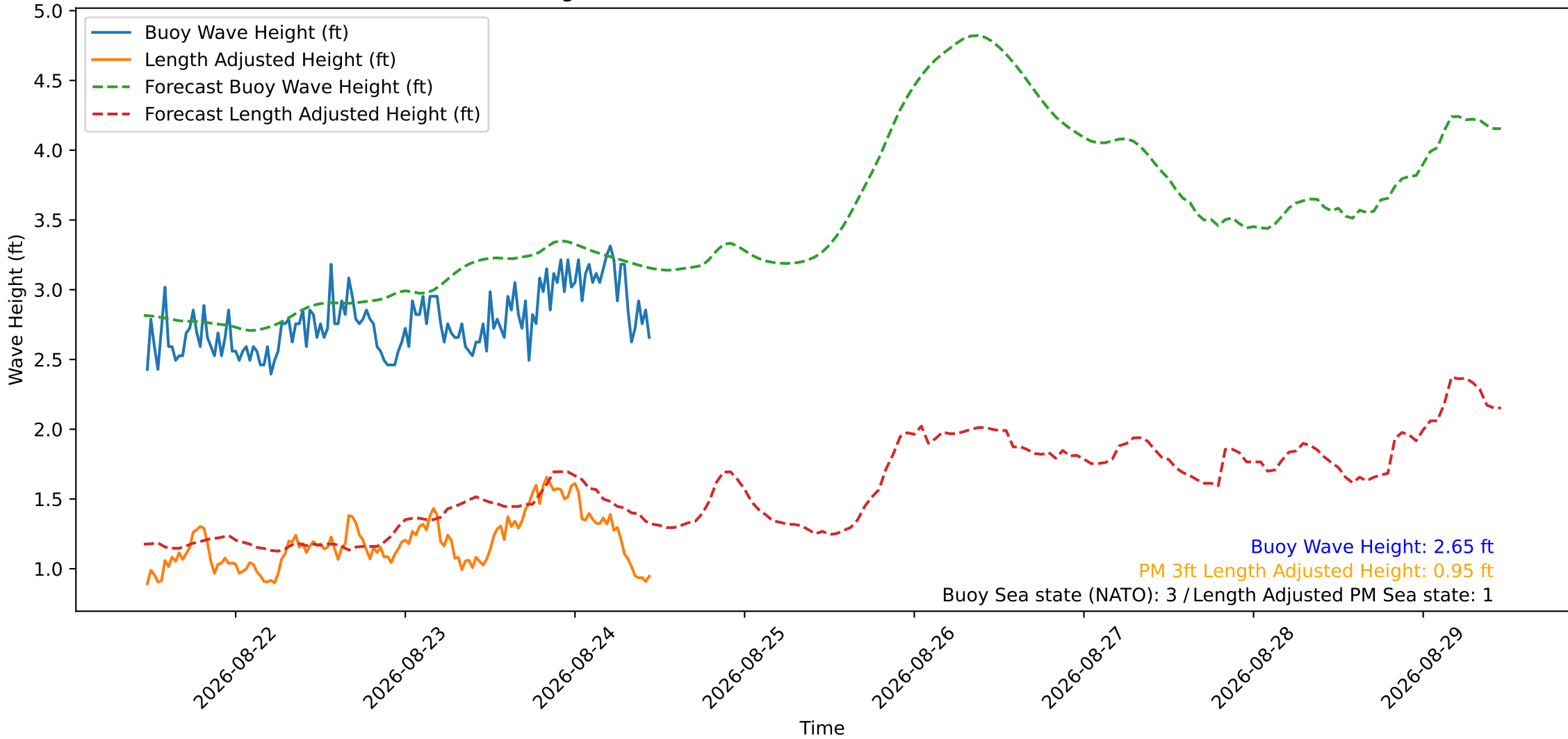
Wave Heights over Time for Green Beach at 2026-08-24 11:21:14
