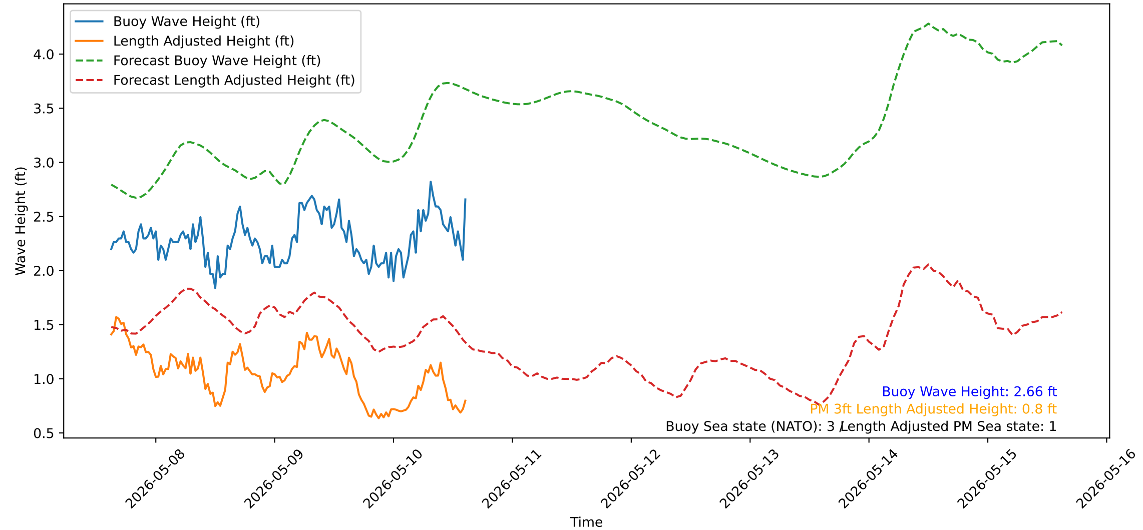
Wave Heights over Time for Green Beach at 2026-05-10 15:11:12
