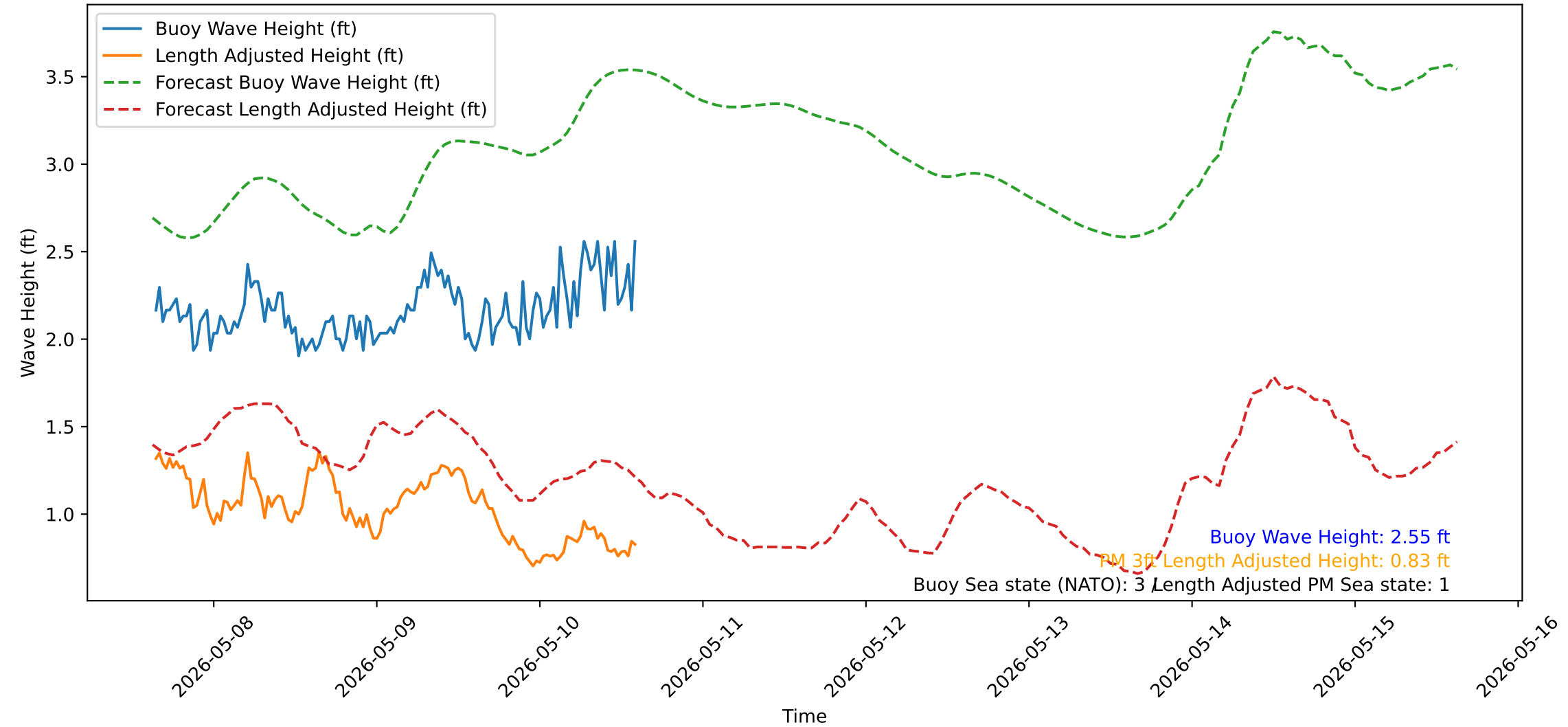
Wave Heights over Time for Red Beach at 2026-05-10 15:10:50
