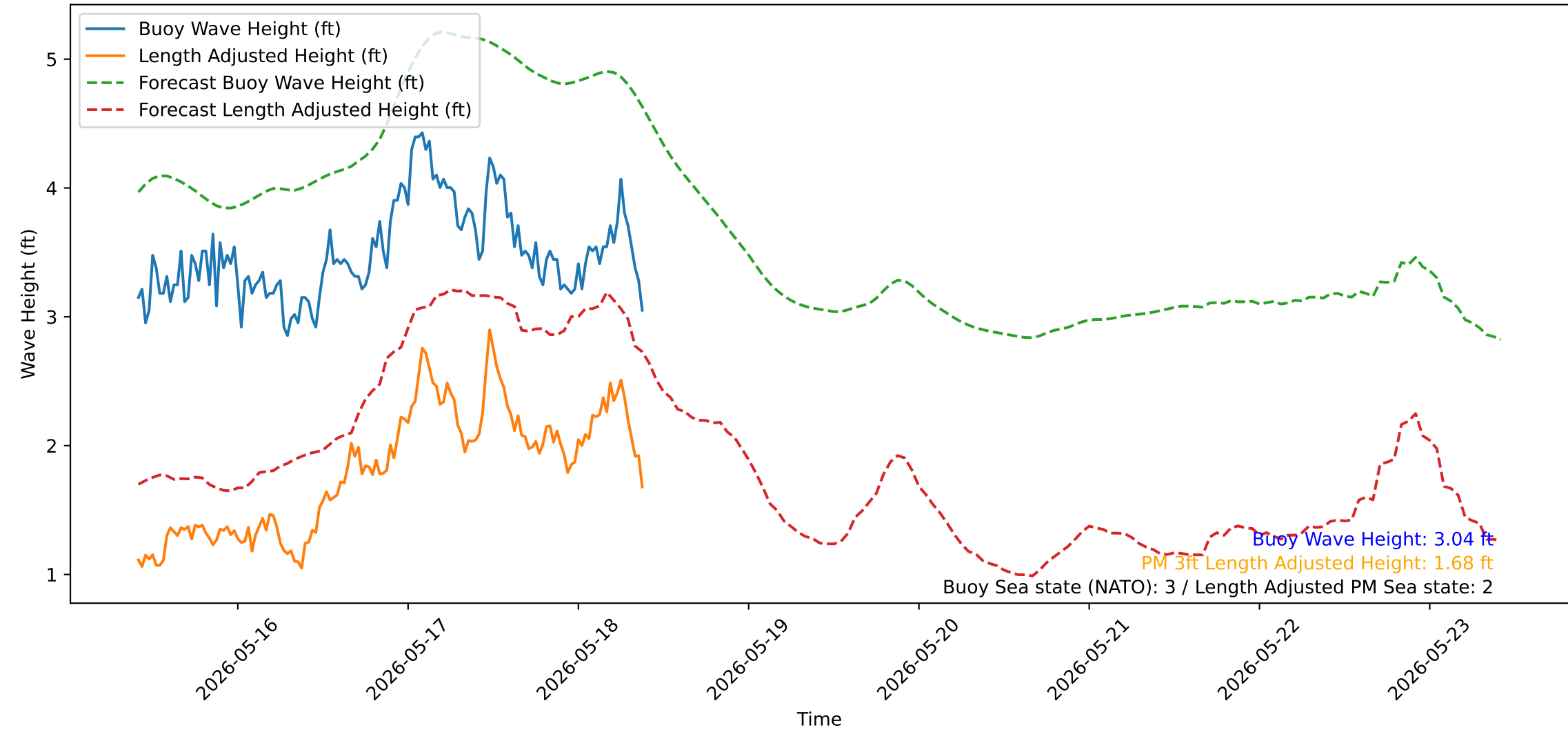
Wave Heights over Time for Green Beach at 2026-05-18 09:51:14
