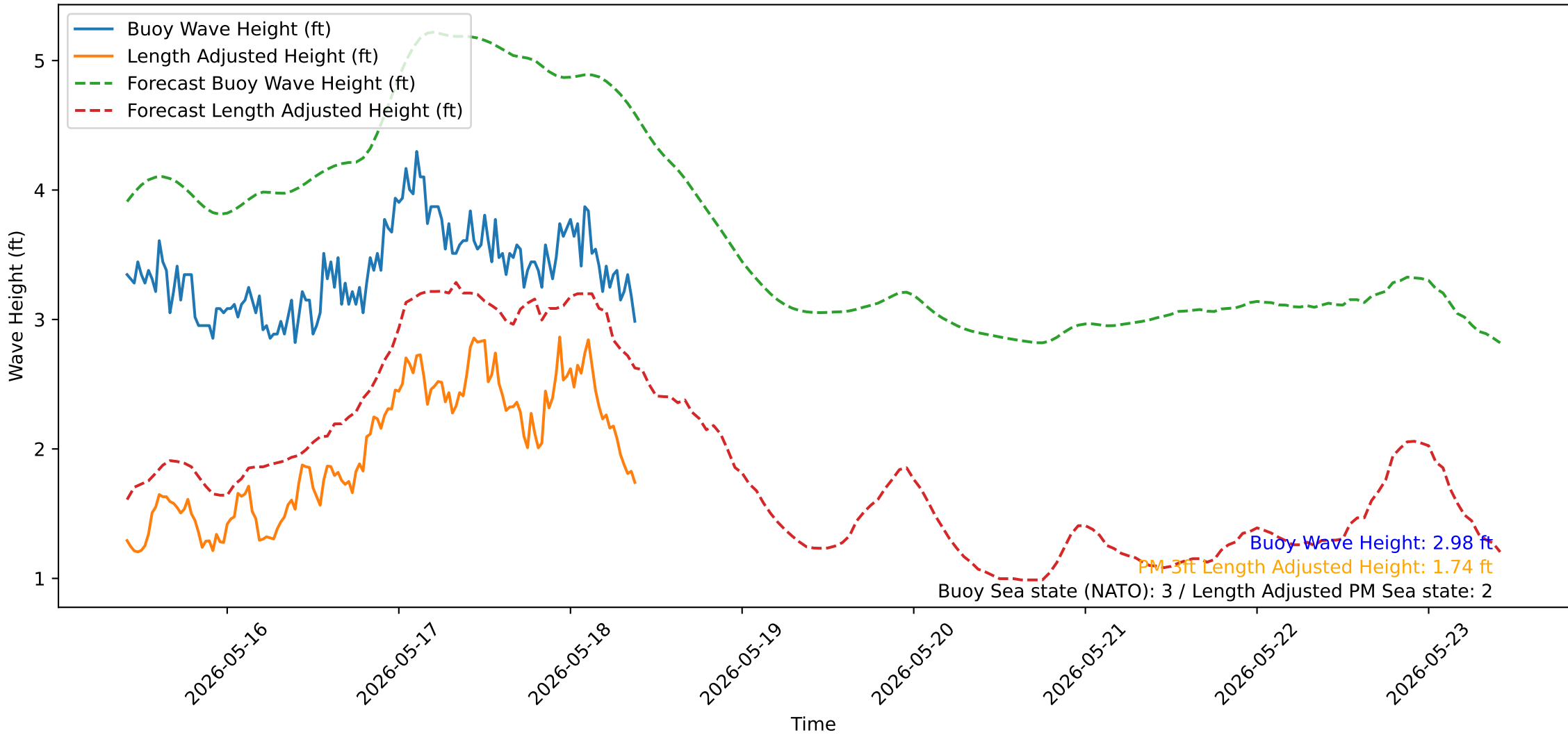
Wave Heights over Time for Oceanside Harbor at 2026-05-18 09:50:32
