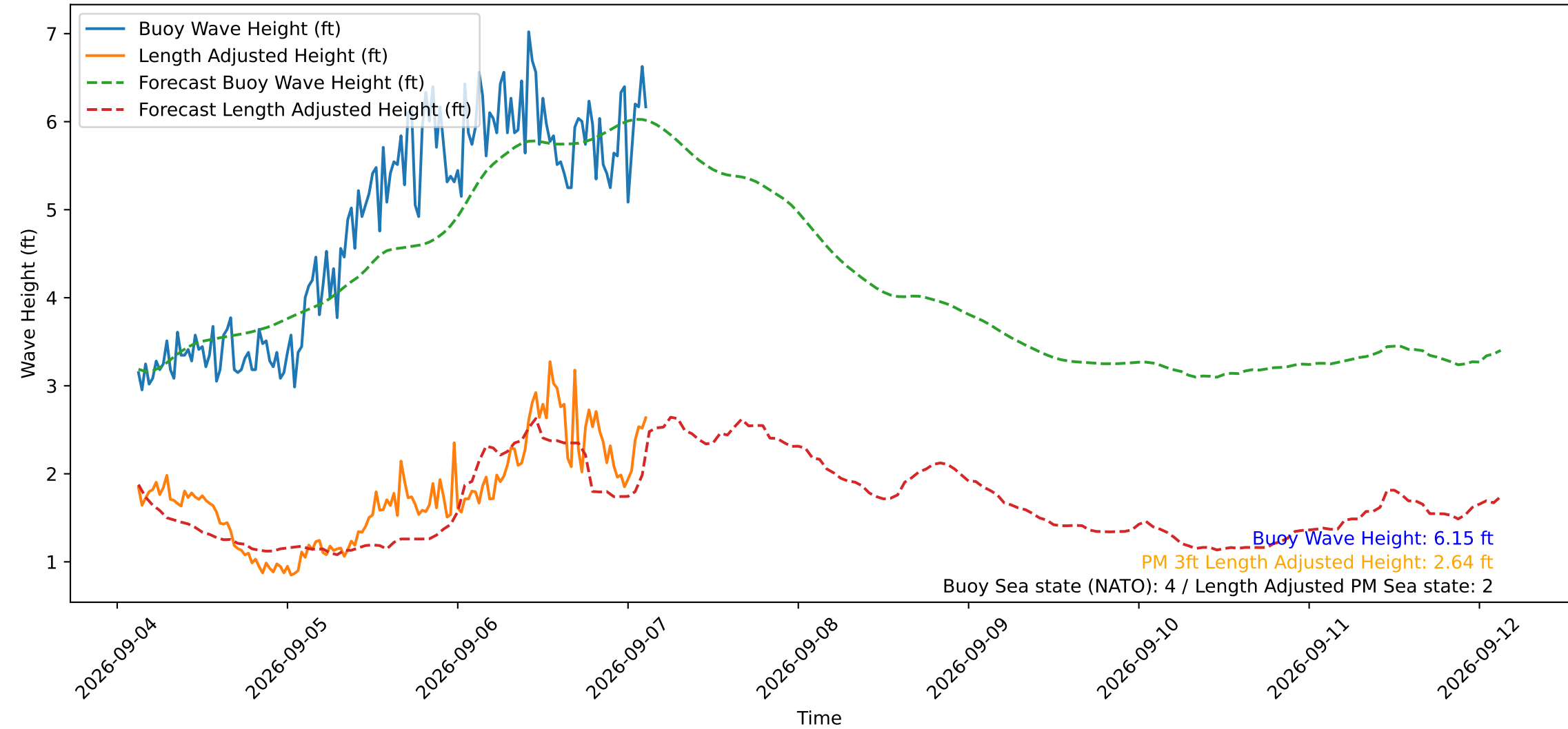
Wave Heights over Time for Oceanside Harbor at 2026-09-07 03:10:30
